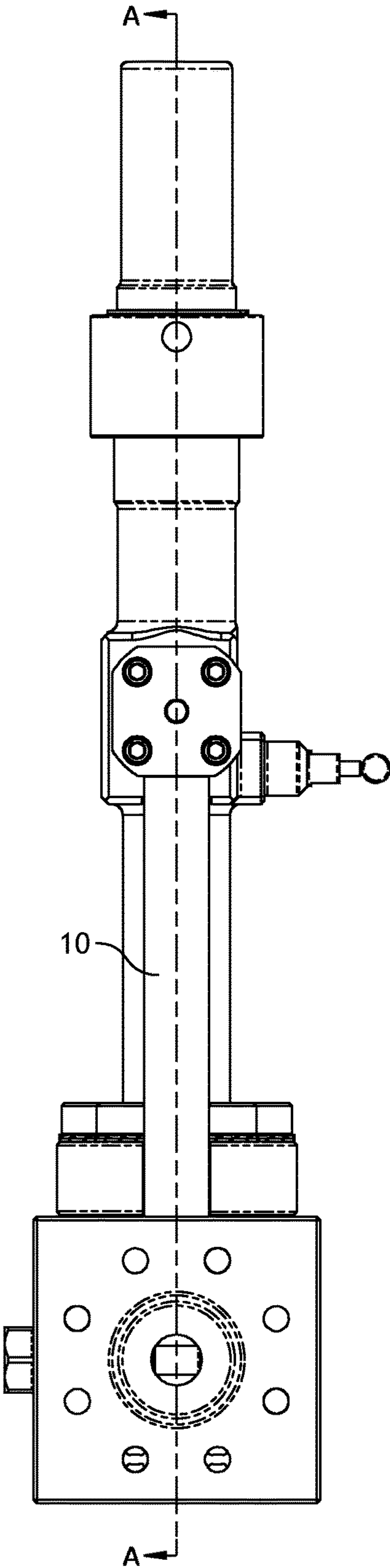
FIG. 2 PRIOR ART
