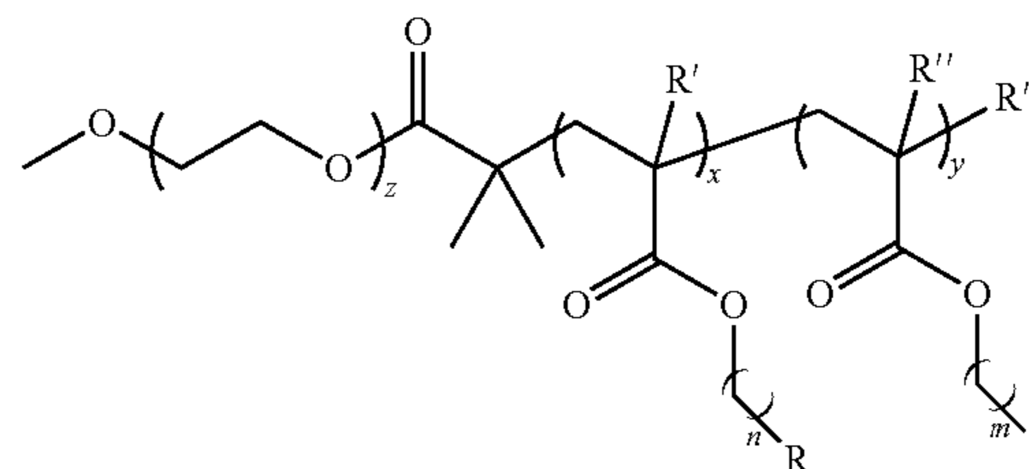
(Formula I)
