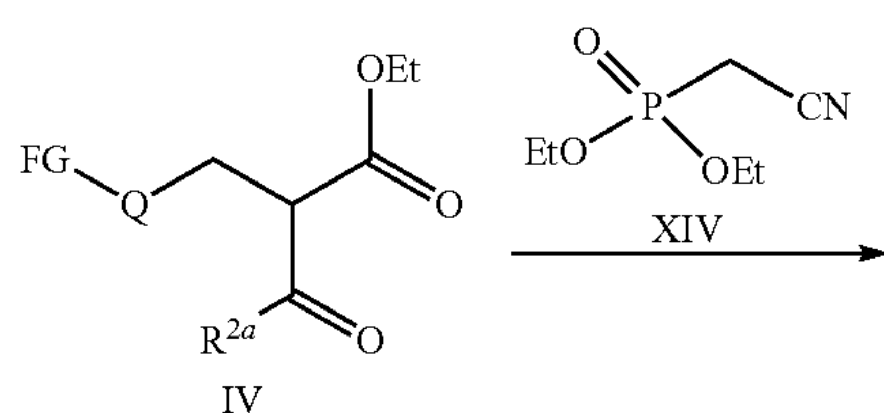
Scheme 5.
