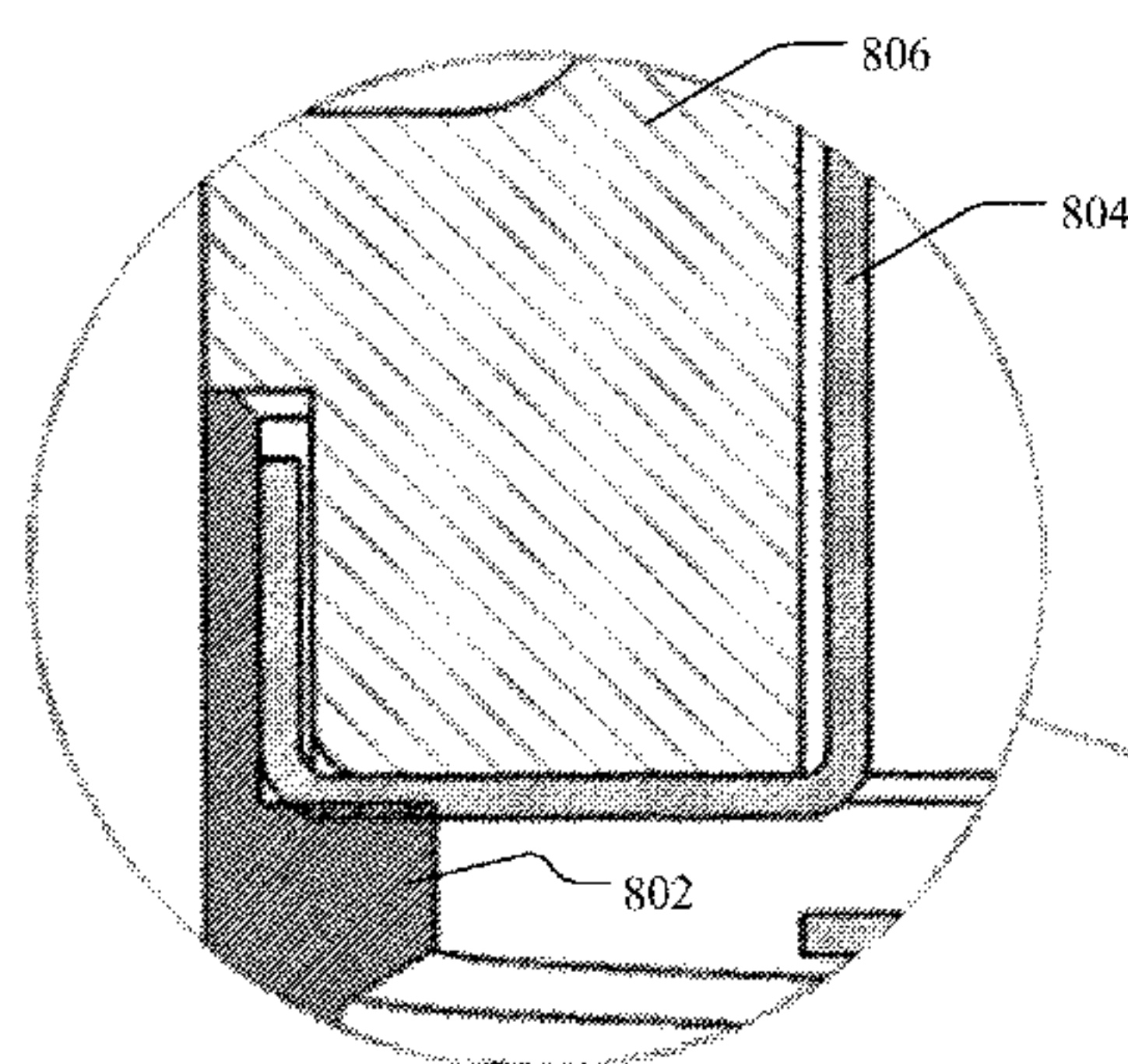
DETAIL C SCALE 5 : 1
