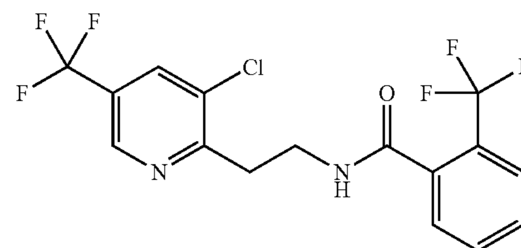
fluopyram
