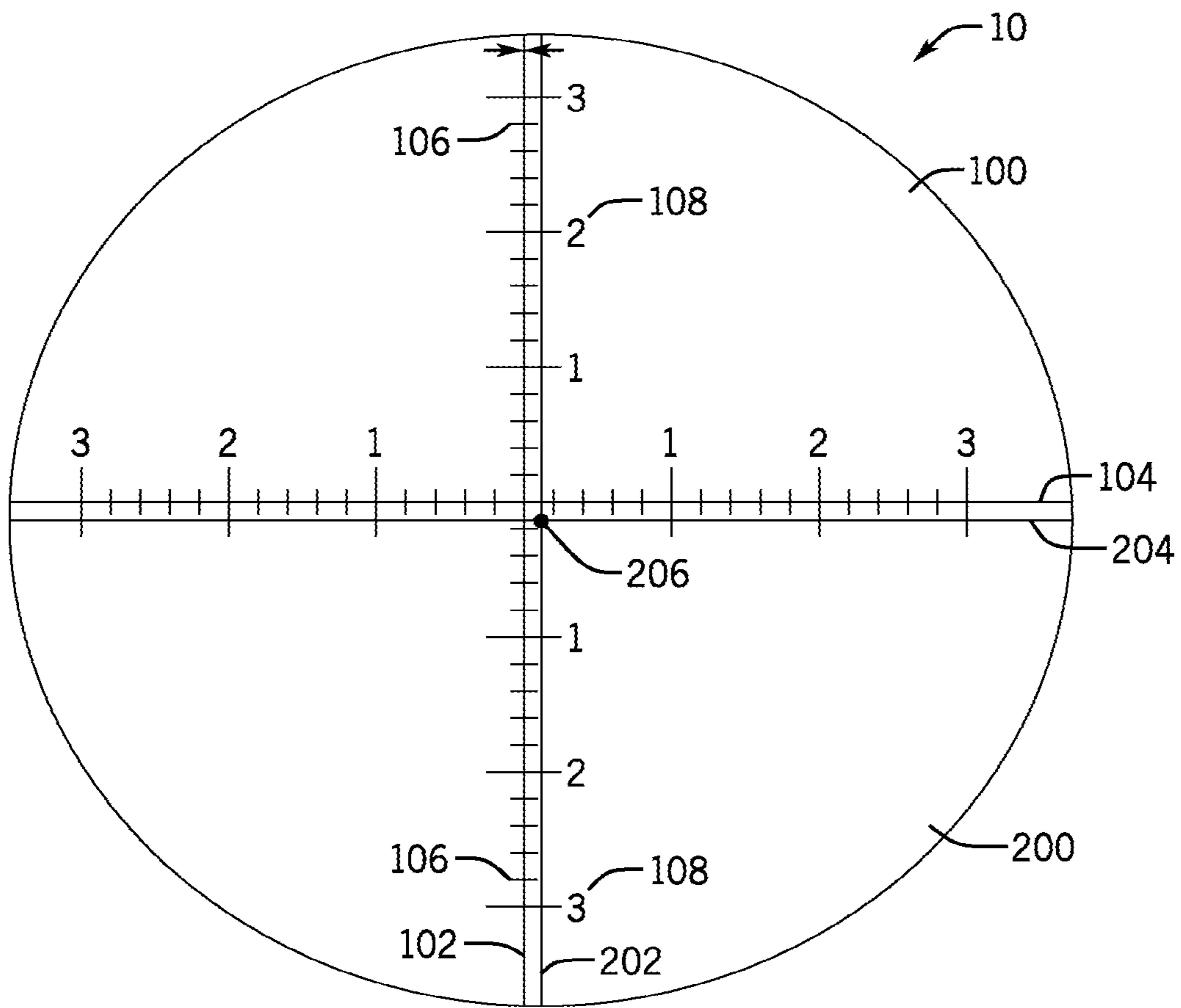
FIG. 10 PRIOR ART
