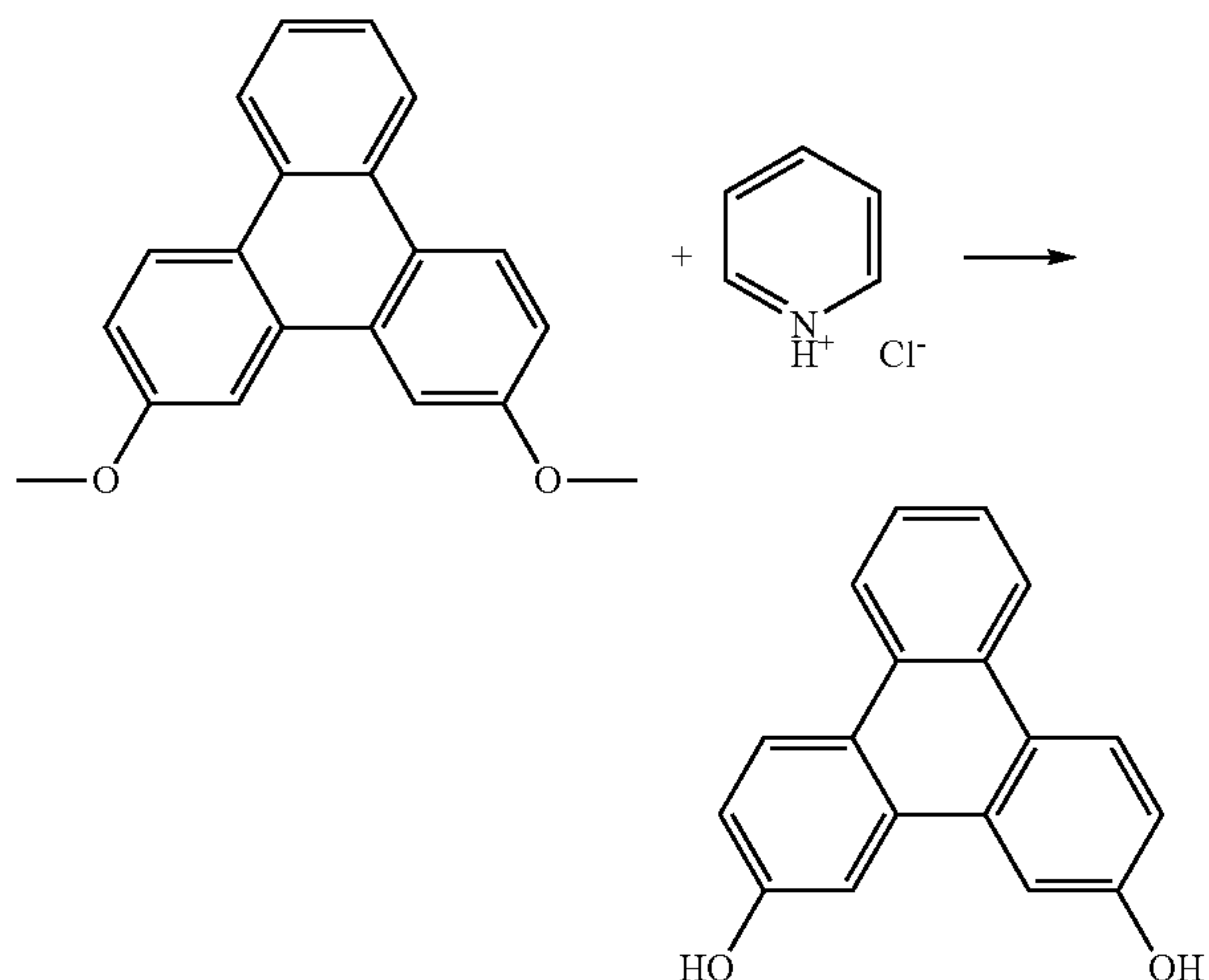
Triphenylene-2,11-diol
