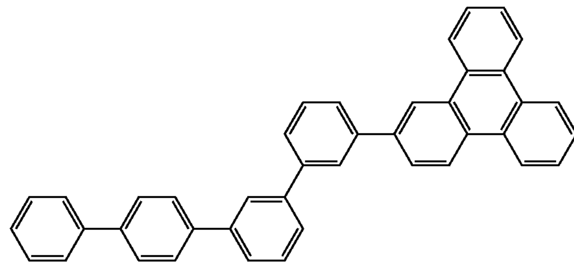
Compound 11
