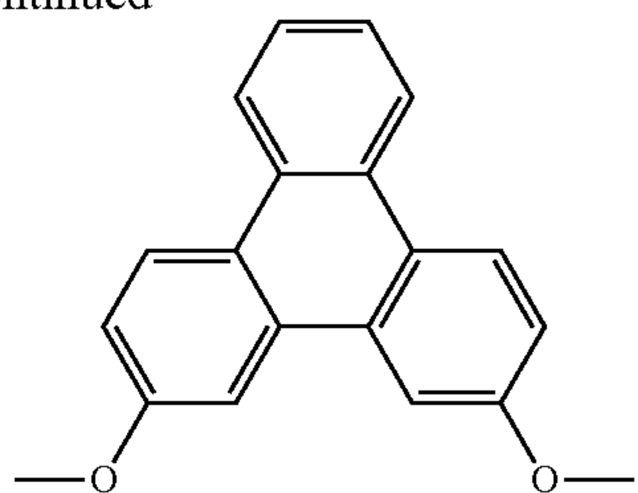
2,11-Dimethoxytriphenylene
