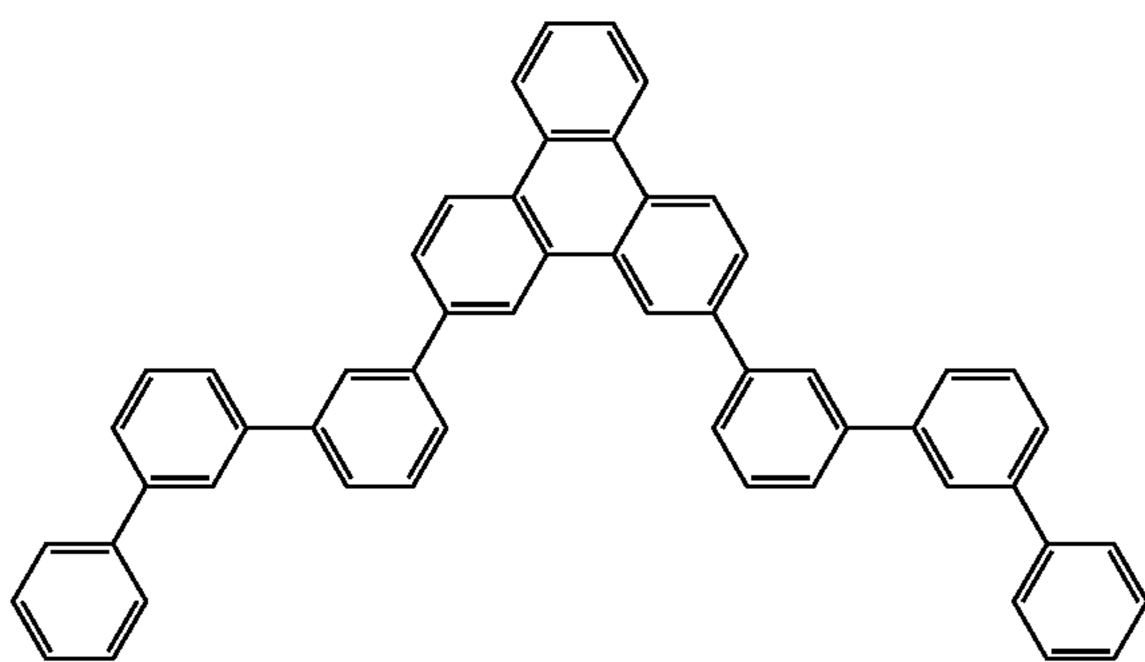
Compound 8
