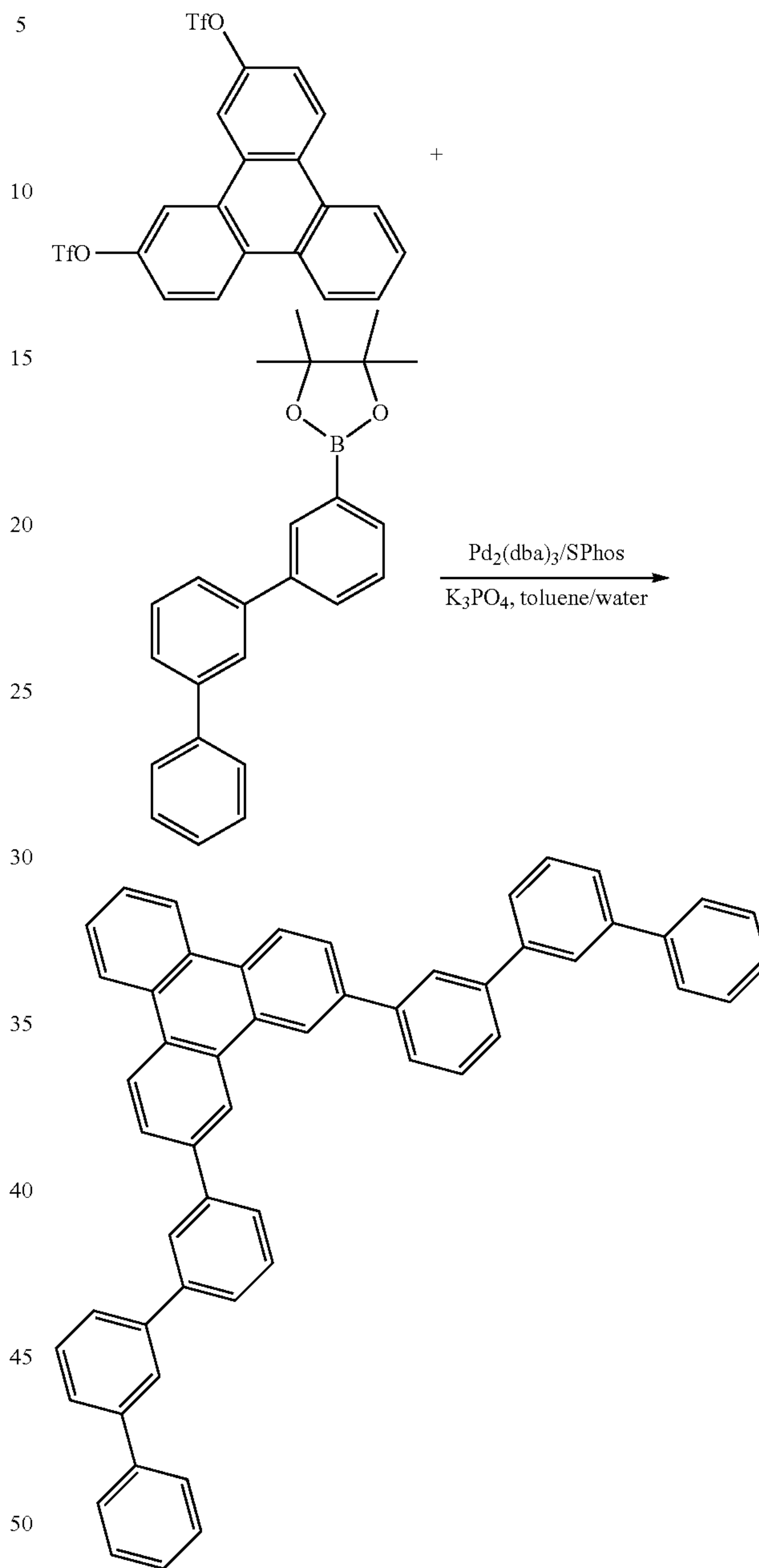
Compound 8
