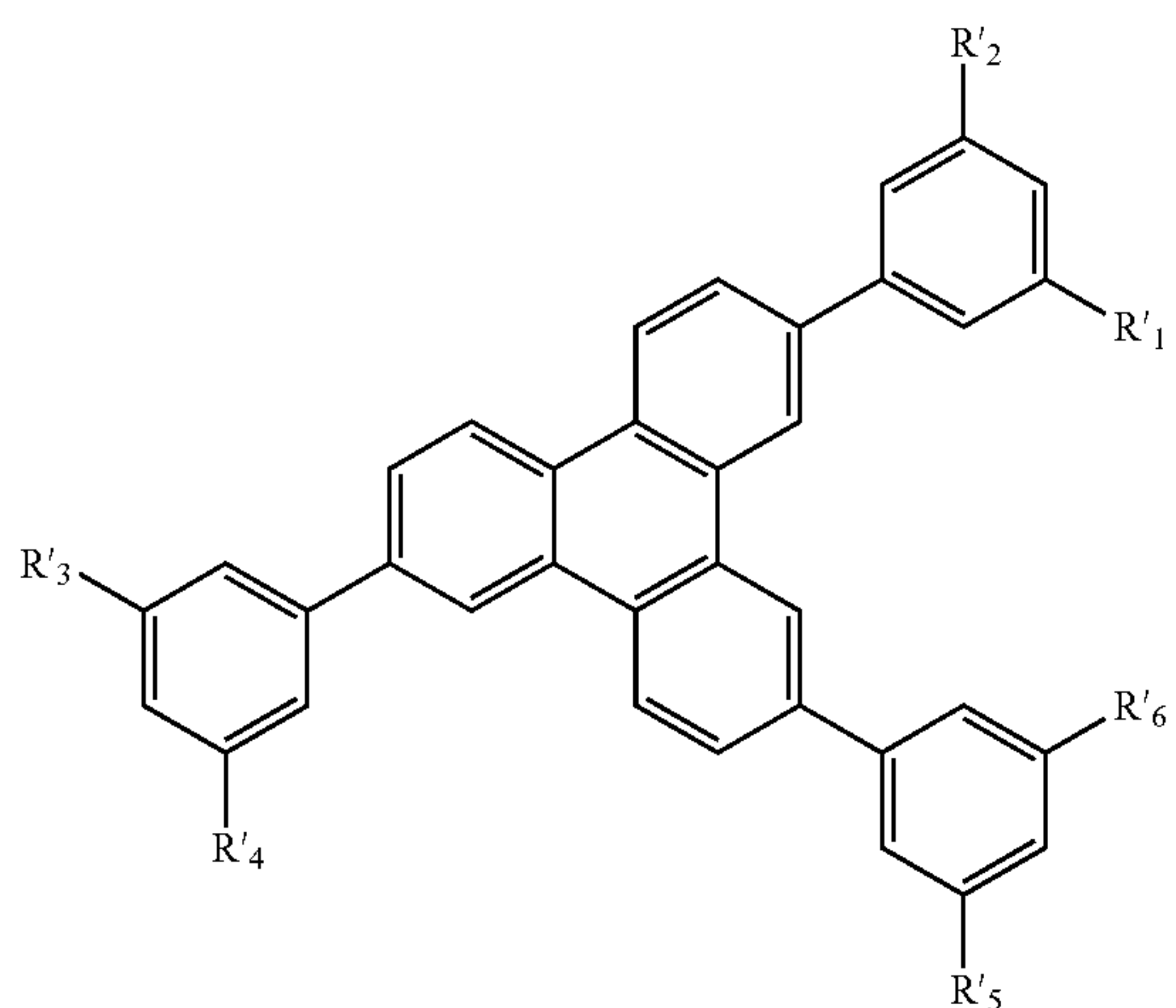
Substructure M
