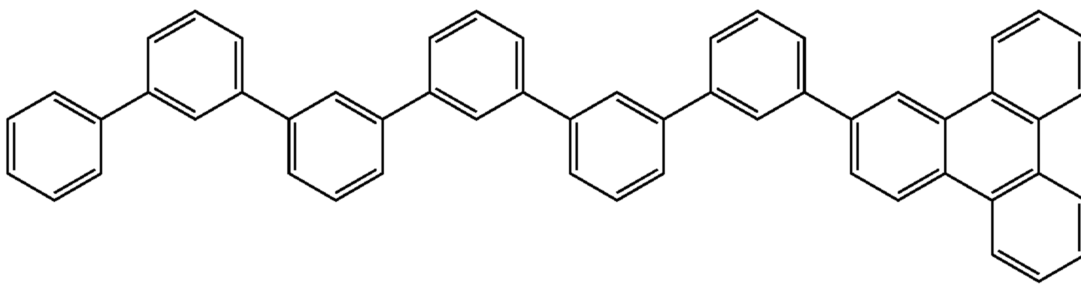
Compound 6
