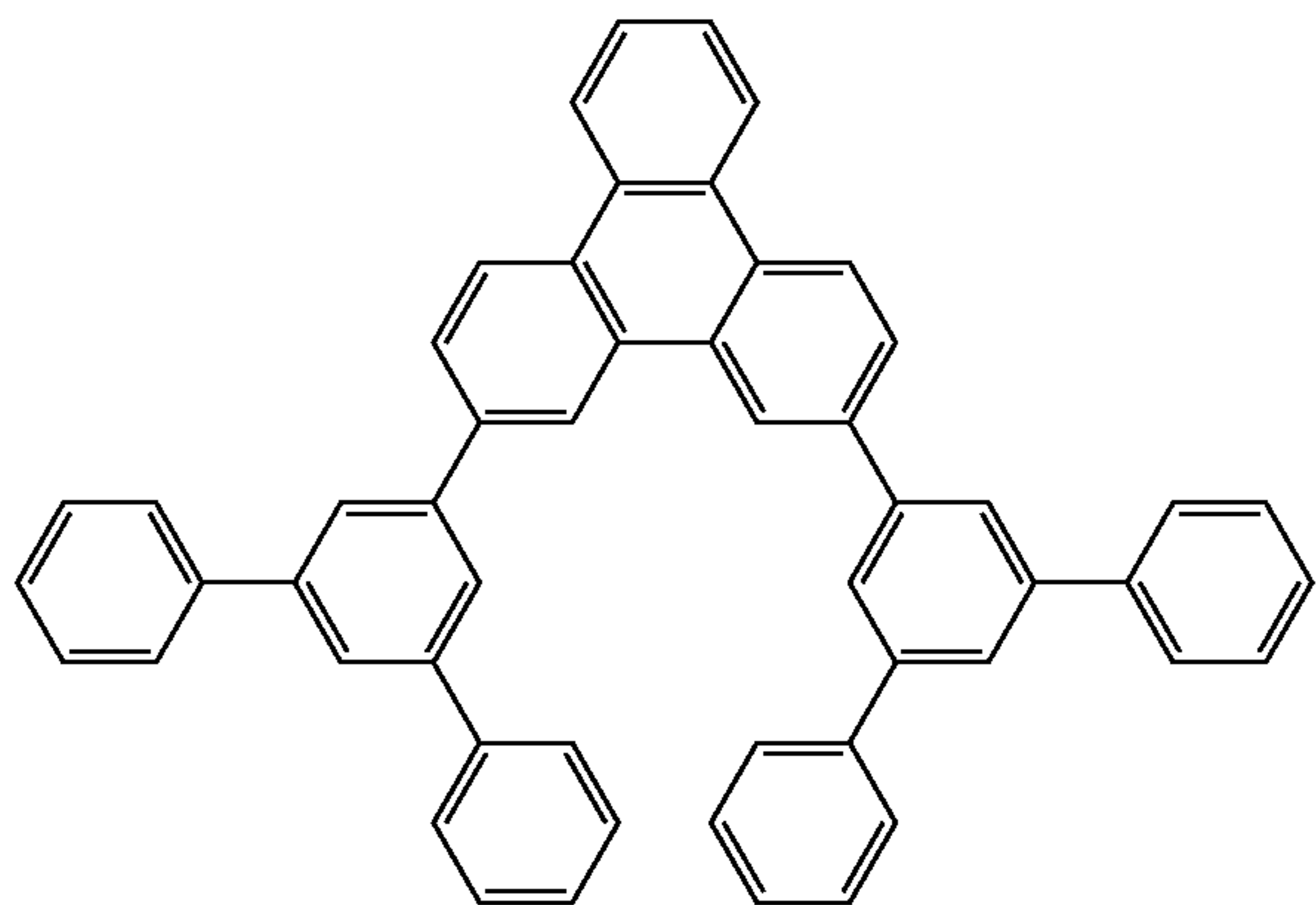
Compound 7
