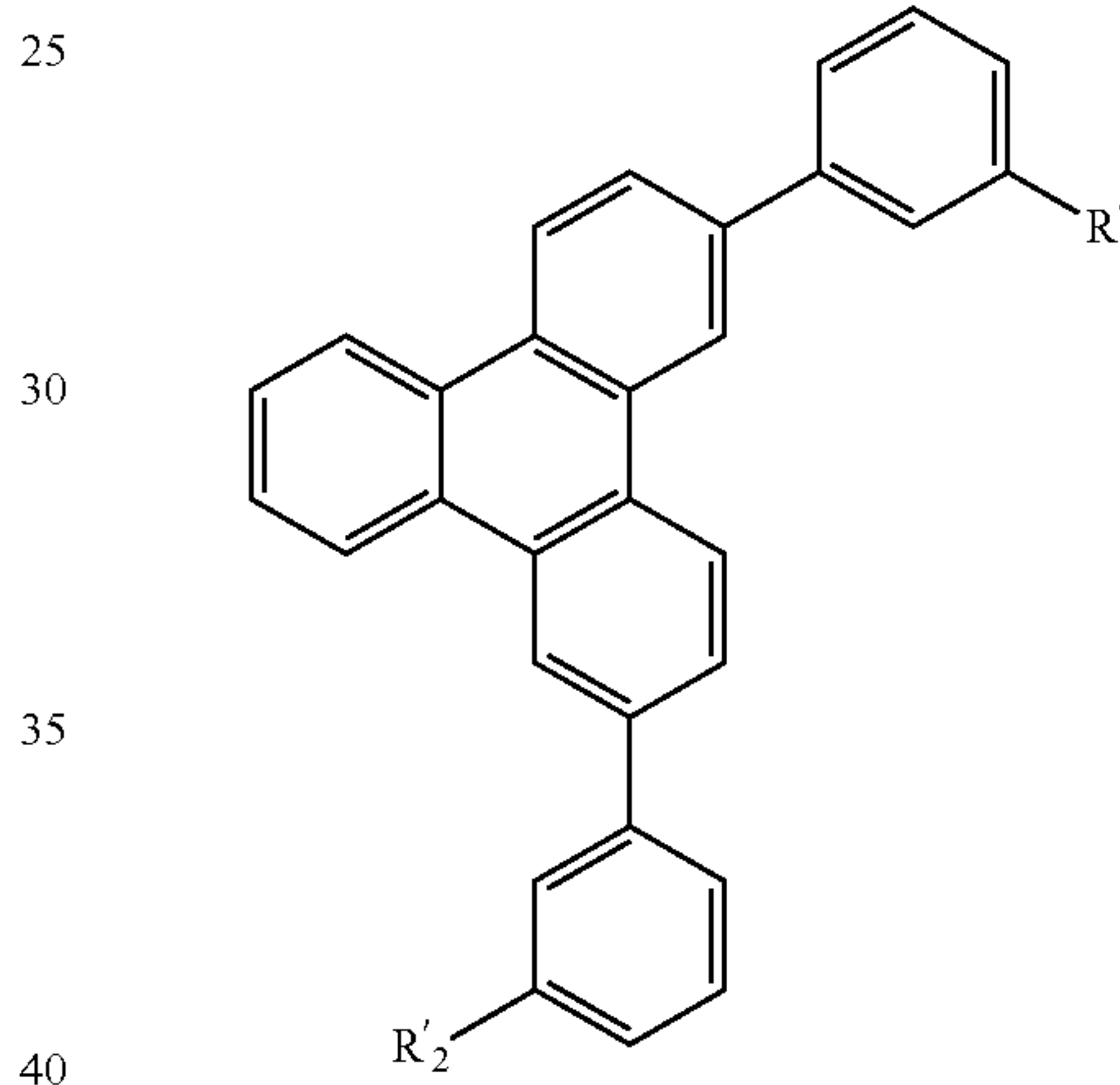
Substructure M
