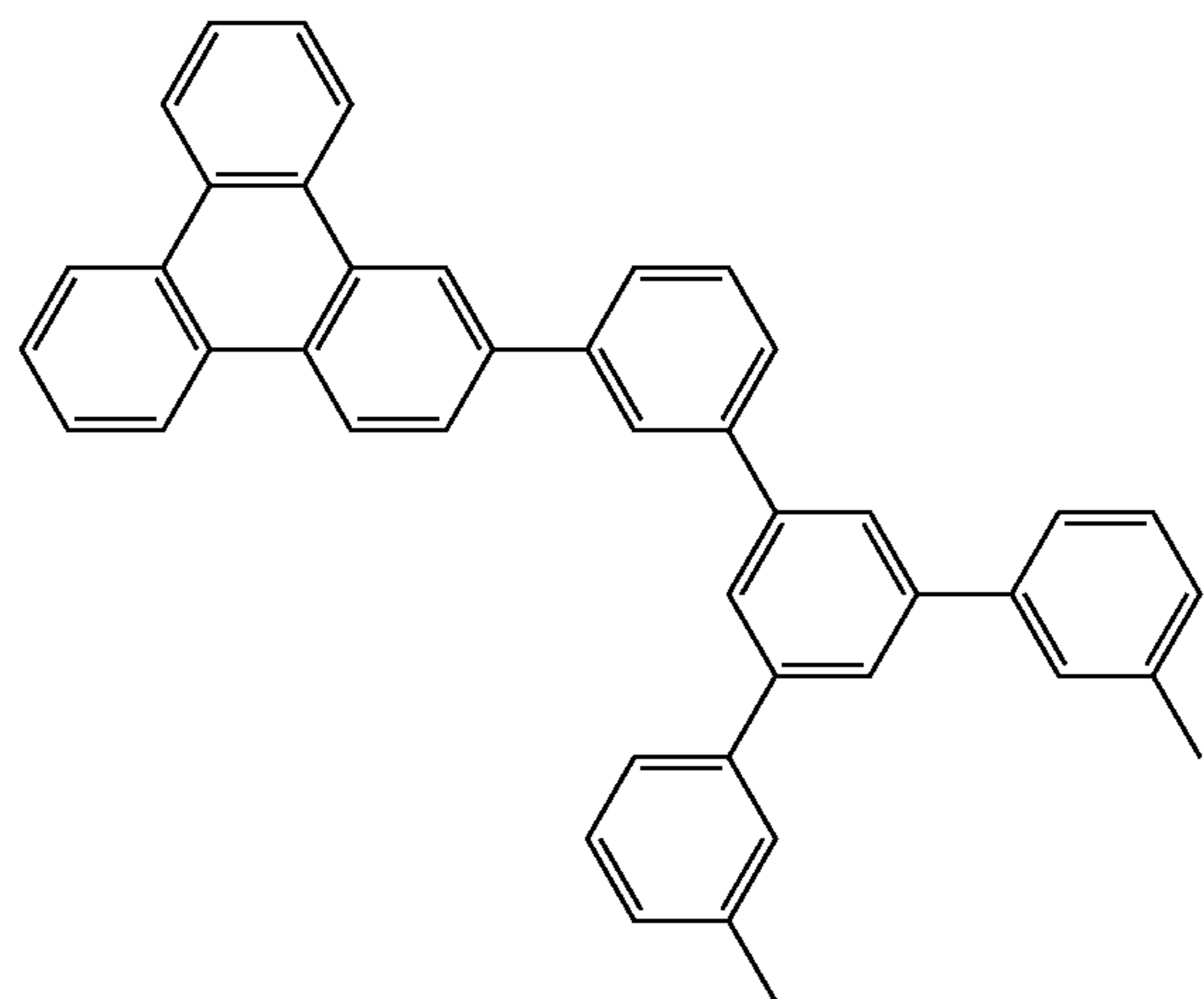
Compound 10
