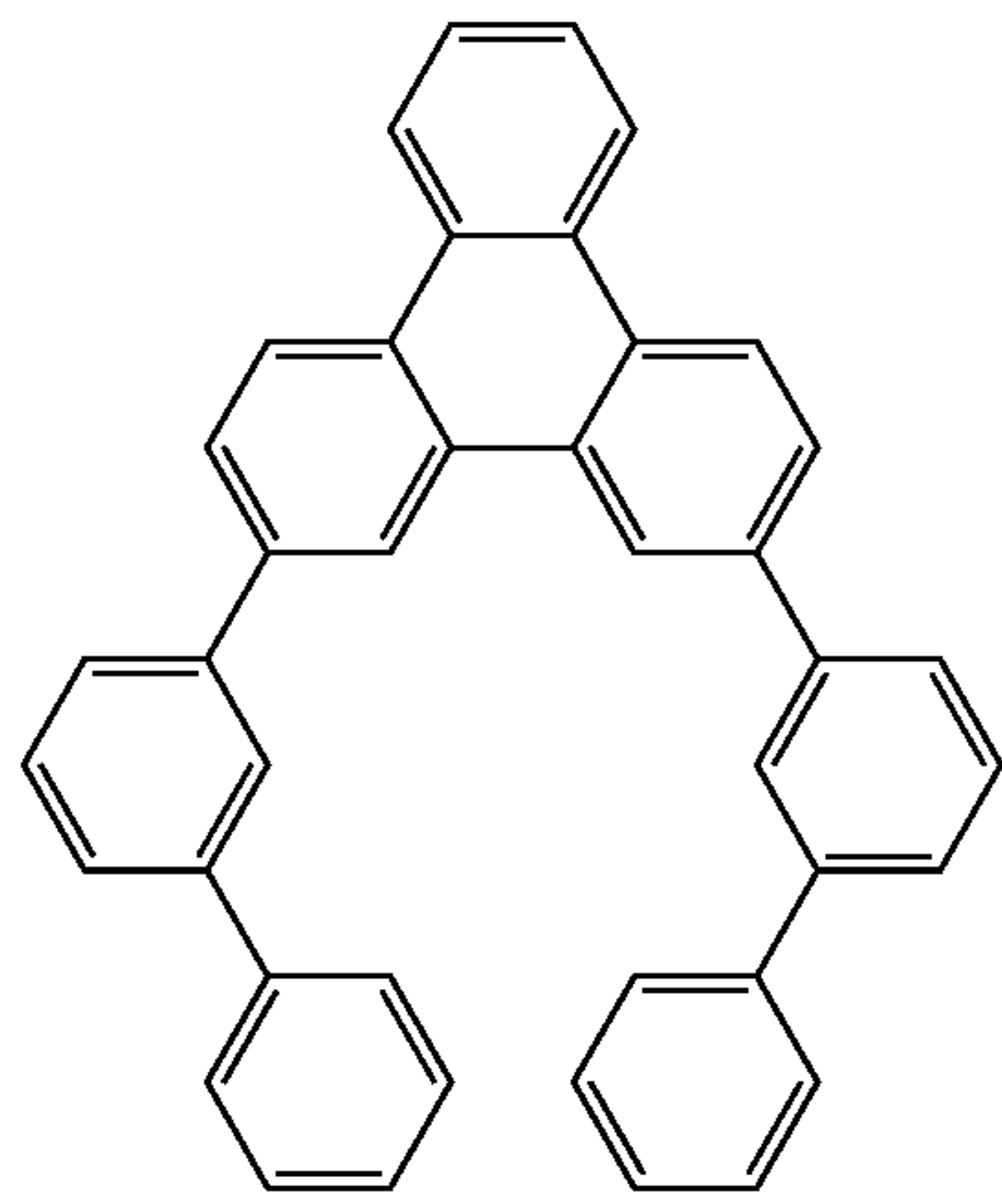
Compound 12
