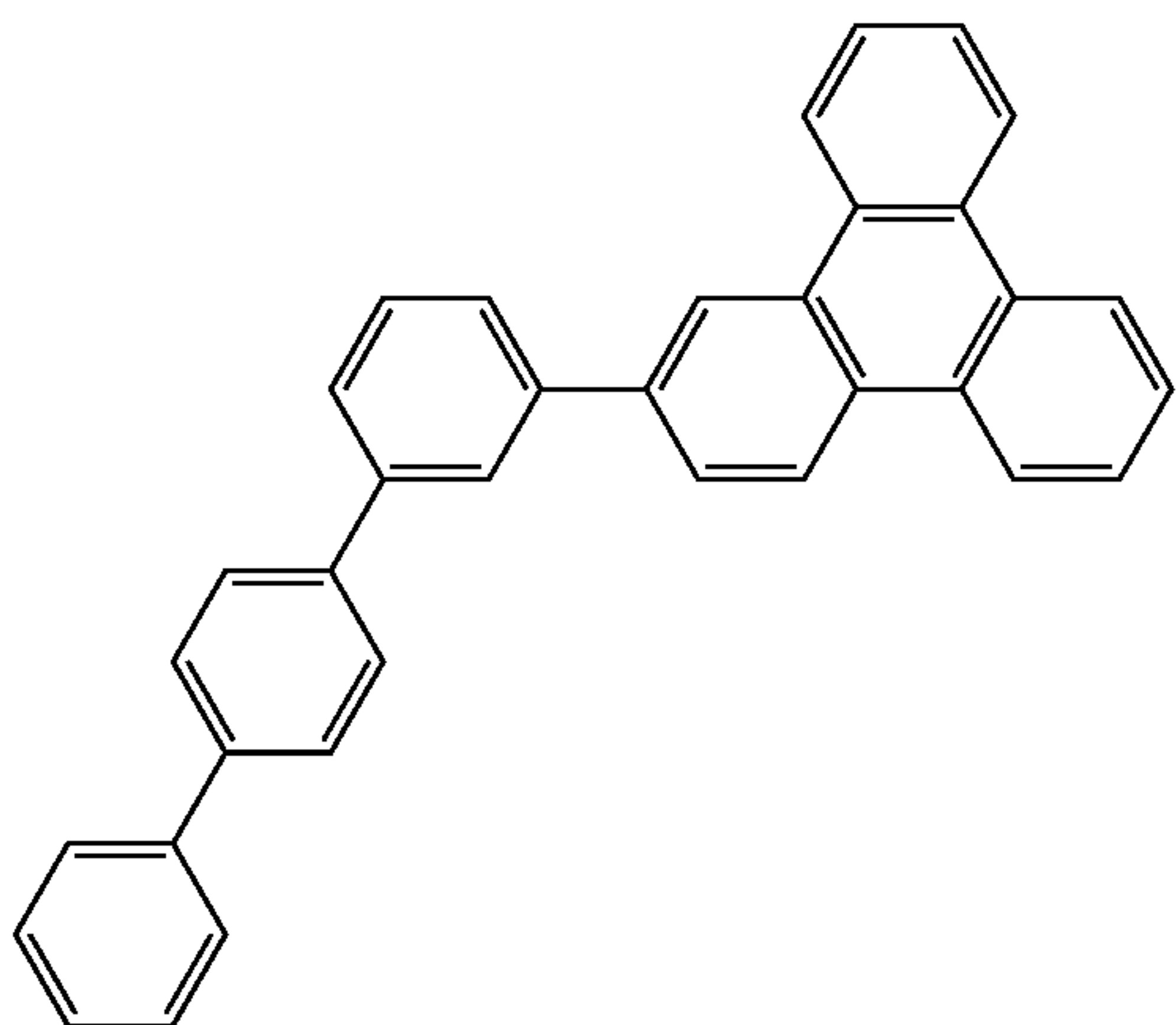
Compound 6
