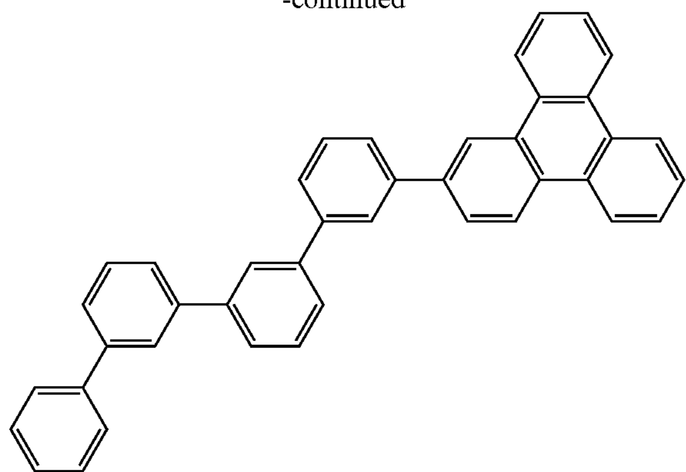
Compound 3
