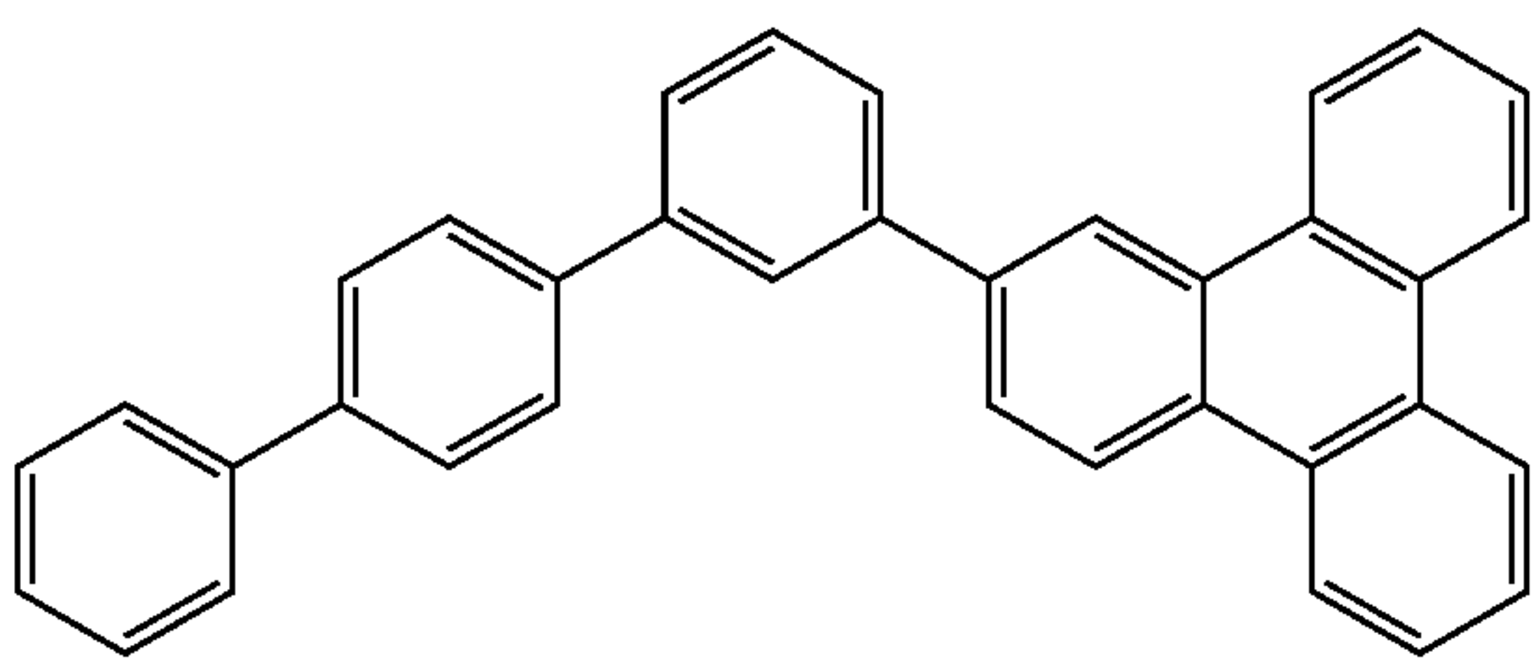
Compound 6
