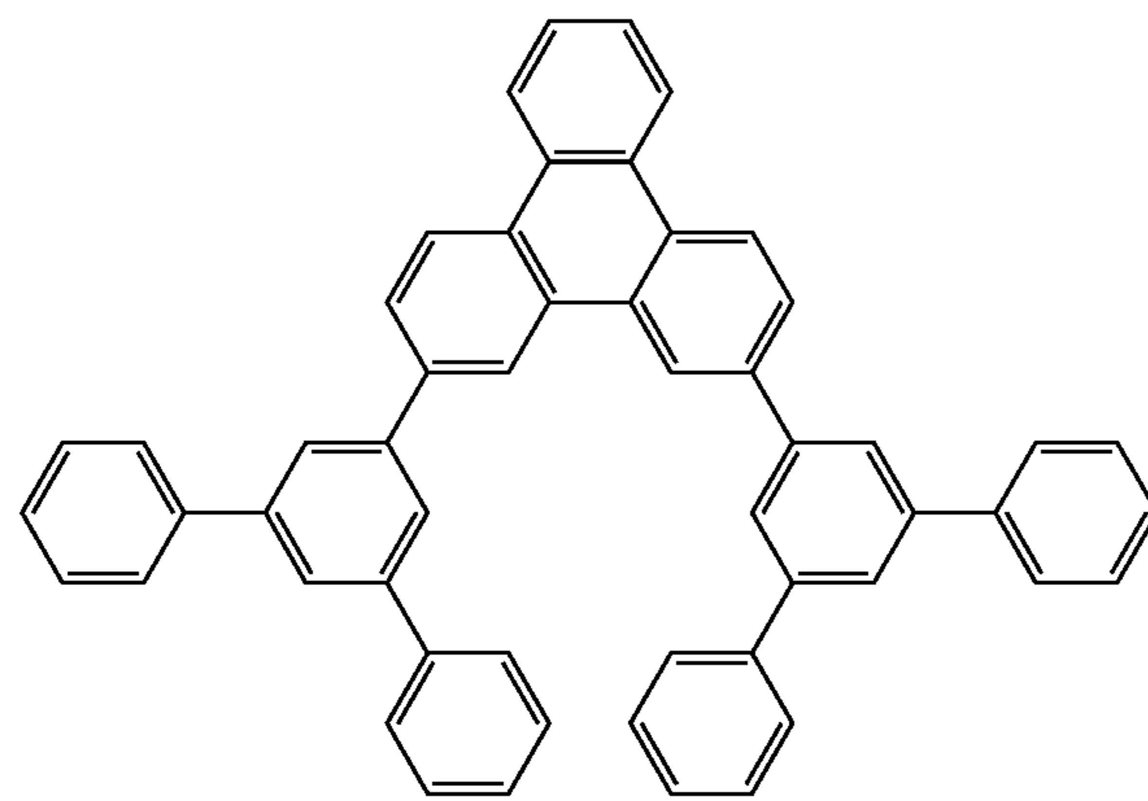
Compound 7
