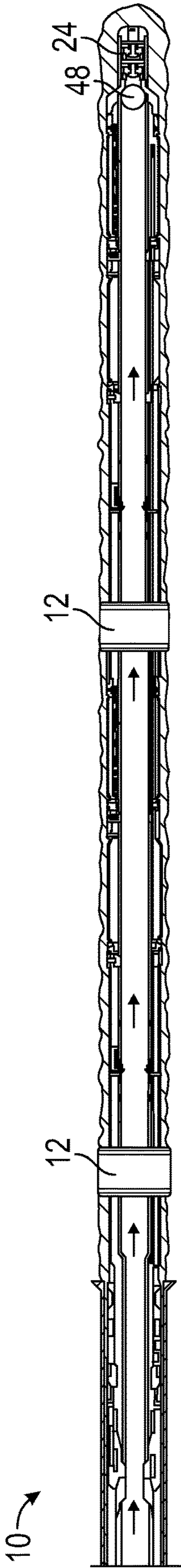
Drop "Shoe Deactivation Ball" and Set Packers FIG. 6D
