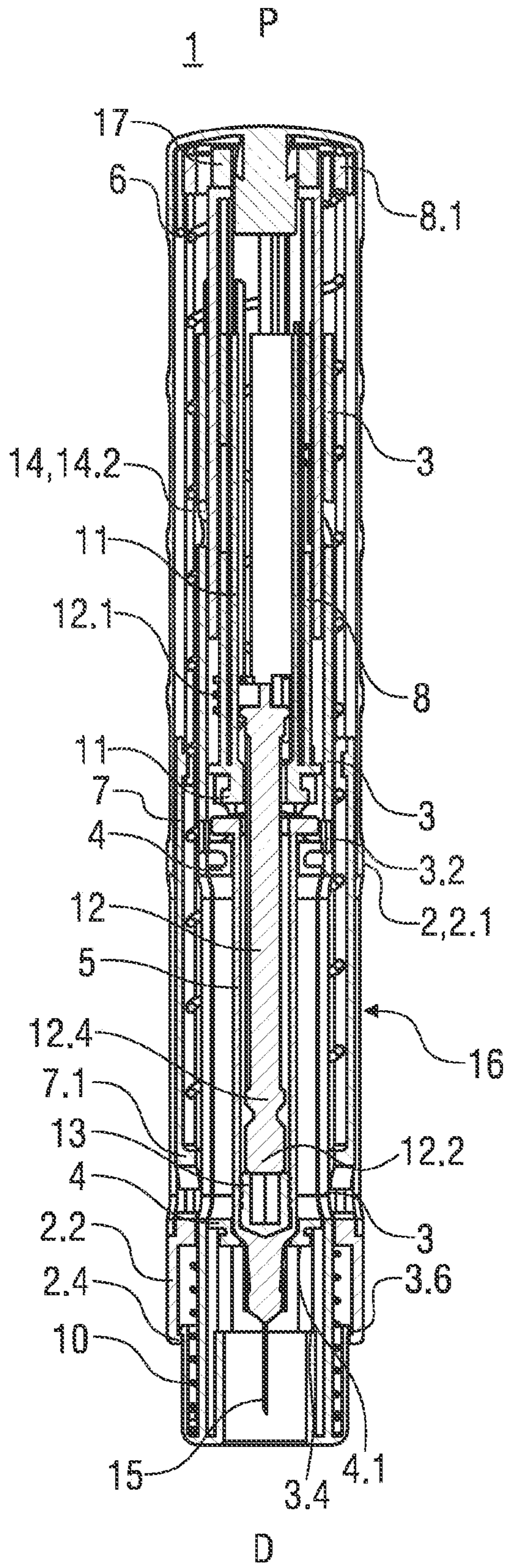
FIG 10B
