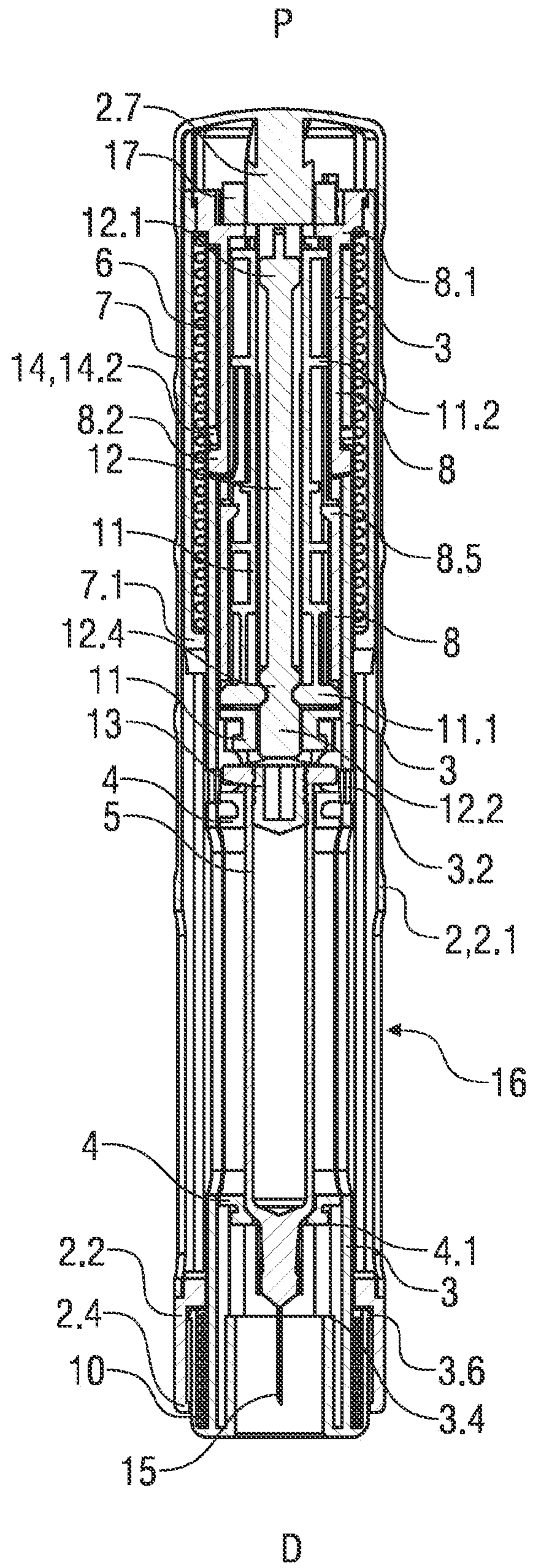
FIG 5B
