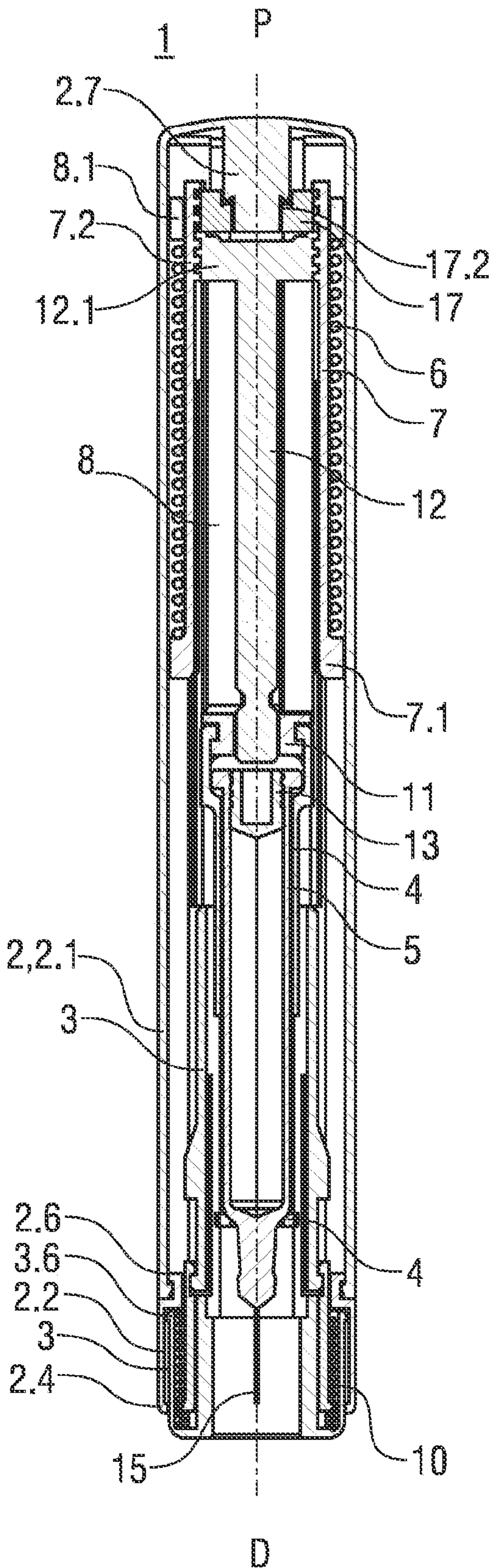
FIG 5A
