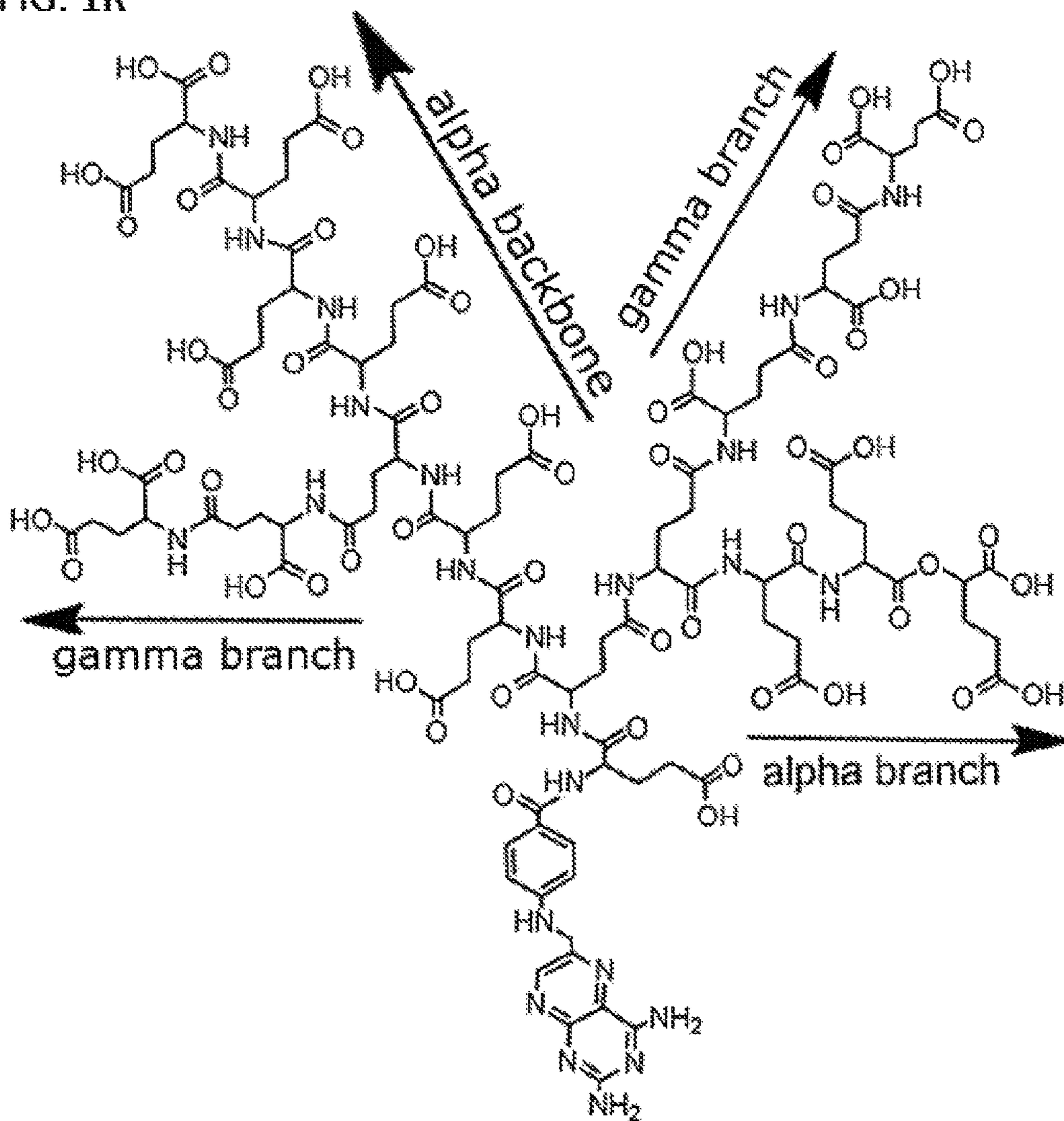
Alpha glutamyl backbone gamma glutamyl branches
