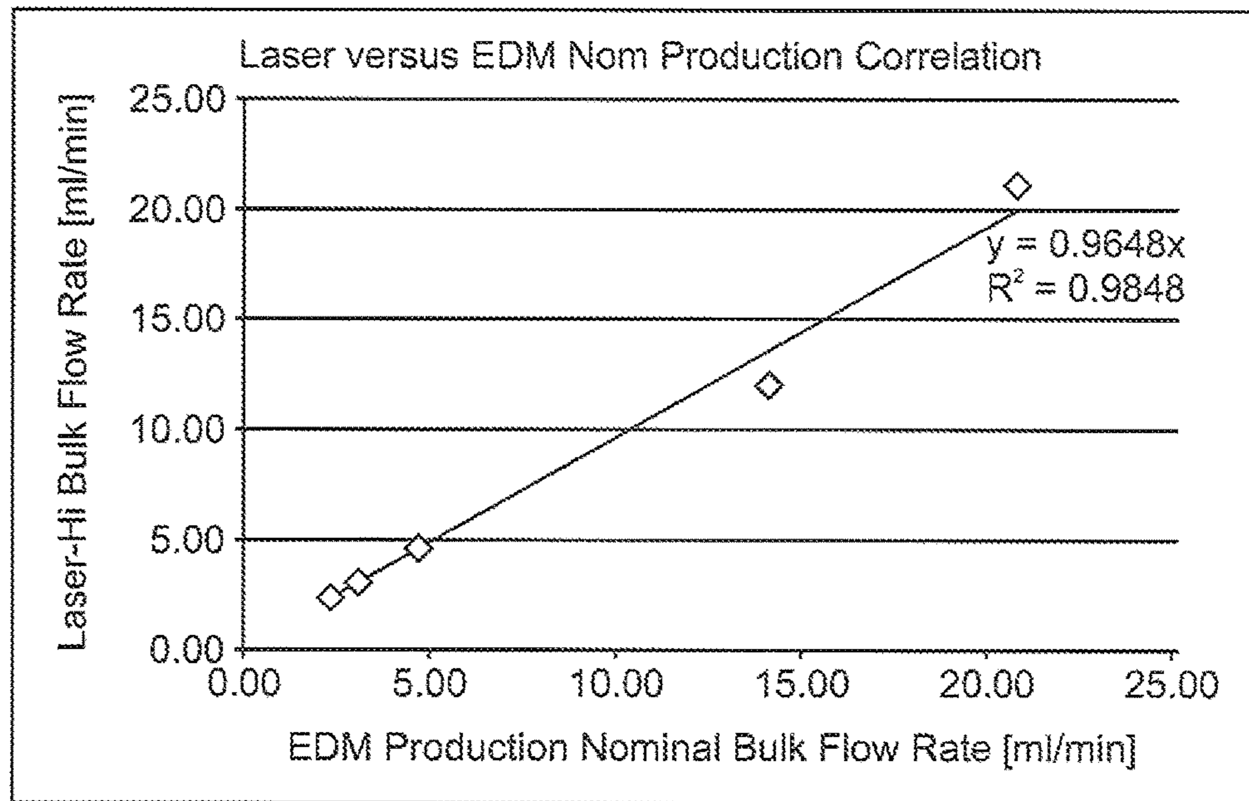
Correlation of Laser and EDM Tips
