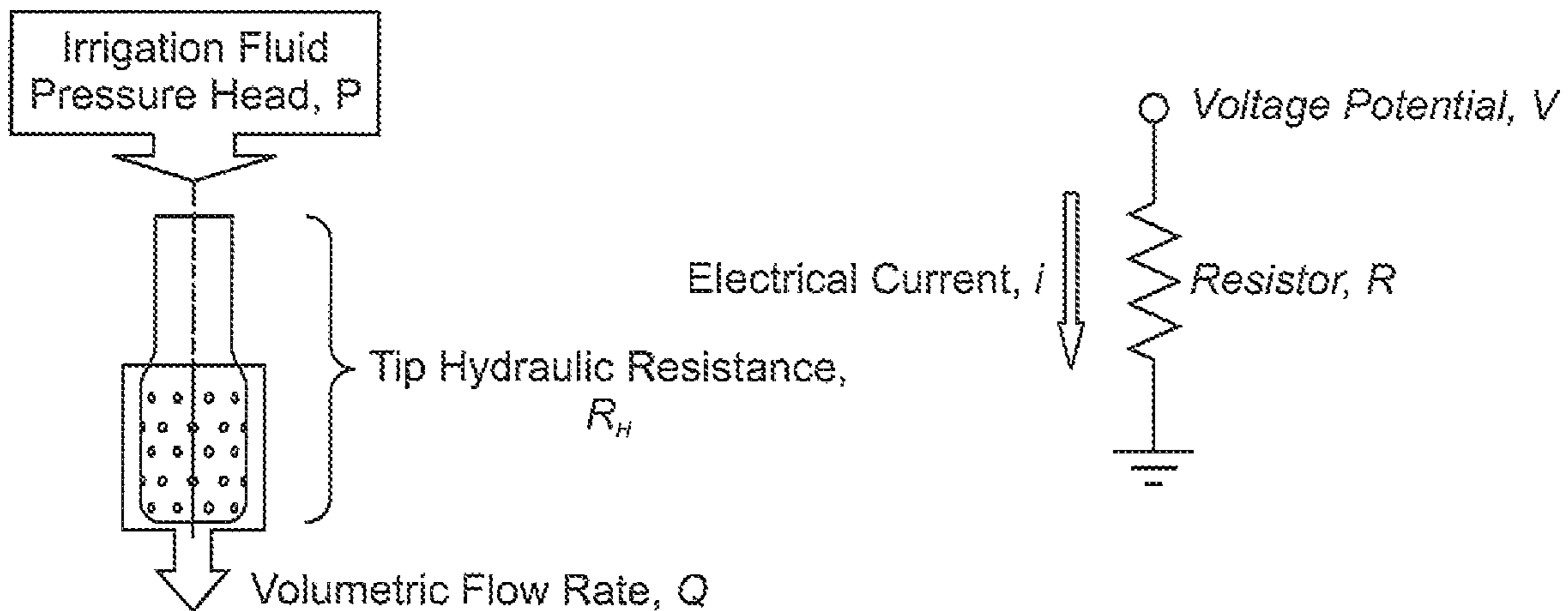
Irrigated Tip Shell Hydraulic and Electrical Analogs
