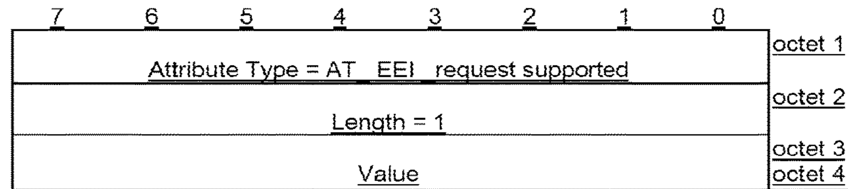
Figure 8.2.X.1-1: AT EI Request Supported attribute
