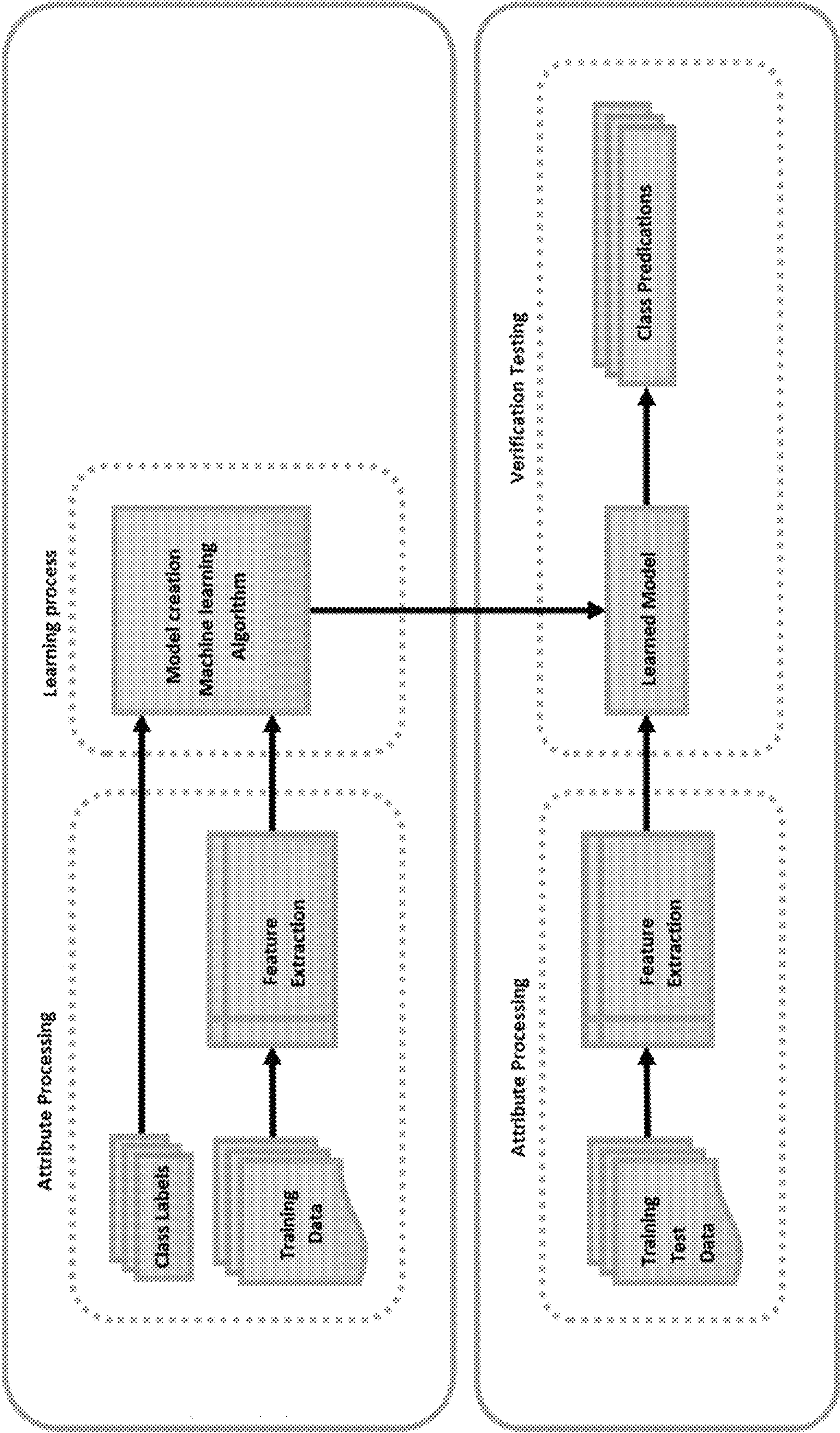
Machine Learning Model Creation Process
