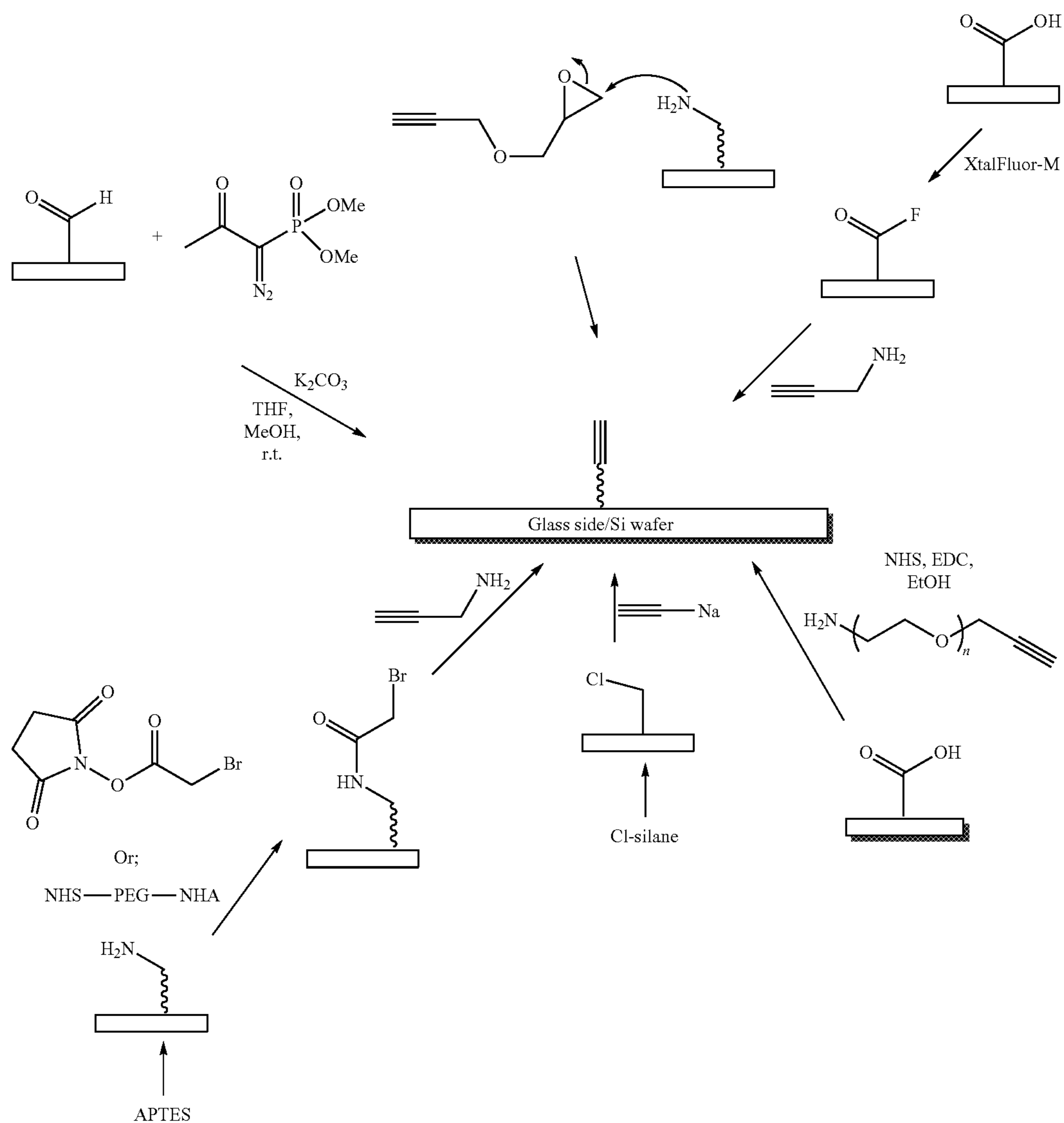
Scheme 3. Suggested Synthetic Routes for Preparing Alkyne Functionalized Surfaces
