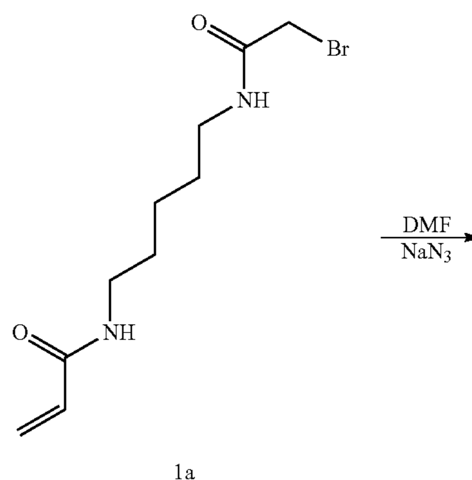
Scheme 1B. Synthesis of a Linear PAZAM
