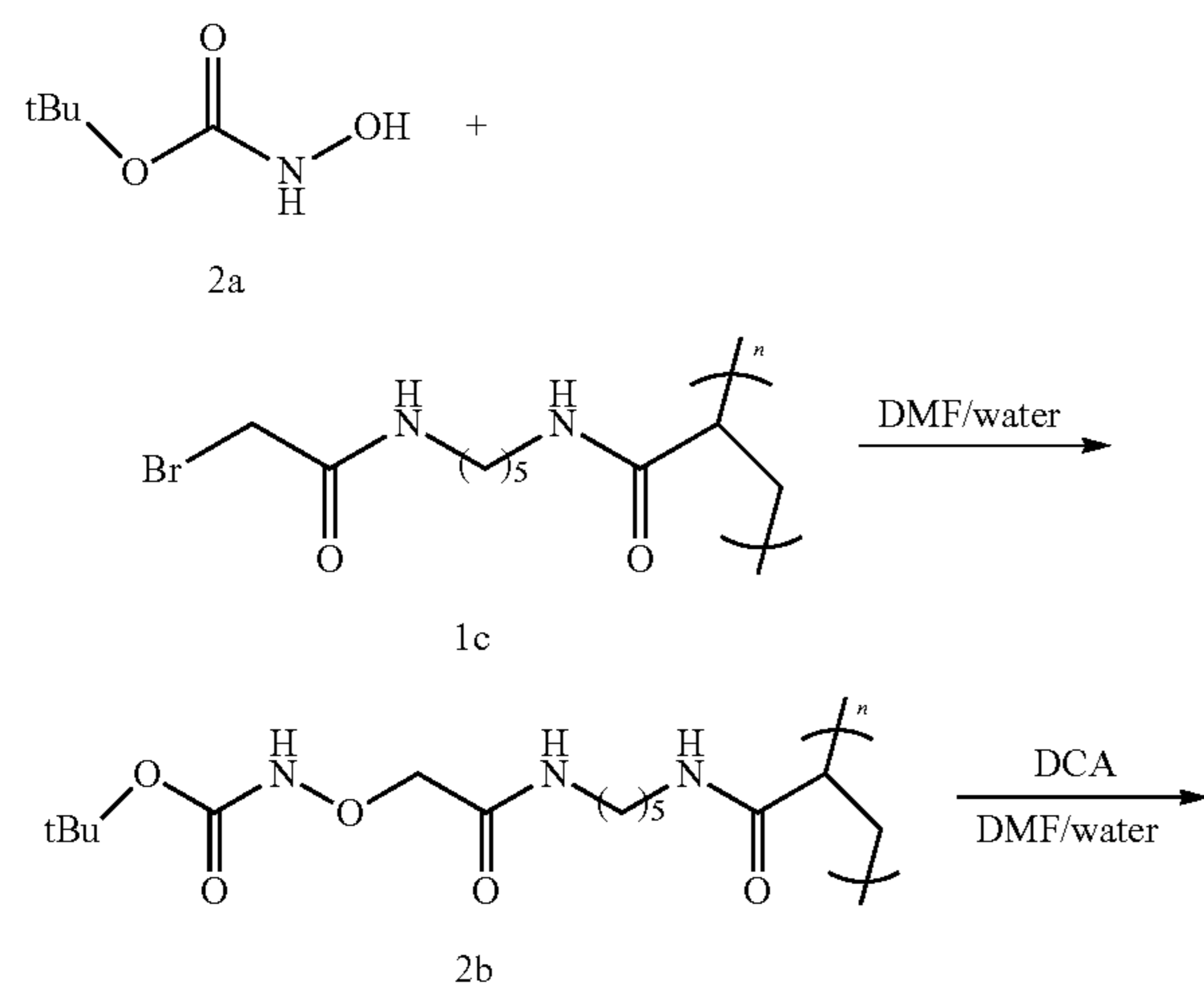
Scheme 2. Synthesis of an oxo-amine derivative of PAZAM
