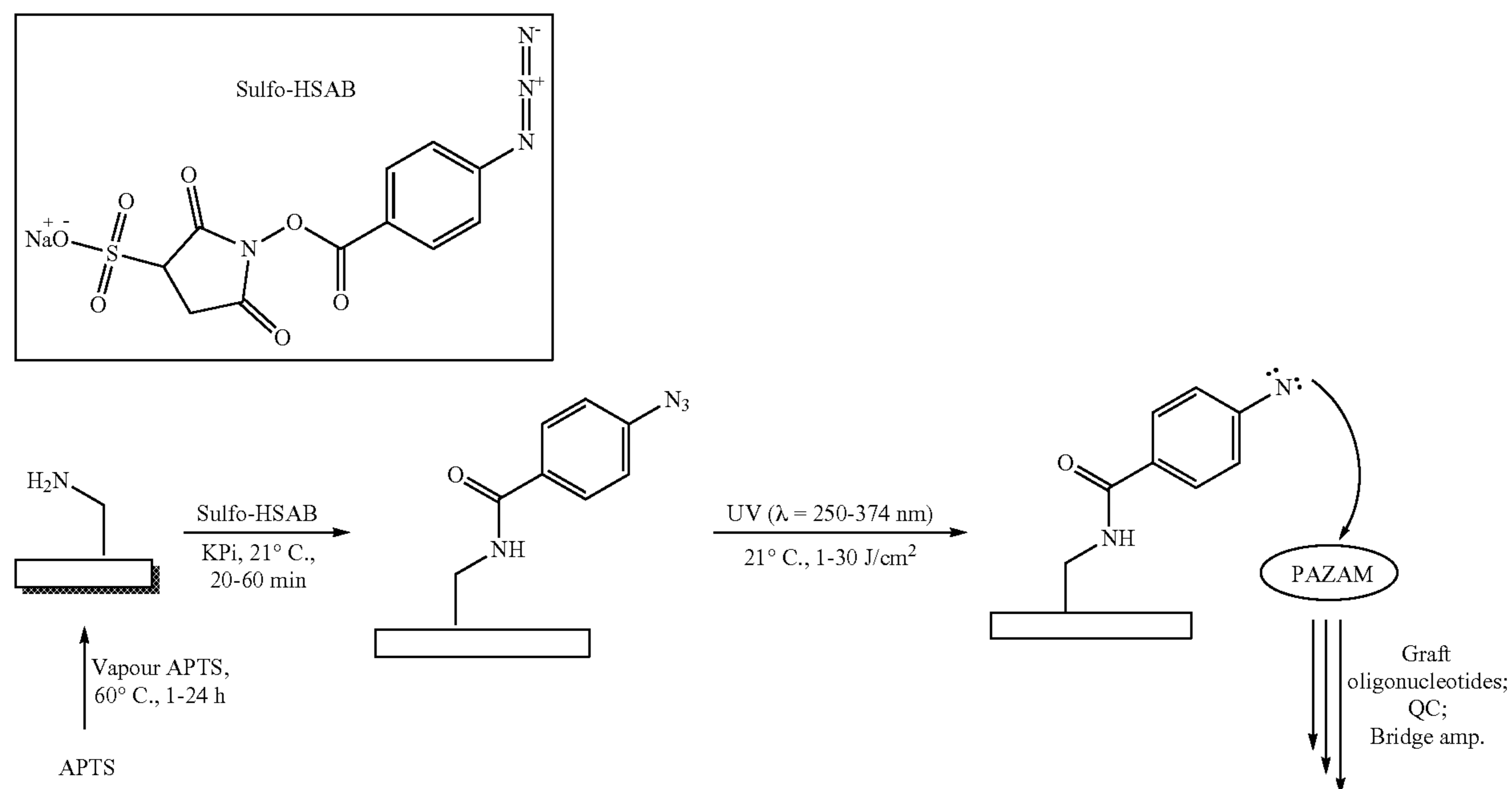
Scheme 4. Pathway Used to Generate a Photoactive Surface
