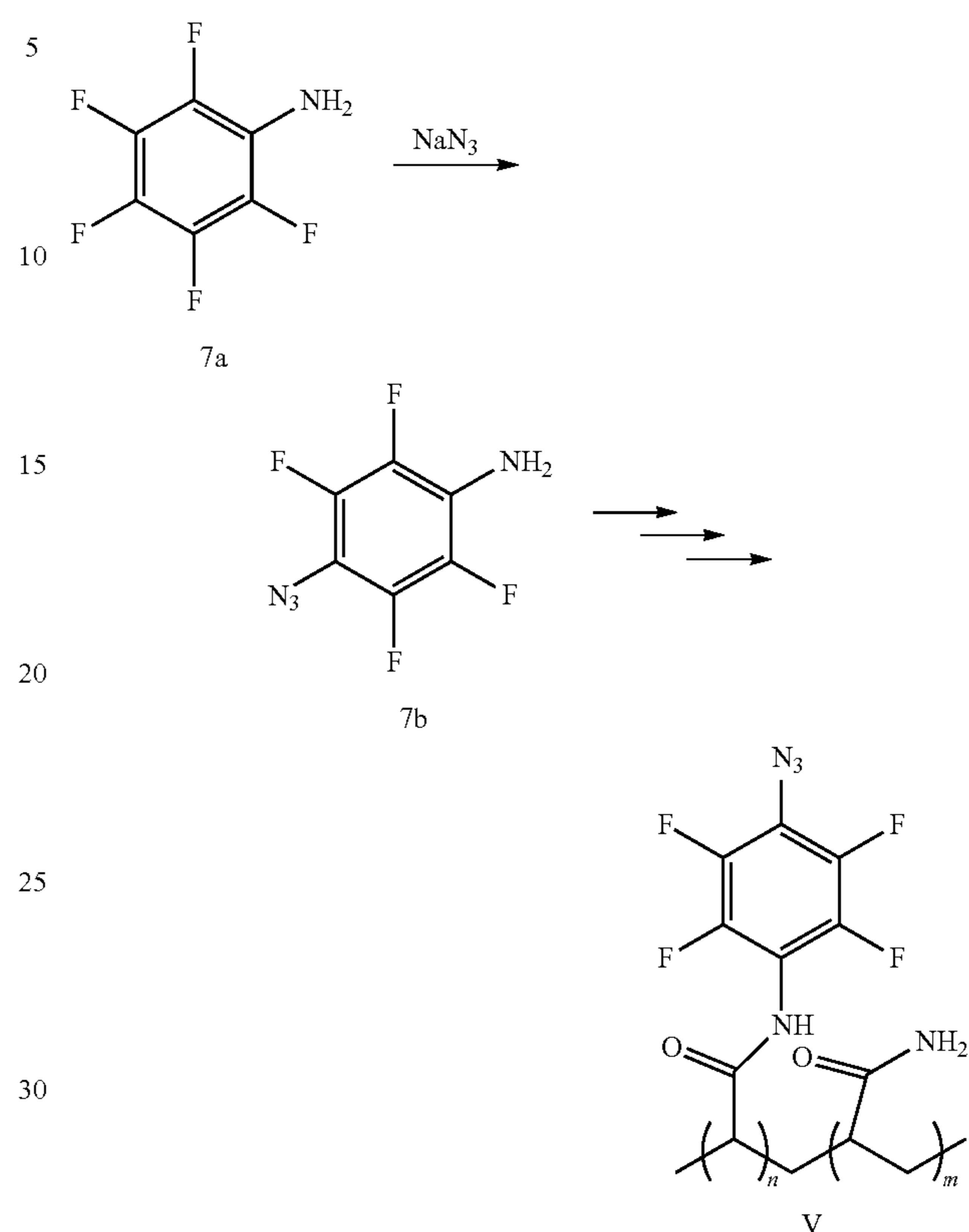
Scheme 7. Synthesis of a Perfluoro Aryl Azide Monomer for Preparing a Photoactive Polymer
