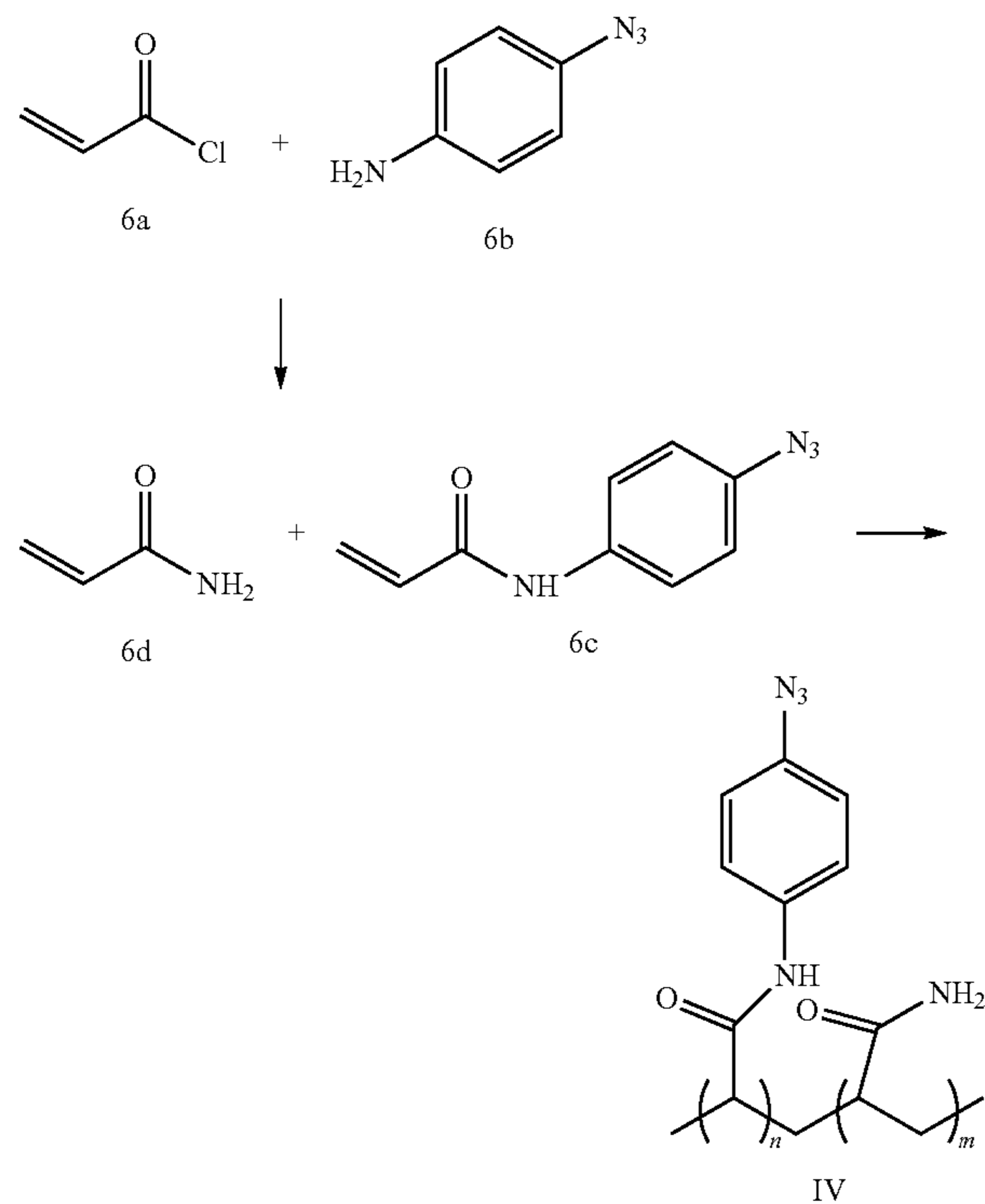
Scheme 6. Synthesis of a Photoactive Linear Polymer
