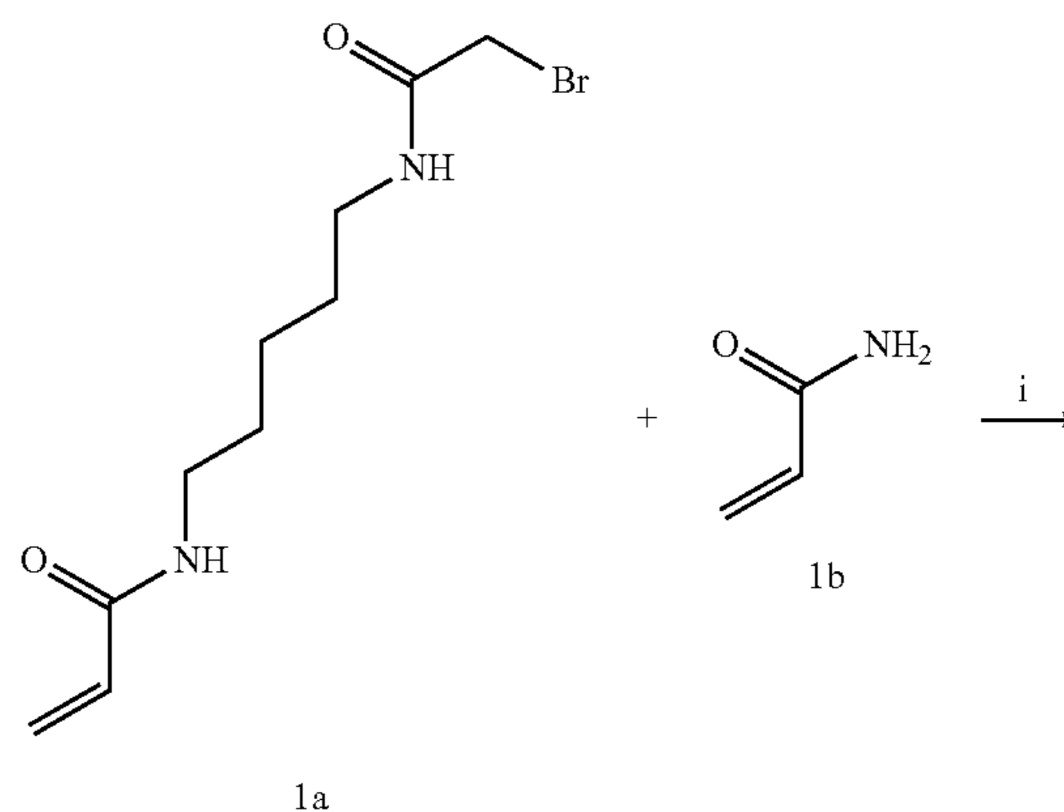
Scheme 1A. Synthesis of solution-state PAZAM mixture
