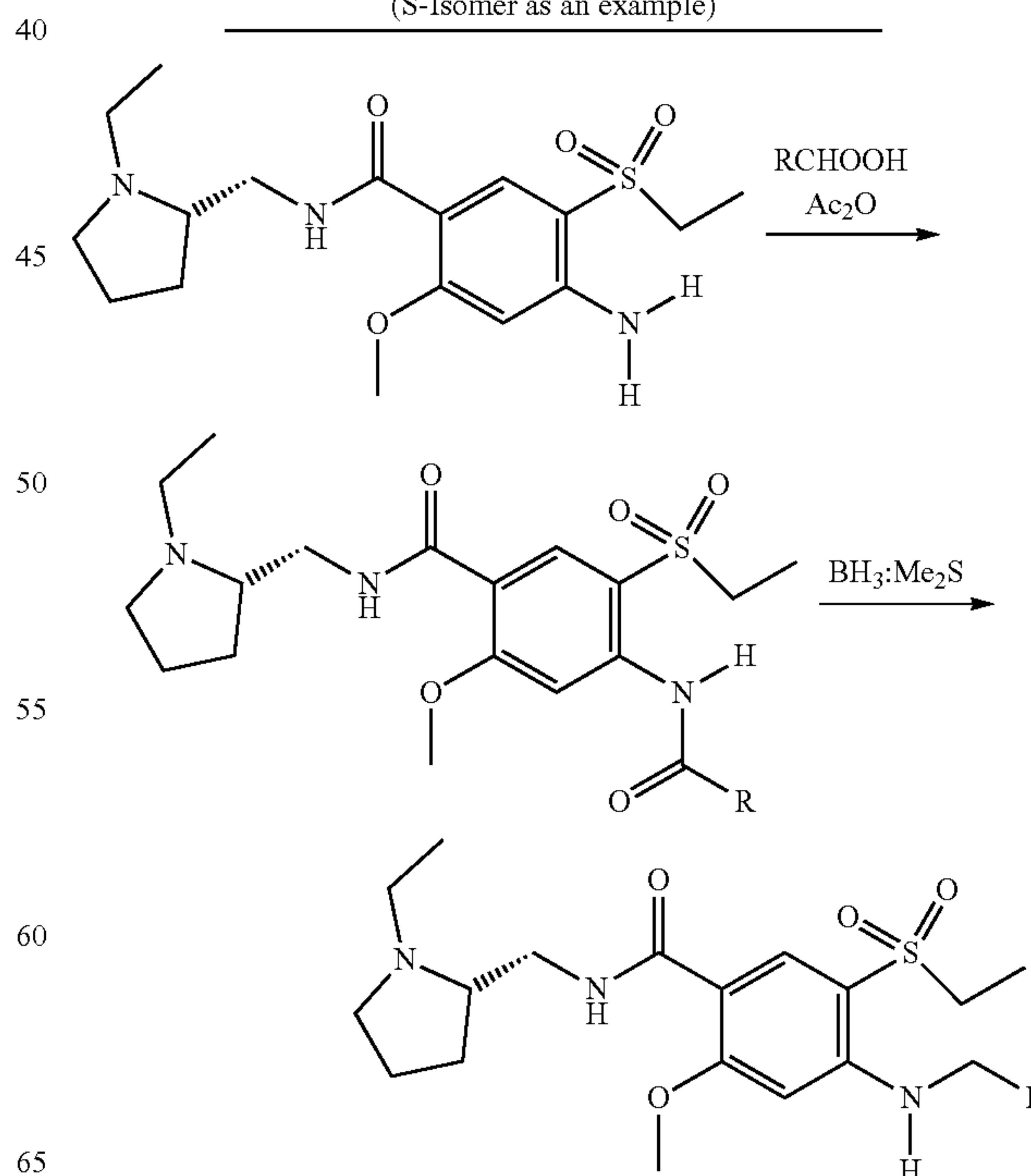
Scheme 3. Preparation of Amisulpride Derivatives (S-Isomer as an example)
