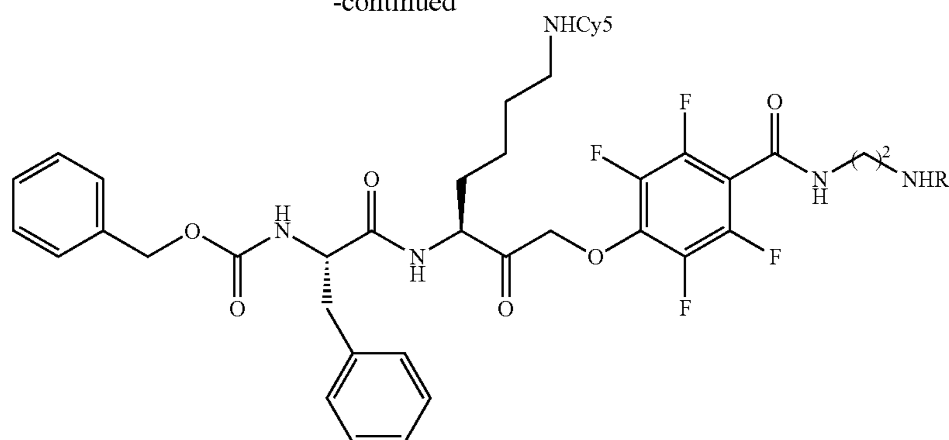
7 (BMV108) R = QSY21 8 (BMV109) R = Sulfo-QSY21
