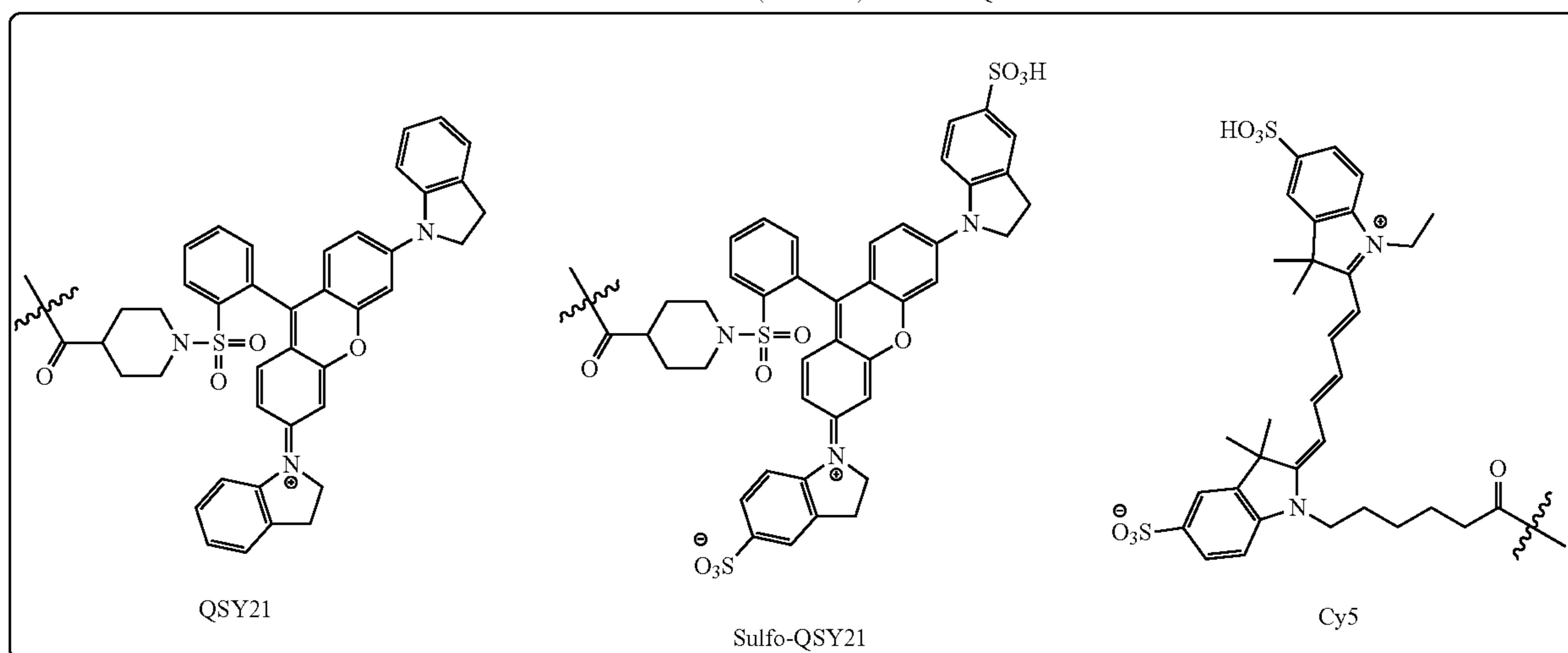
7 (BMV108) R = QSY21 8 (BMV109) R = Sulfo-QSY21
