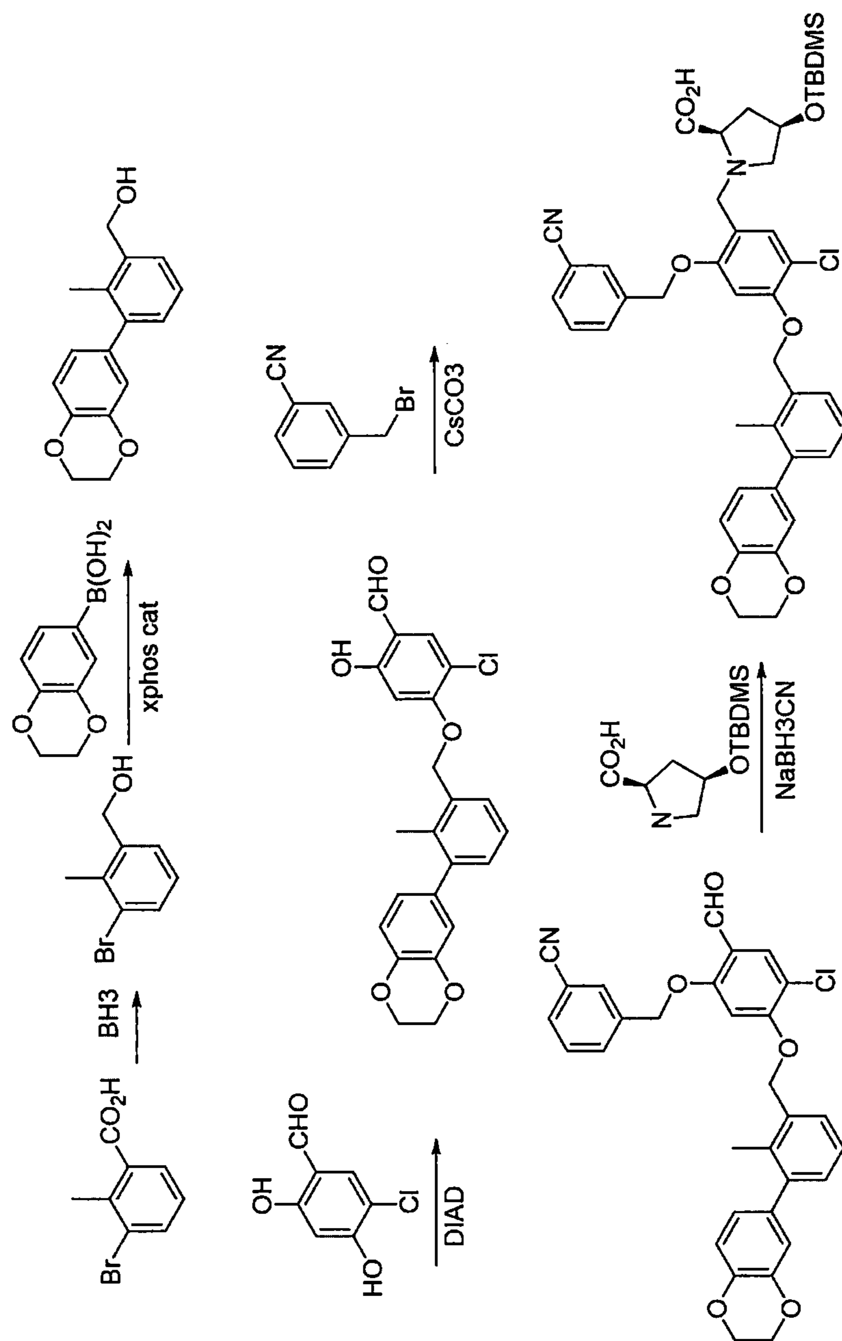
Figure 1. Chemical Synthesis for Protected PD3-Prodrug
