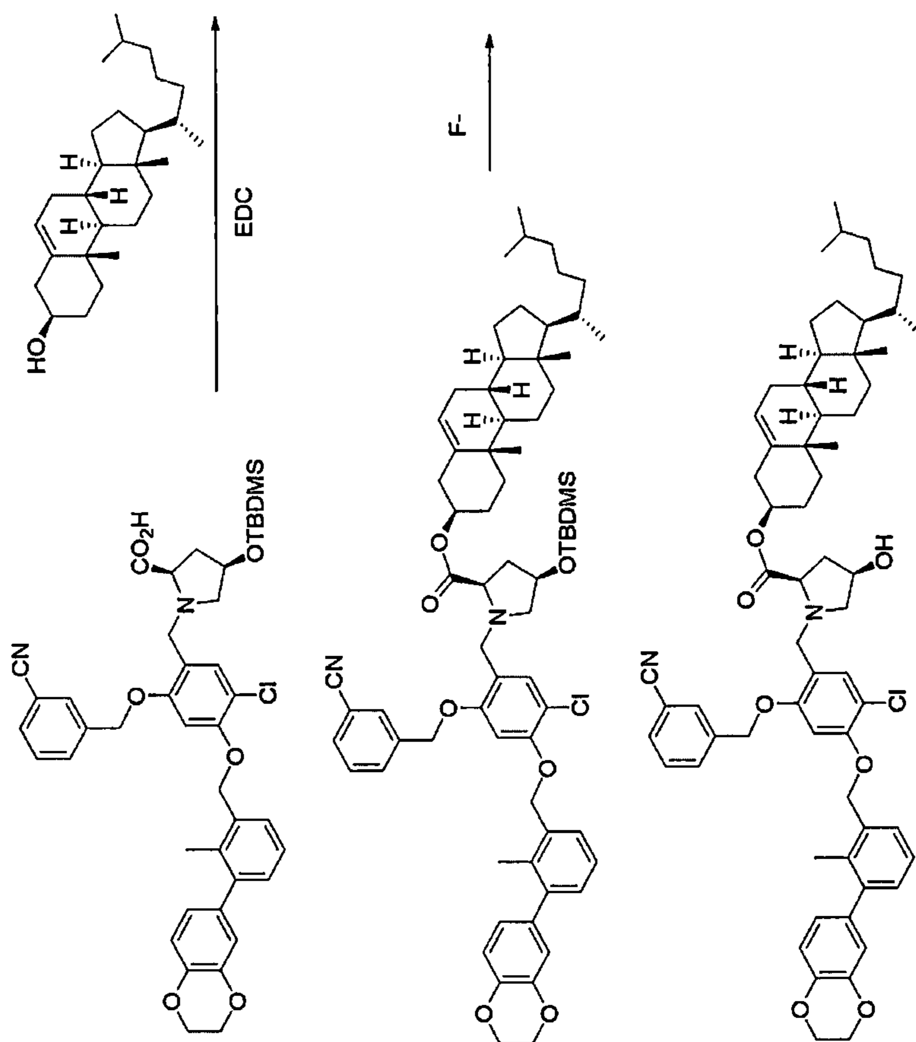
Figure 2. Chemical Synthesis for Protected PD3-Prodrug, continued
