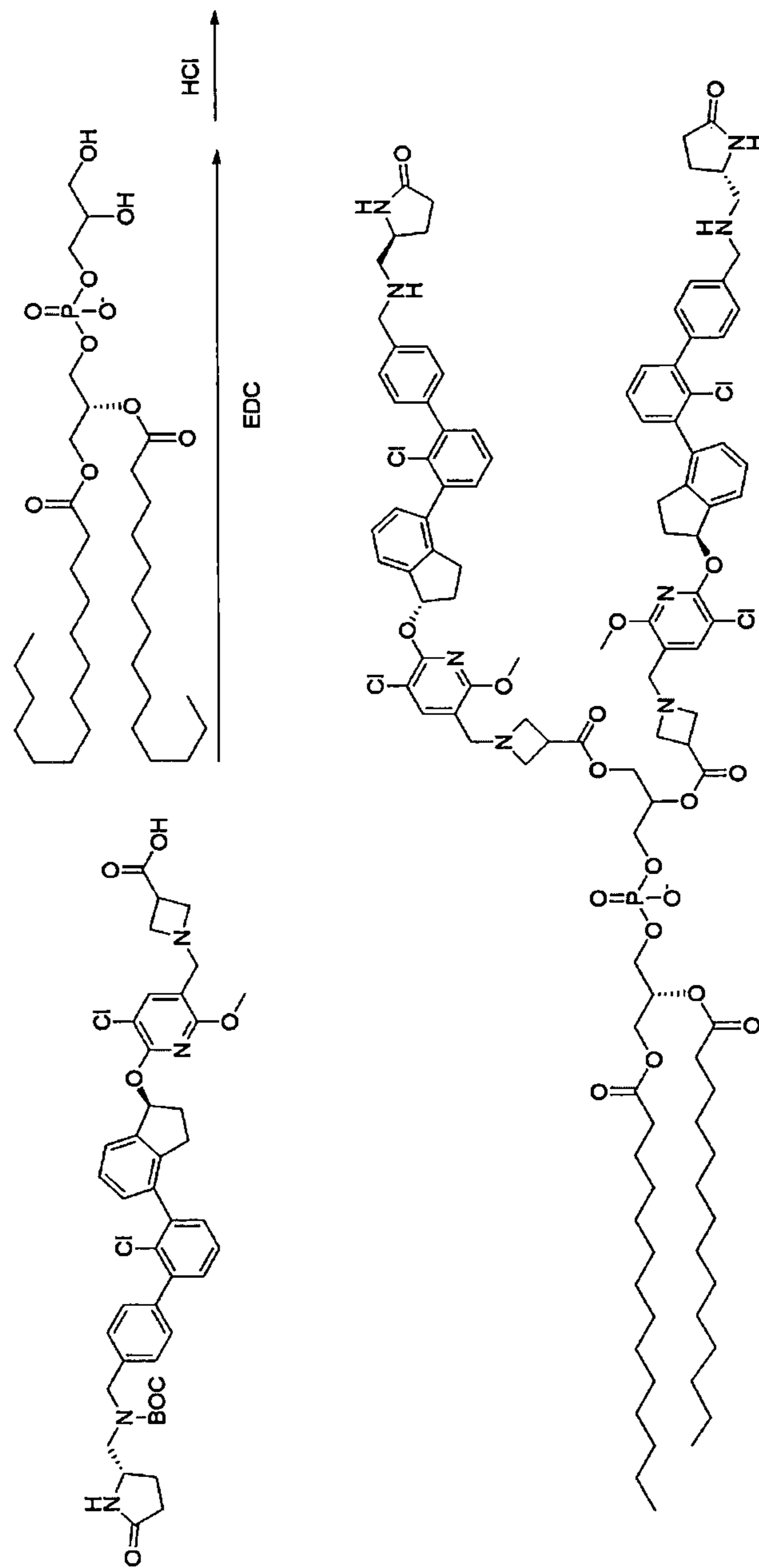
Figure 7. Chemical Synthesis for Protected PD6-Prodrug, Continued
