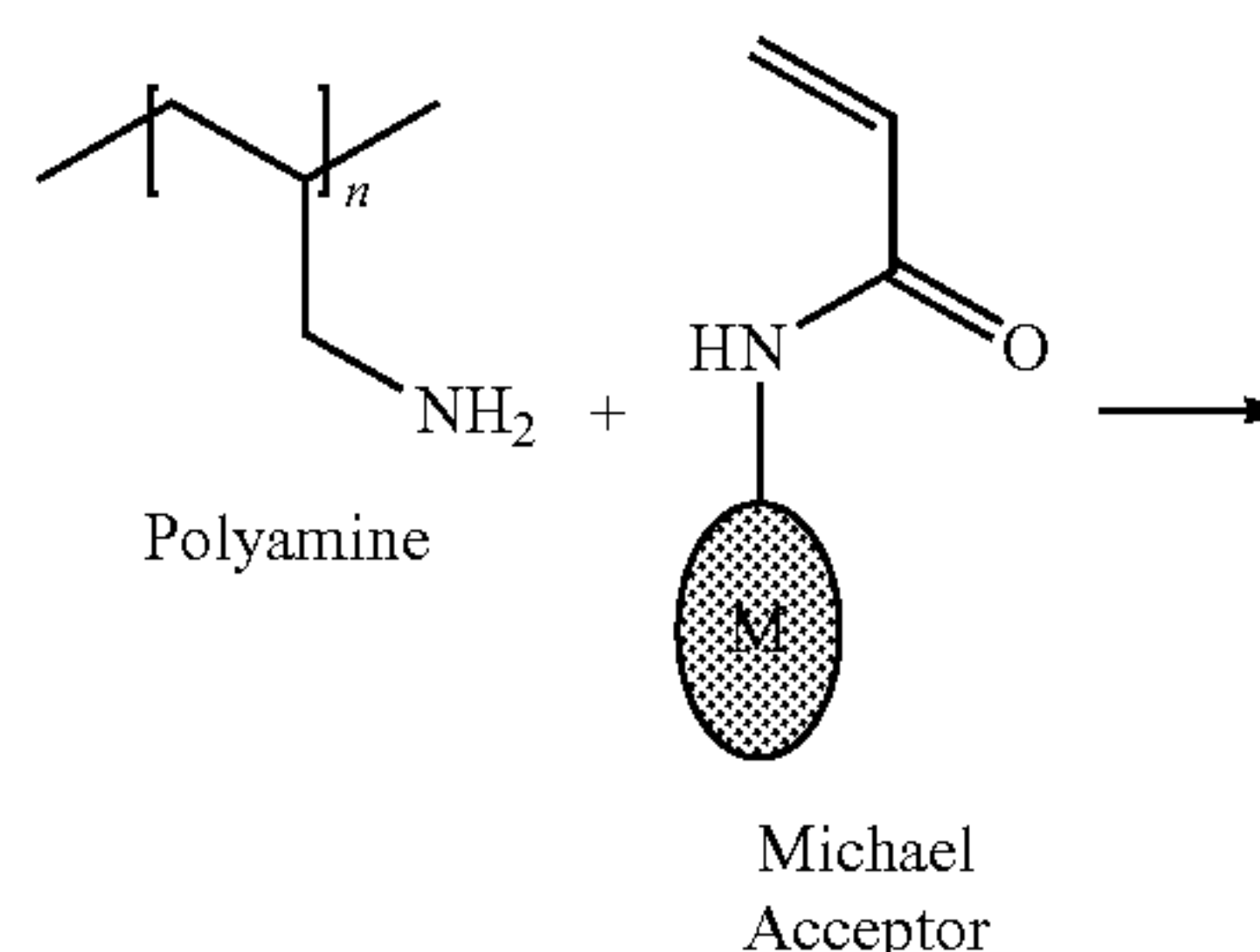
Scheme 2: Michael addition reaction of a polyamine nucleophile with an acrylamides Michael acceptor.
