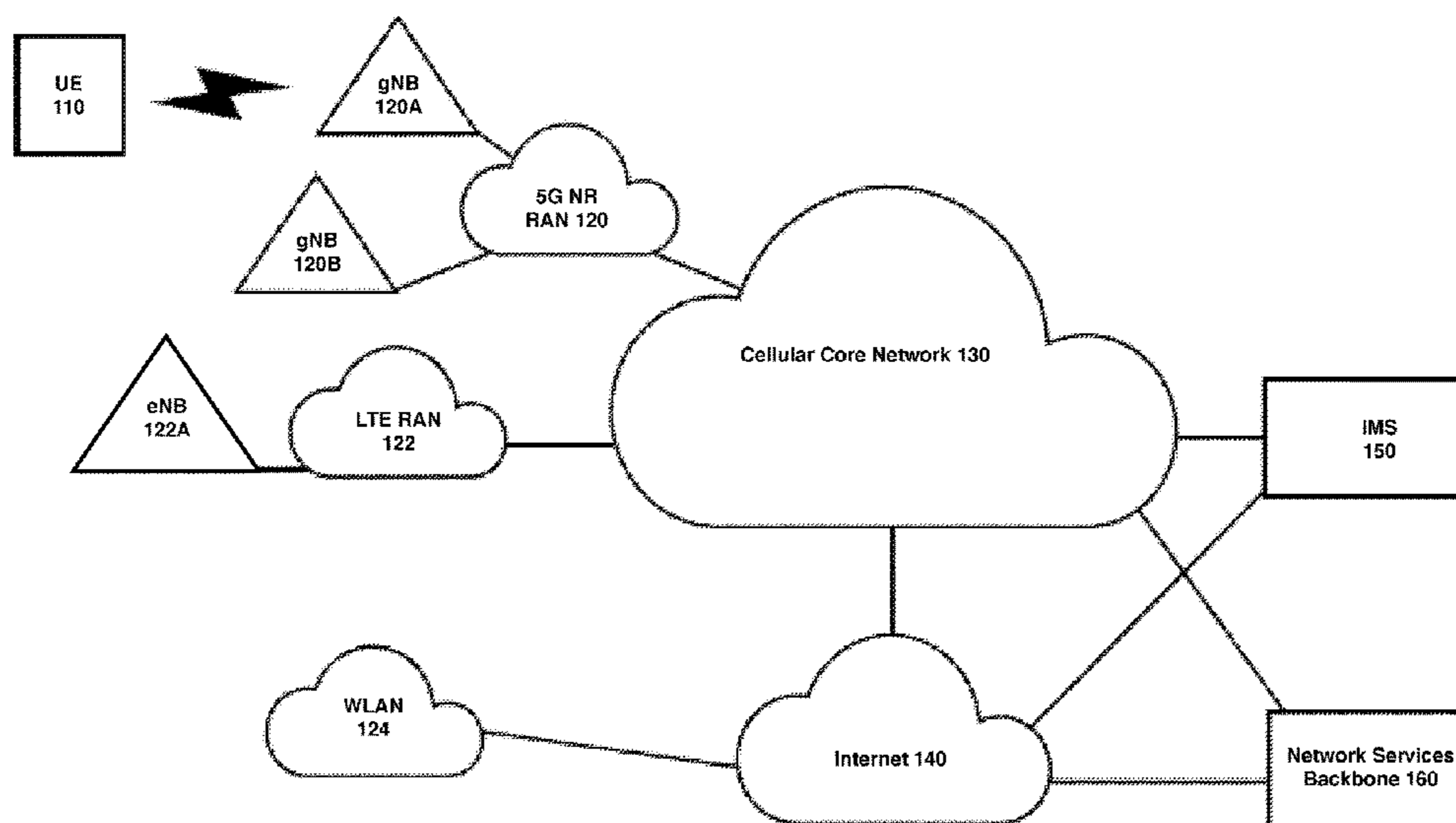
Network Arrangement 100
