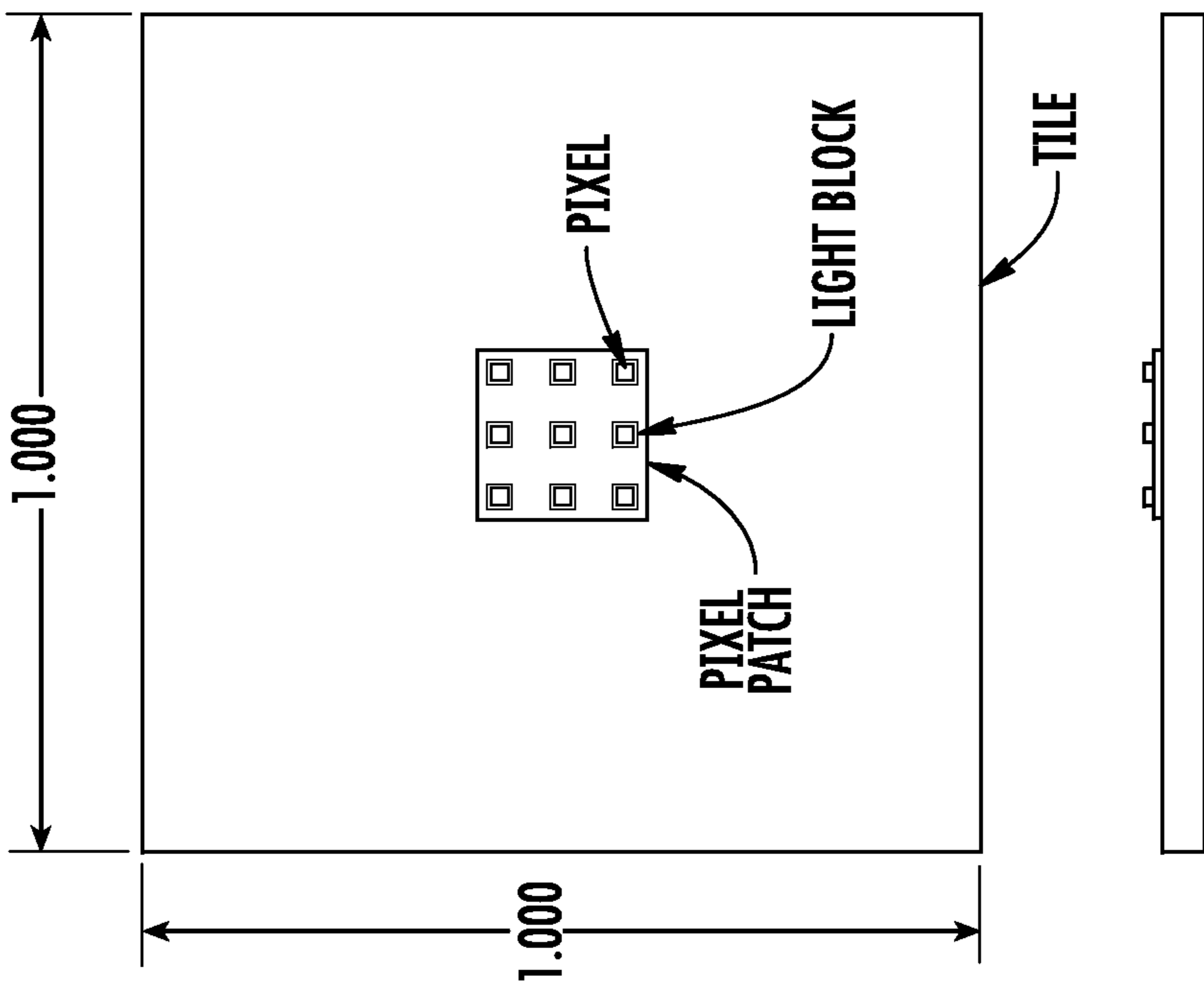
FRONT VIEW OF A TILE WITH ONE PIXEL PATCH
