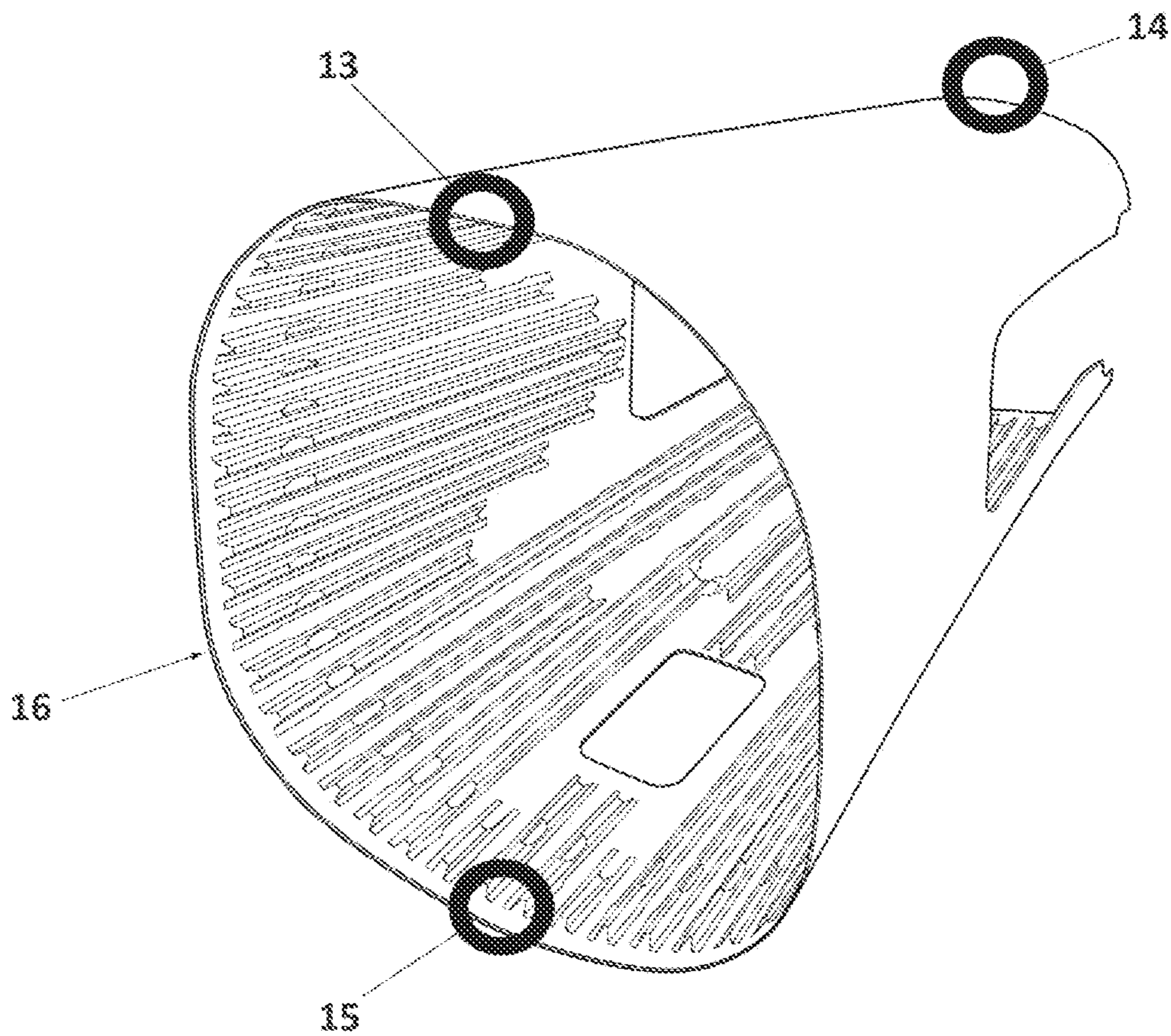
FIG. 2 Prior Art
