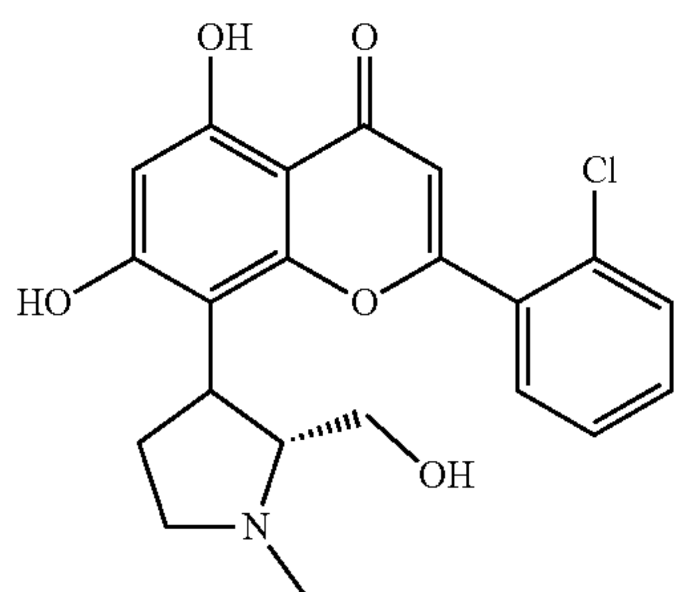
P276-00
