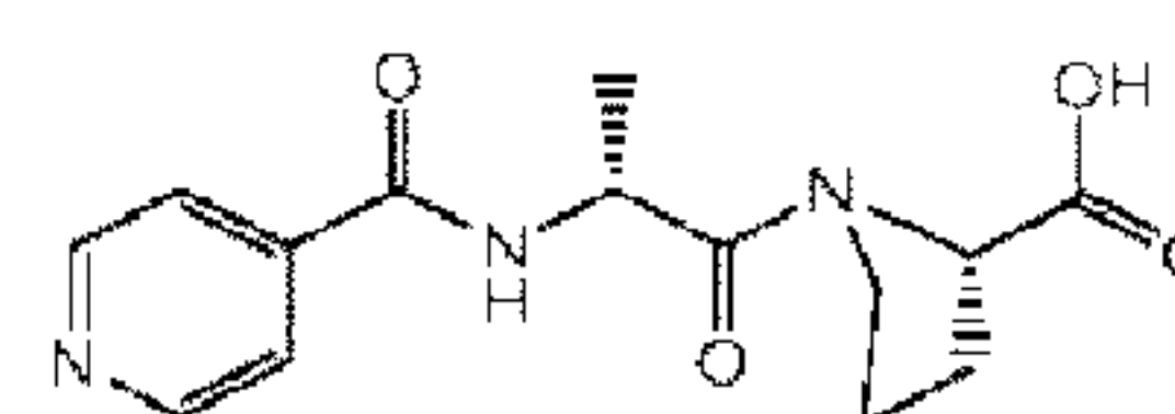
N-((pyridin-4-carbonyl)- D-Ala-L-Proline
