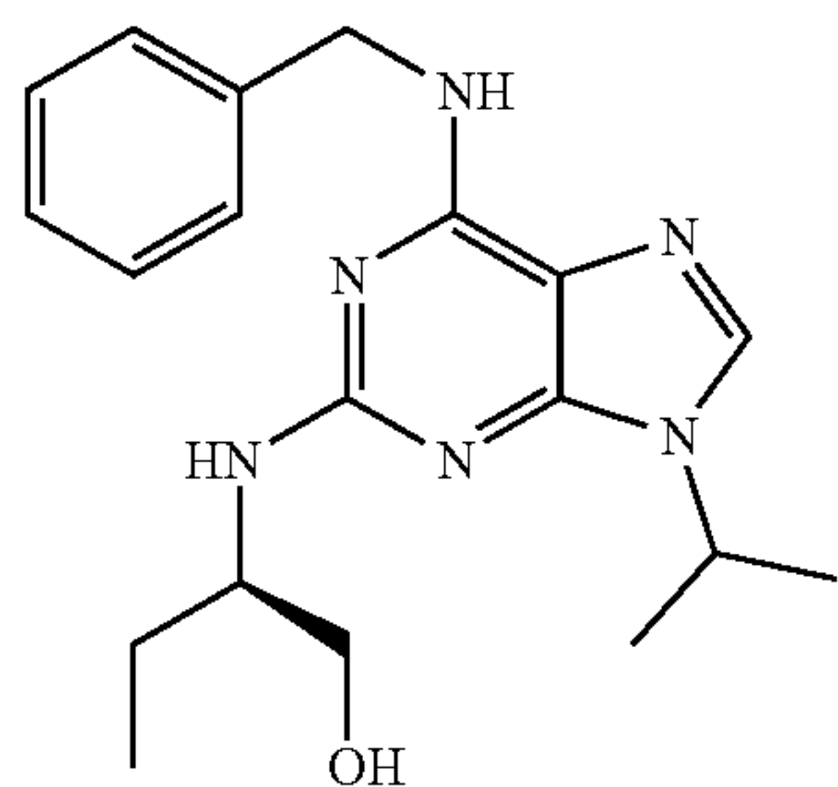
(R)-roscovitine
