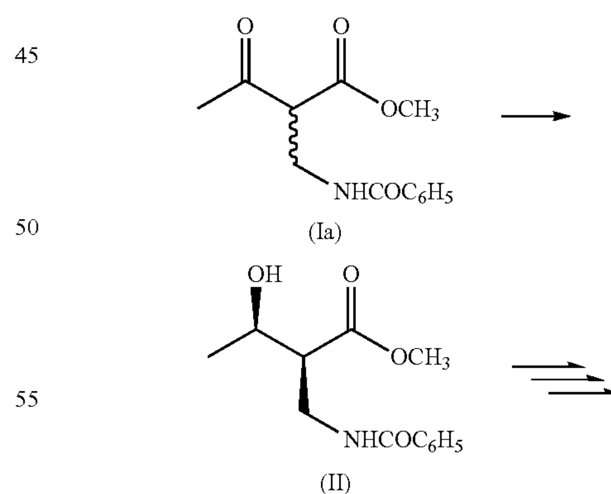
Scheme 3
