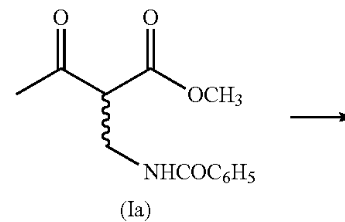
Scheme 3
