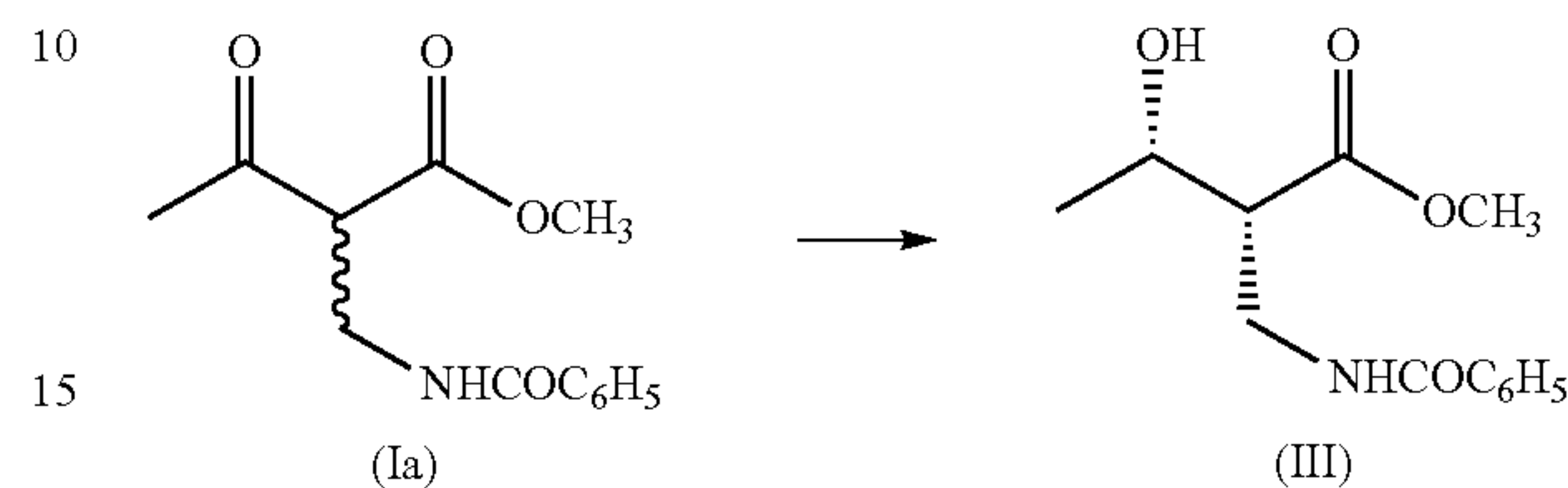
Scheme 2
