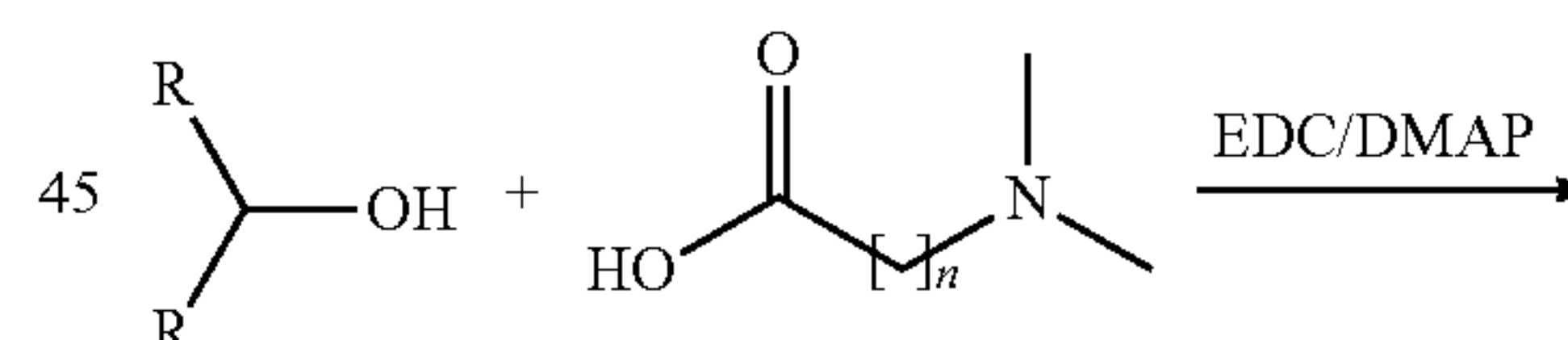
Scheme 1: M series (esters) synthesis
