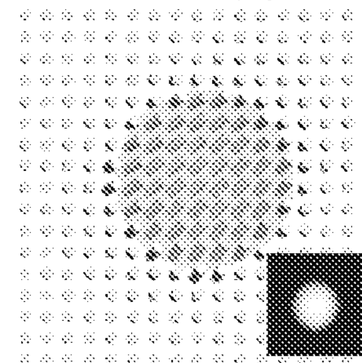
FIG. 1F Uniform (U)
