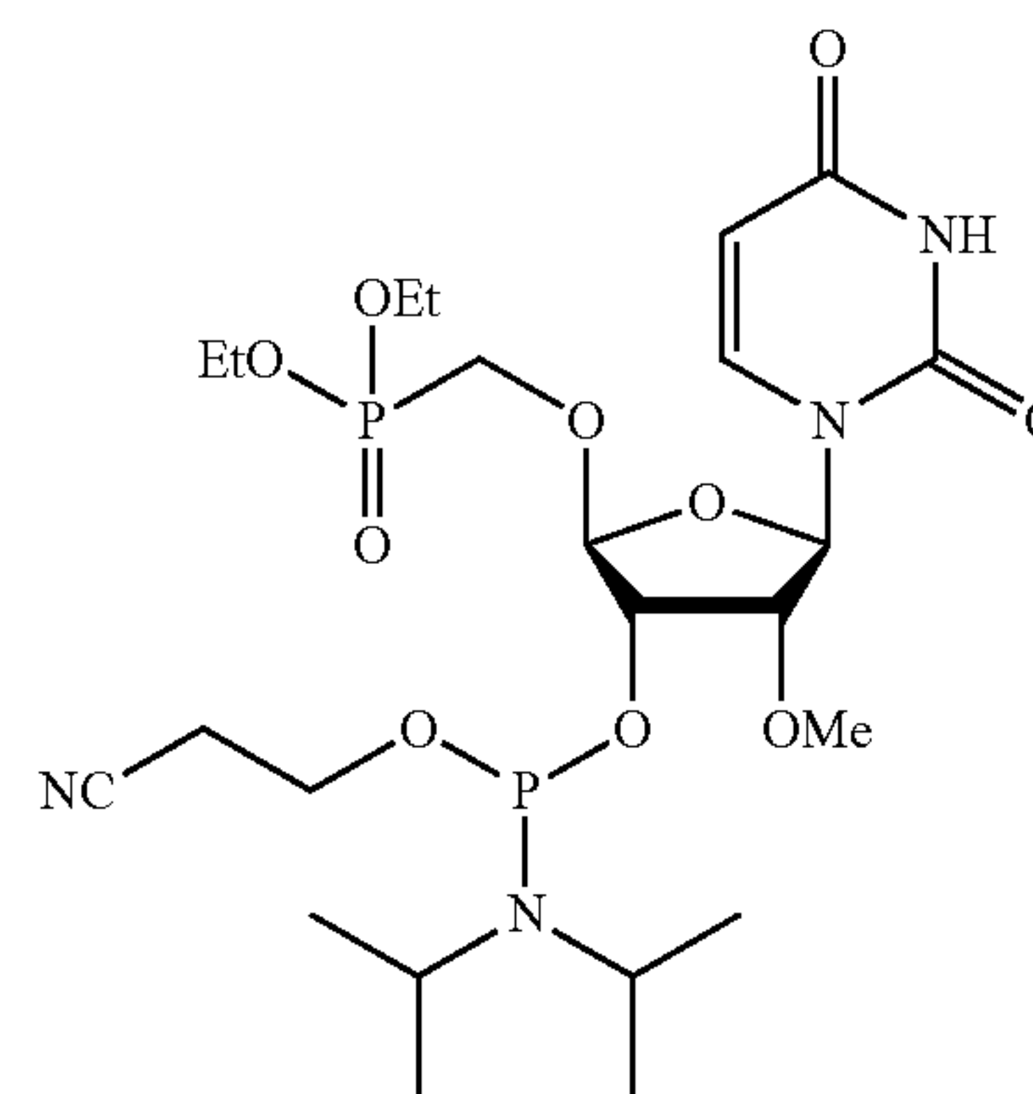
Phosphoramidite 1
