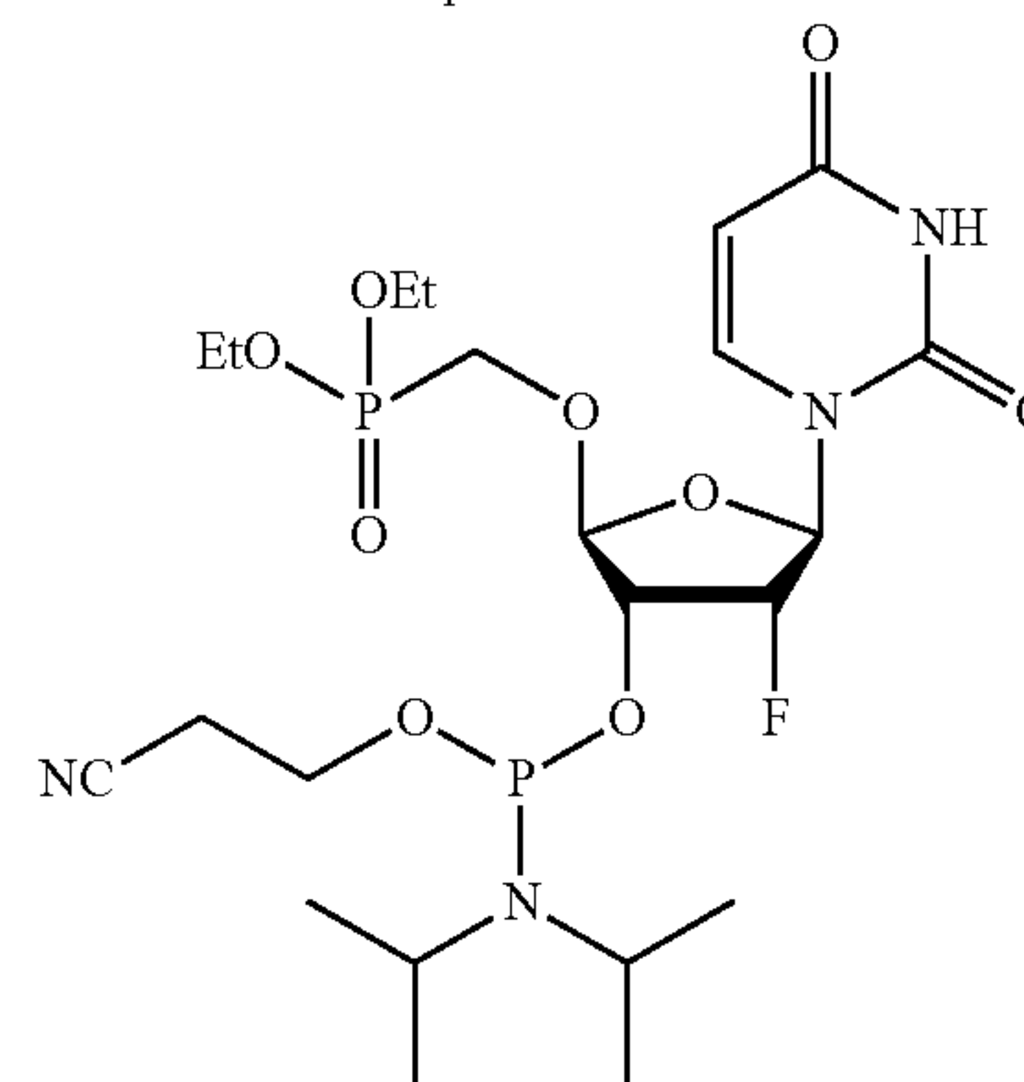
Phosphoramidite 2
