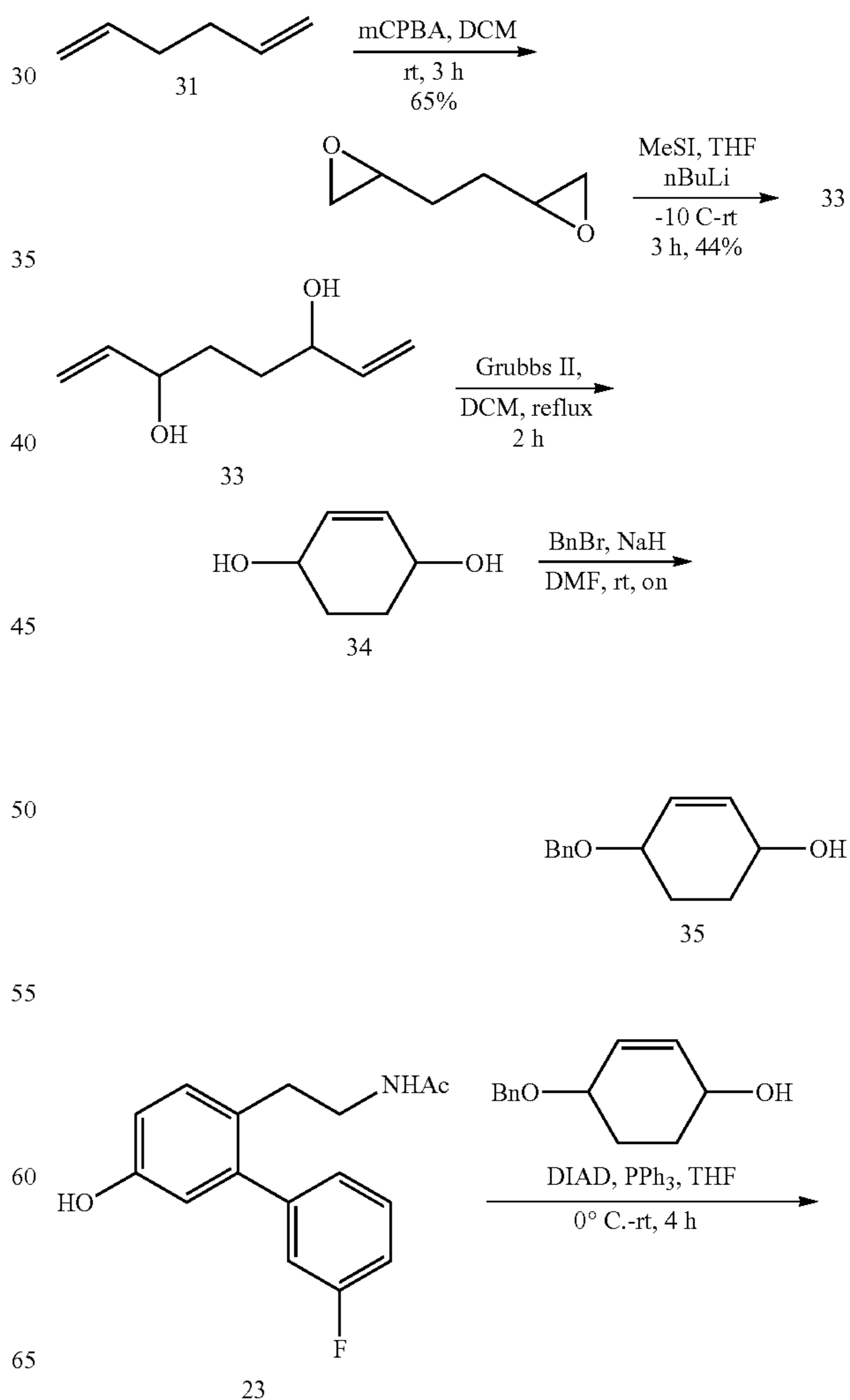
Scheme 7. Synthesis of carbocyclic sugar analogues 36 and 37.
