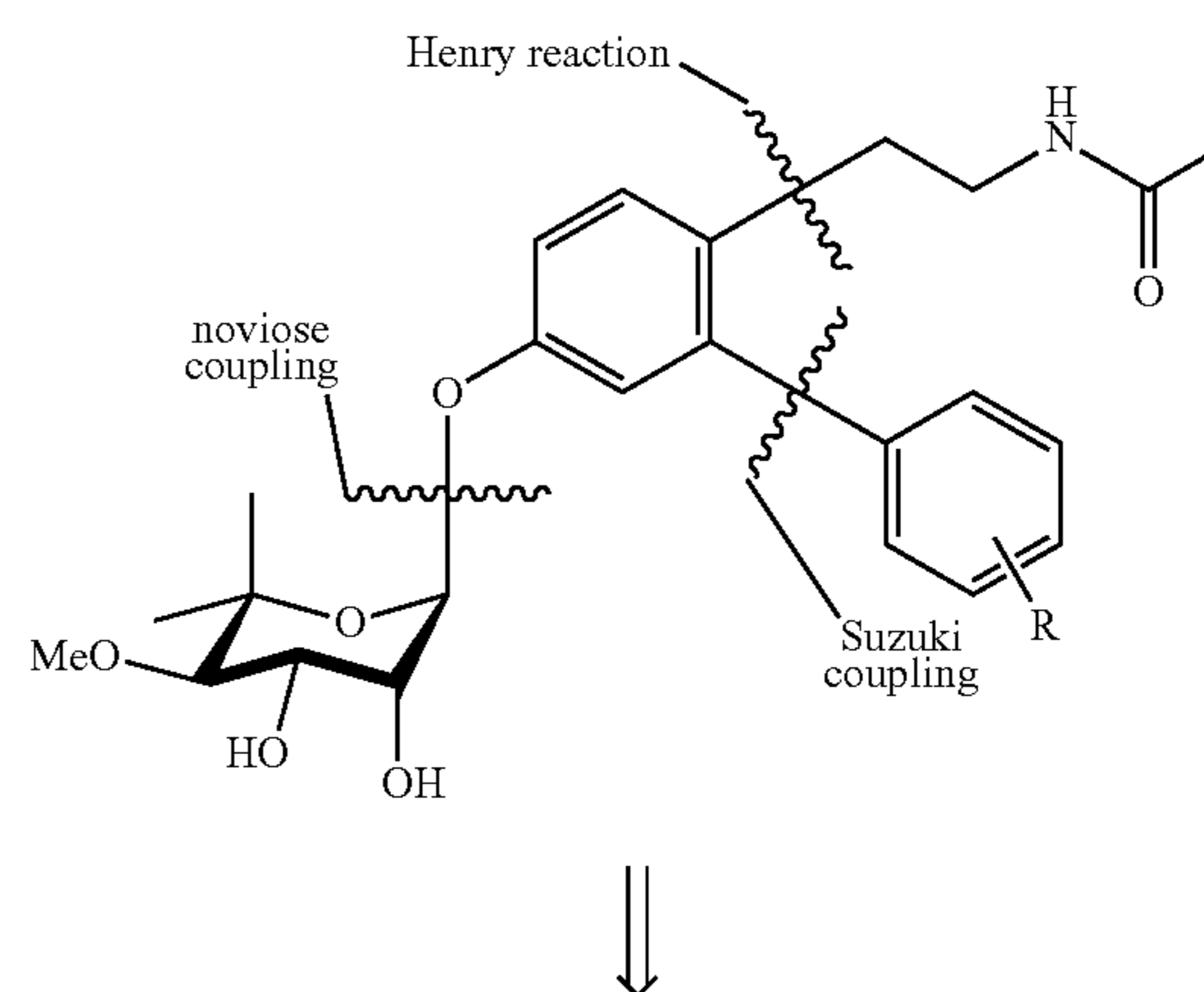
Scheme 1. Retrosynthetic analysis for the construction of novologue.
