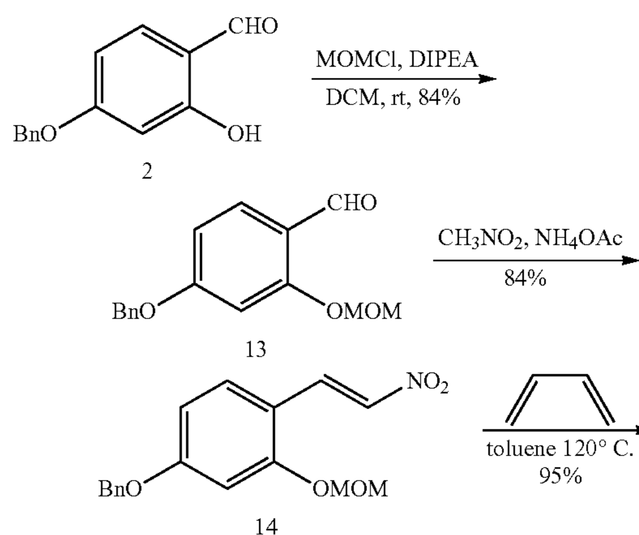
Scheme 4. Synthesis of cyclohexene containing novologues.
