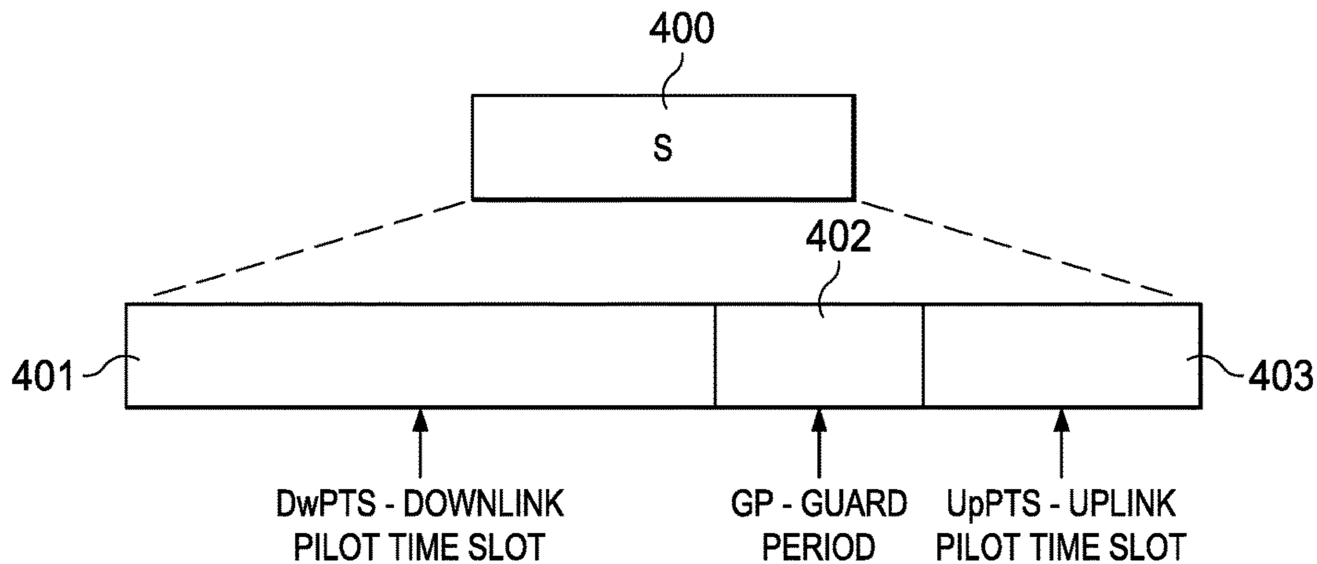
FIG. 4 (PRIOR ART)
