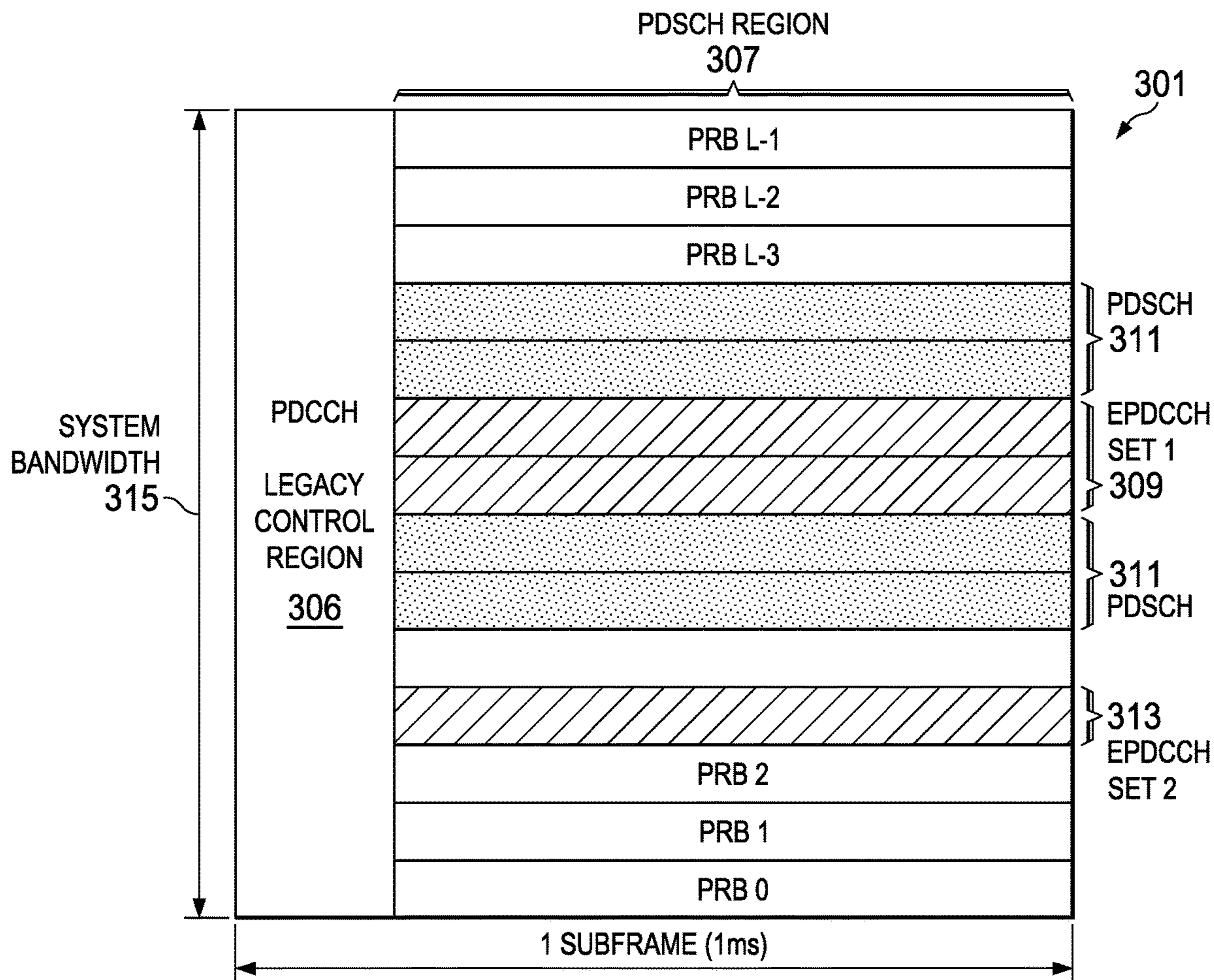
FIG. 3 (PRIOR ART)
