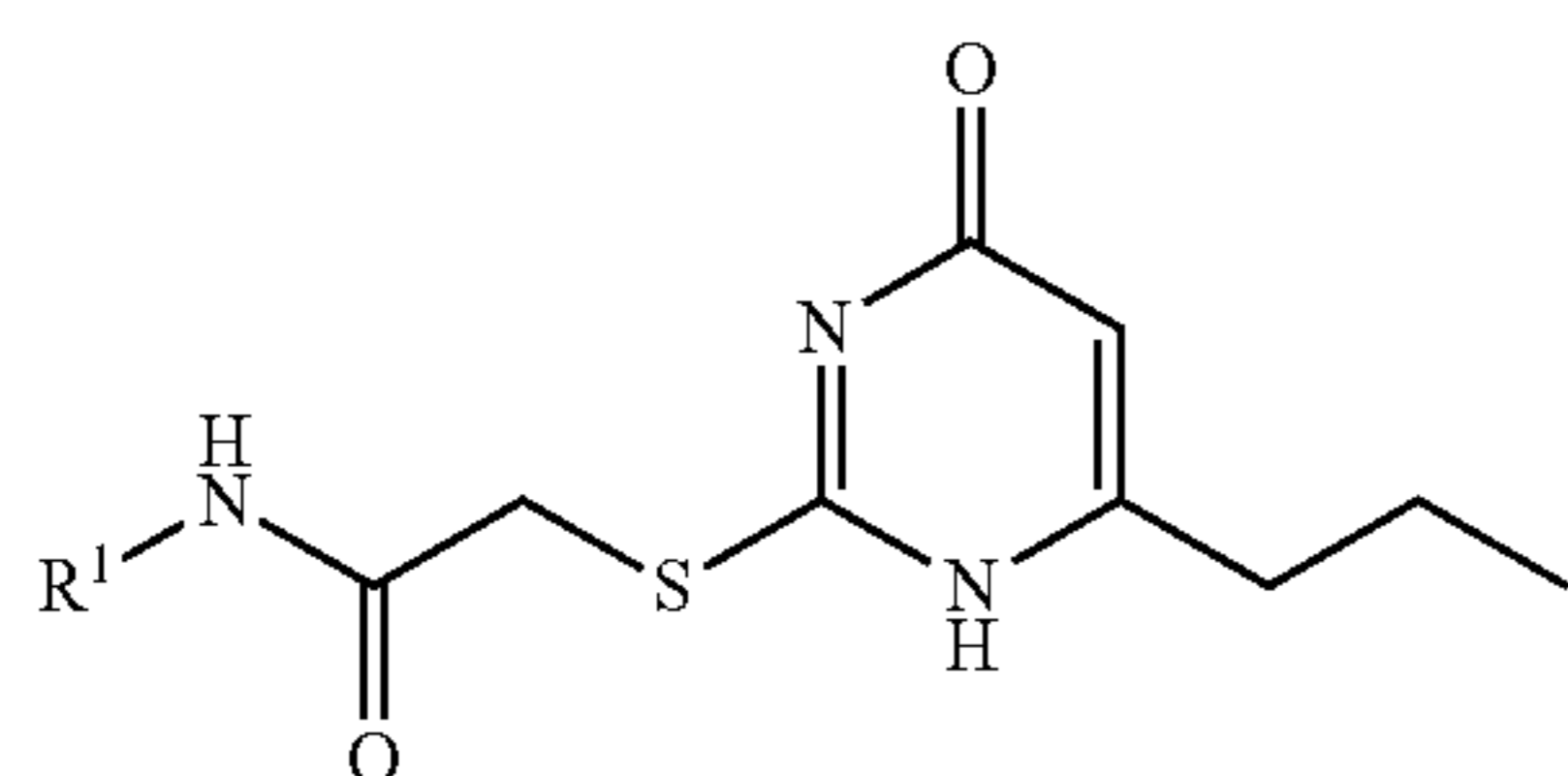
Reaction Scheme I. Synthesis of Inhibitors
