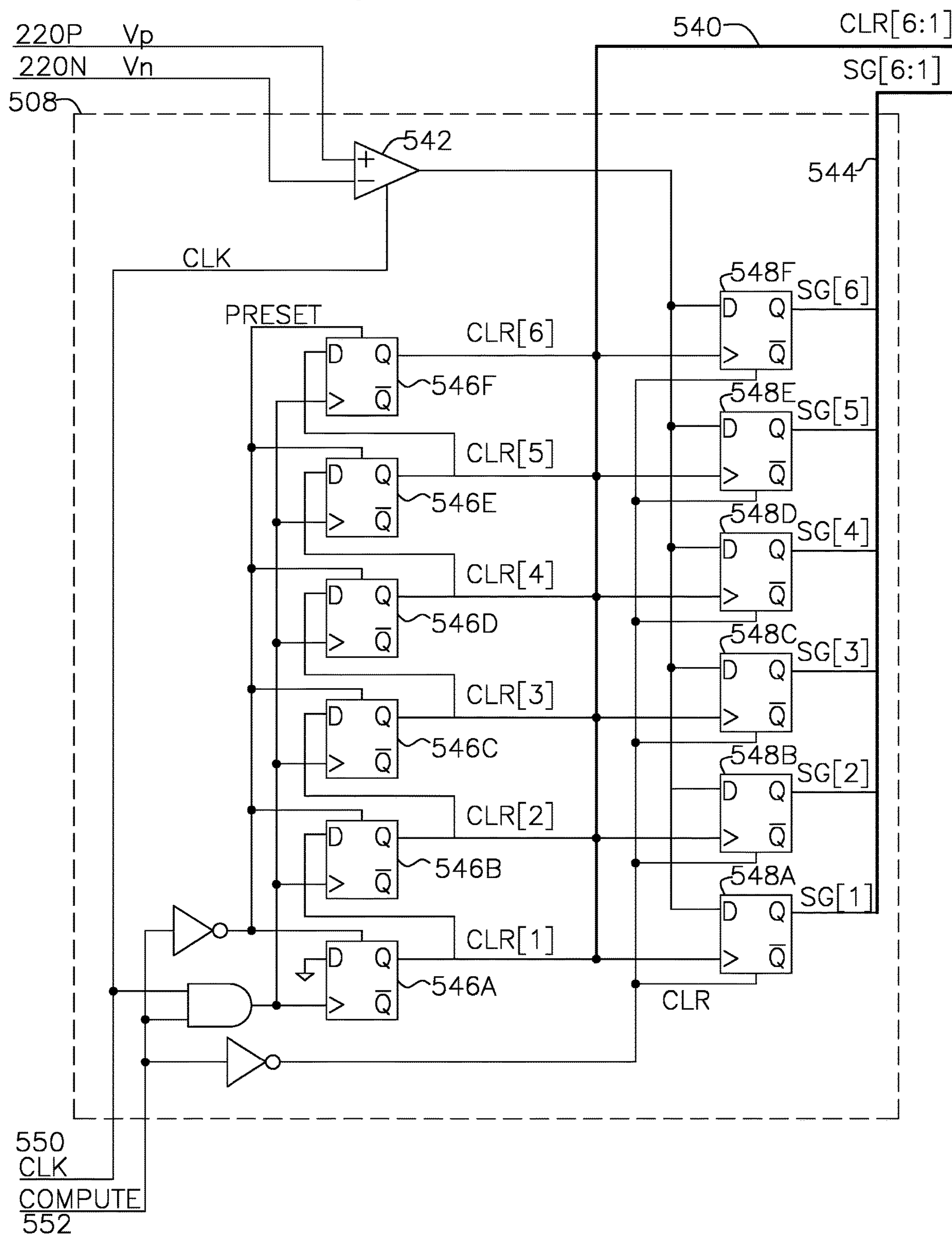
Figure 5B SAR Logic and Control with Relu
