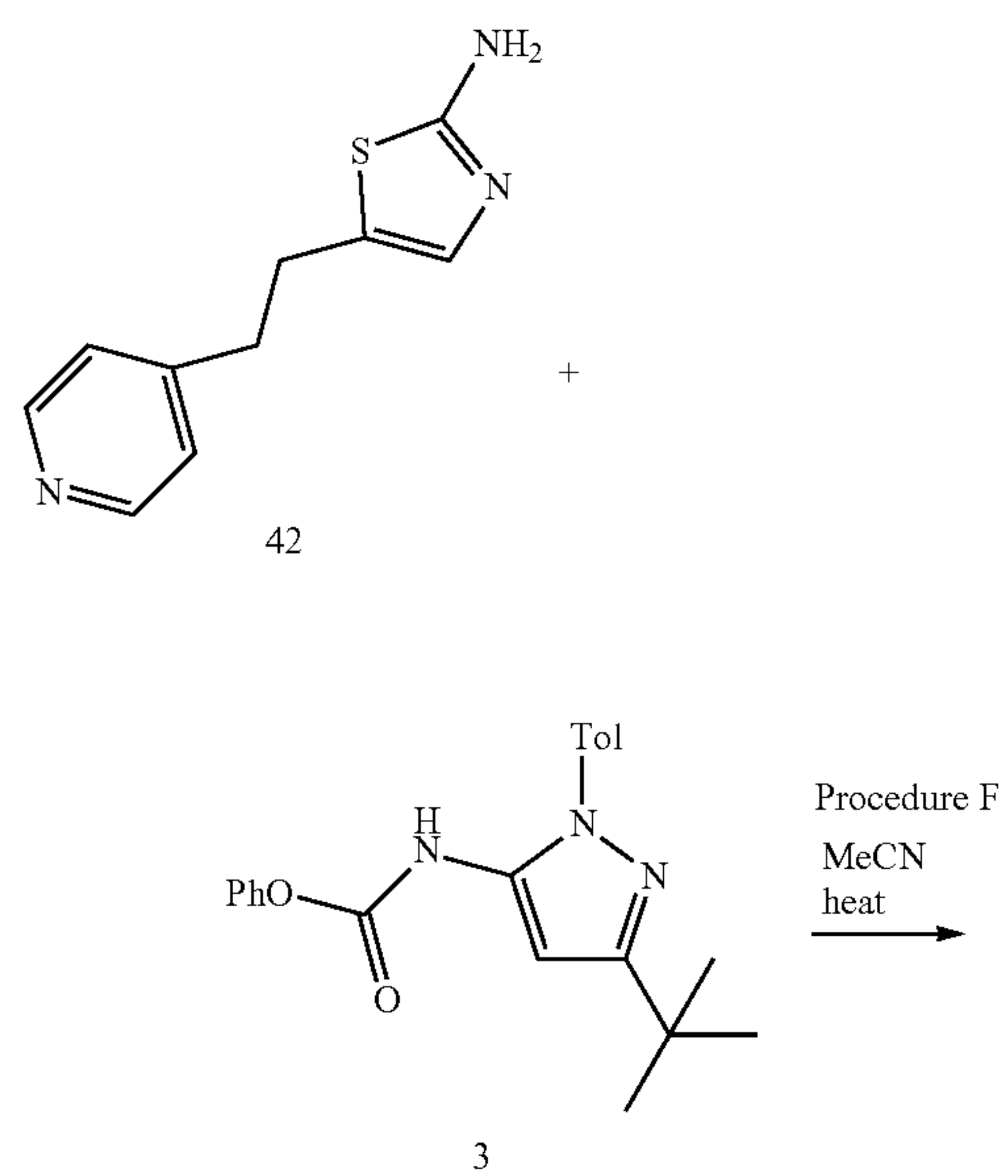
Scheme 9: Synthesis of Formula I Compounds
