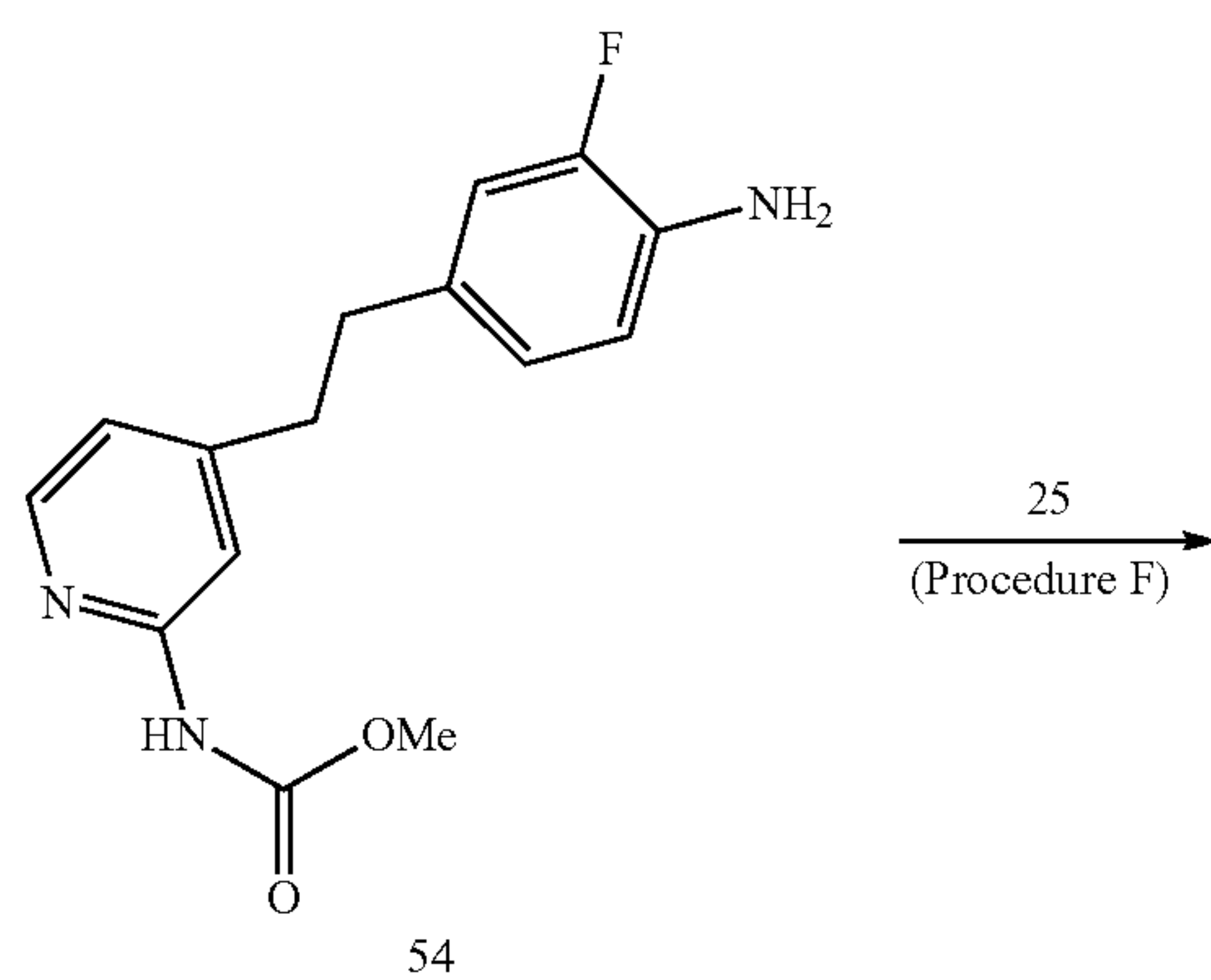
Scheme 10: Synthesis of Formula II Compounds
