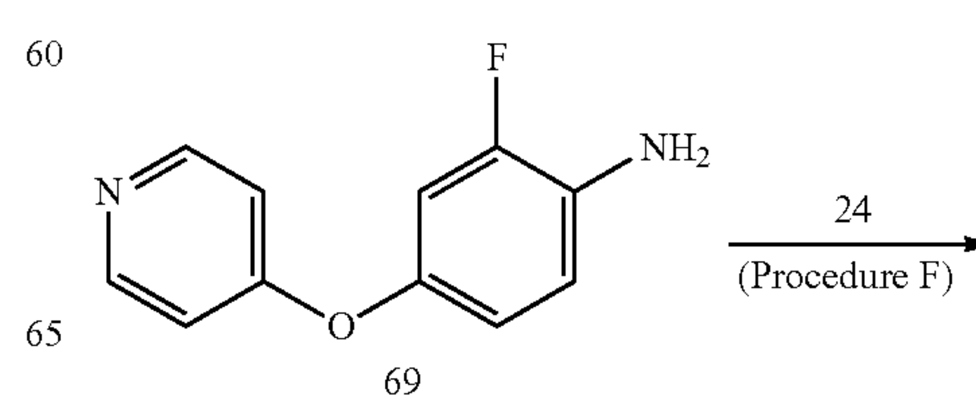
Scheme 11. Synthesis of Formula III Compounds
