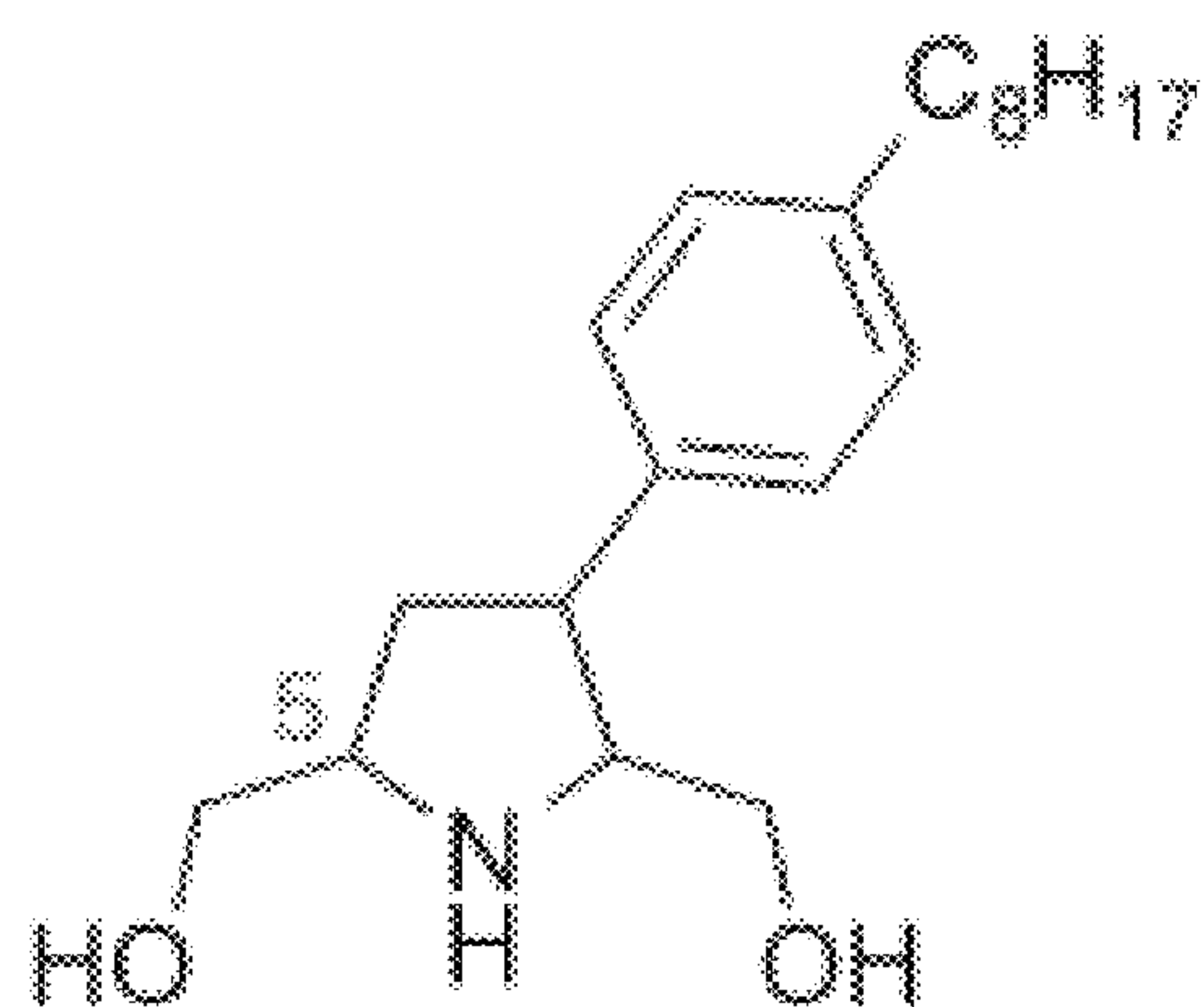
Generic constrained C-aryl analogue A
