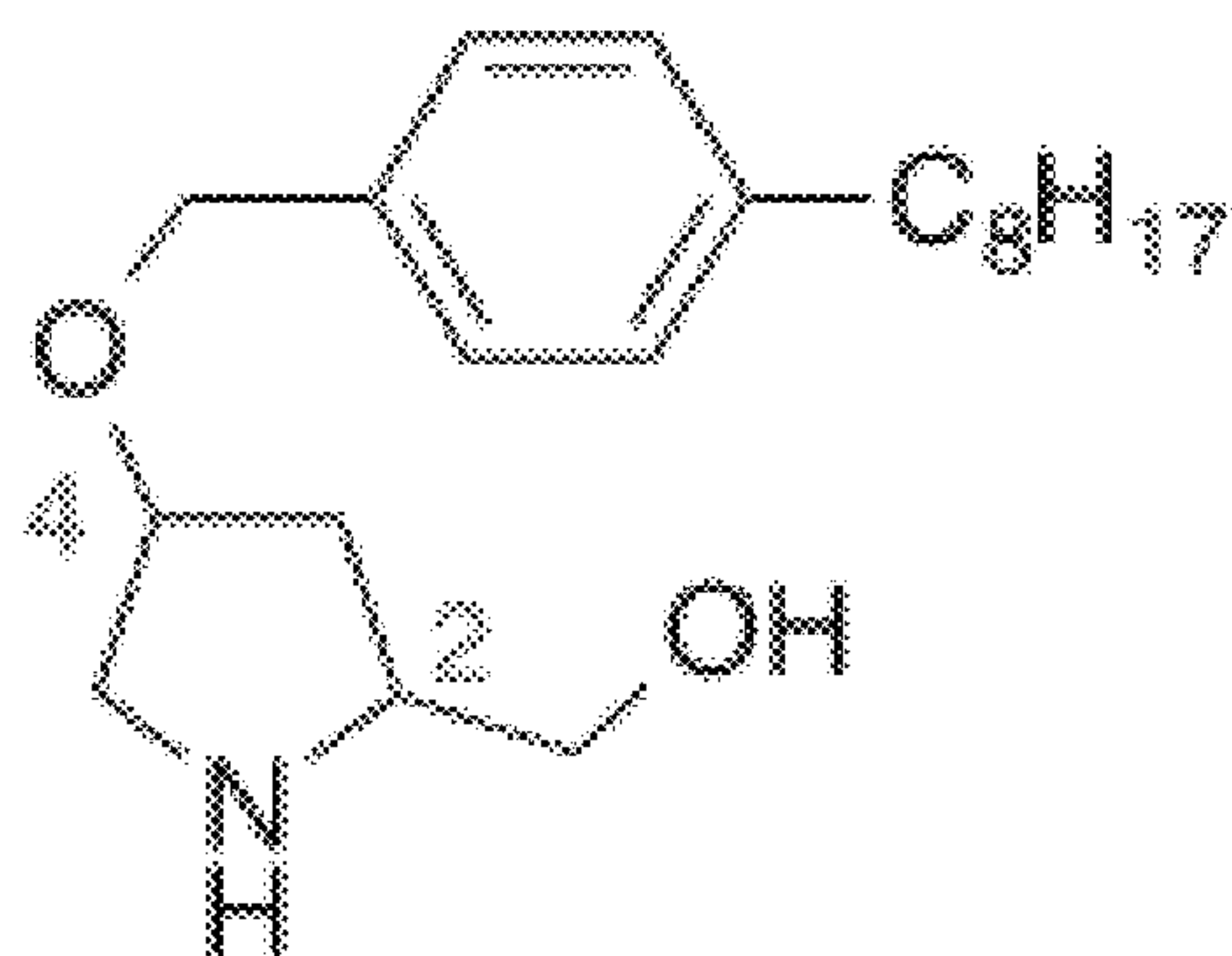
Antileukemic O-arylmethyl (2 R , 4 S ) and (2 S , 4 R ) pyrrolidine analogues B
