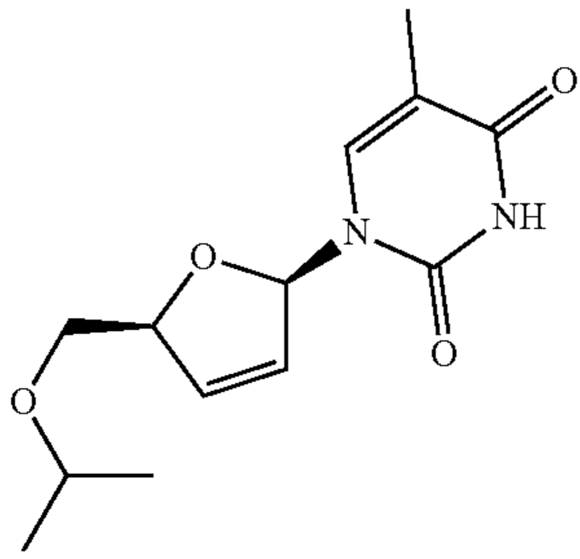
O-isopropyl-d4T.
