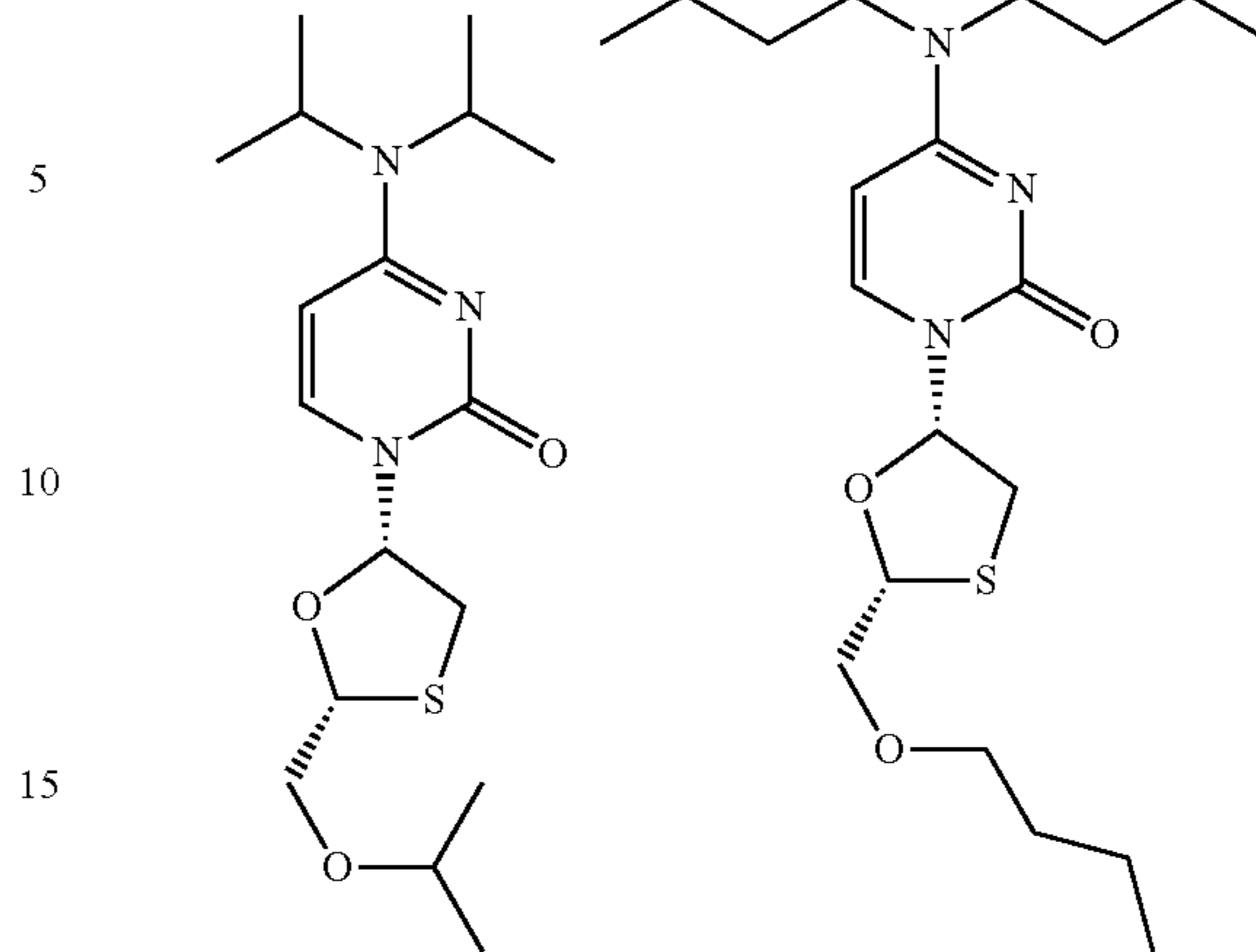
3-Isopropyl-3TC
