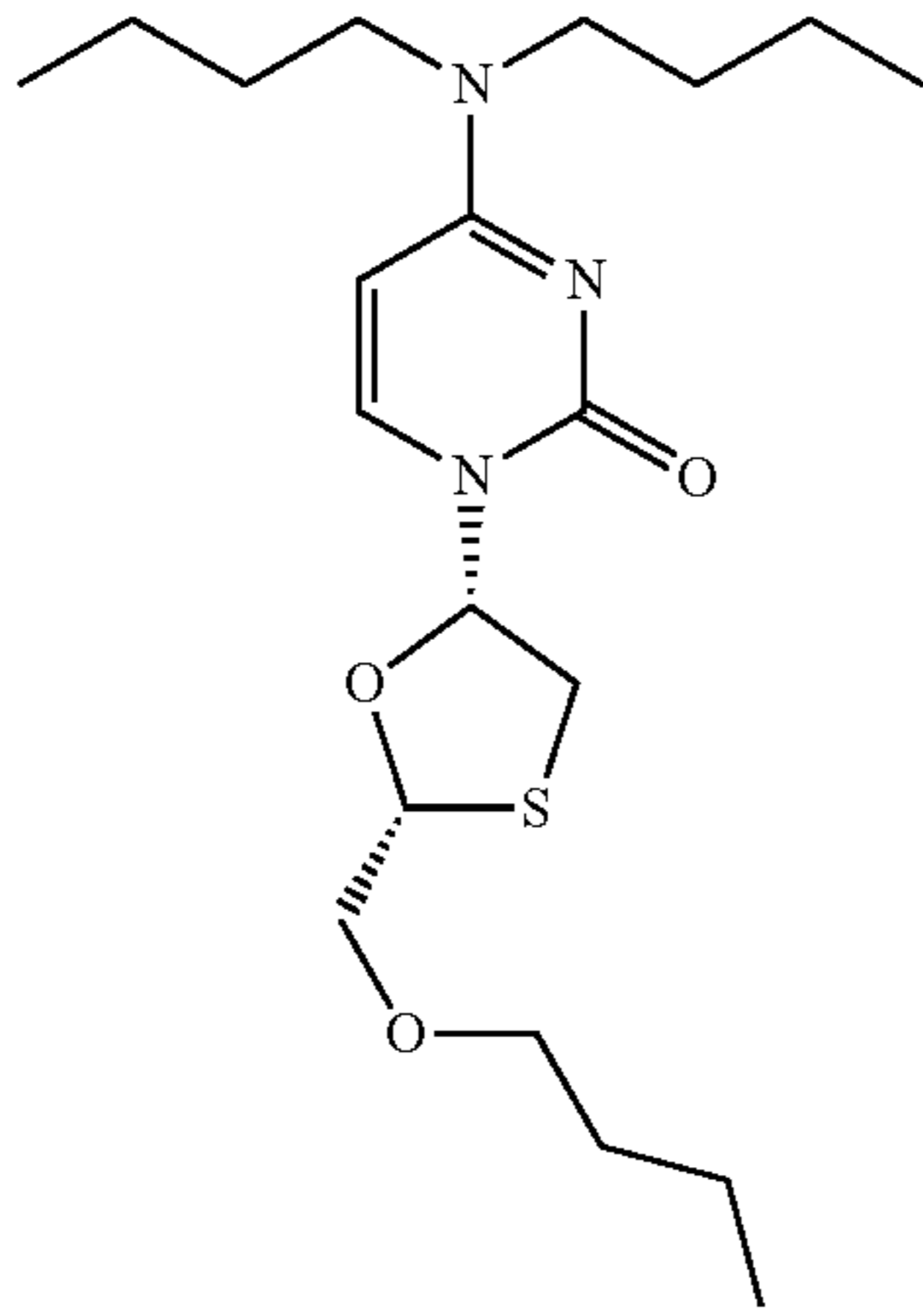
3-Butyl-3TC,
