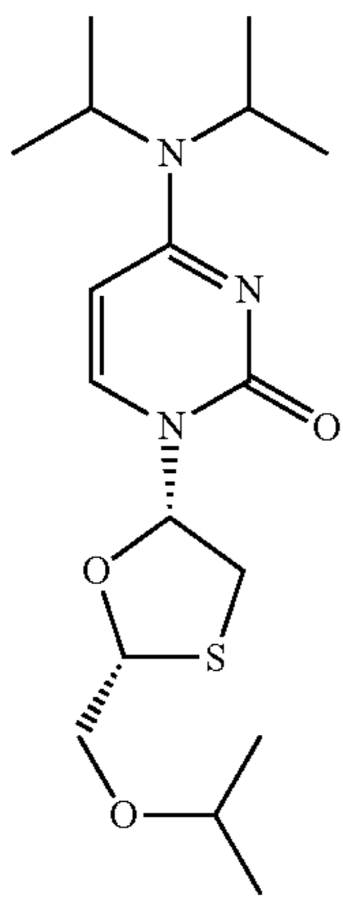
3-Isopropyl-3TC,
