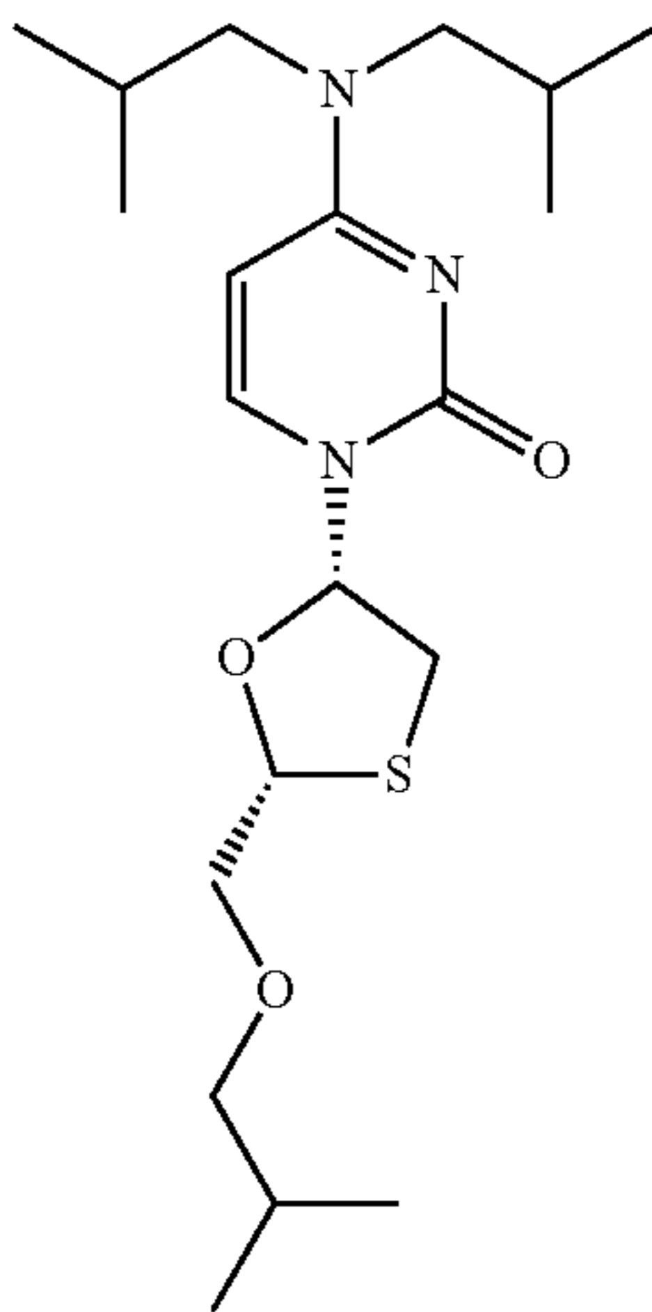
3-Isobutyl-3TC,
