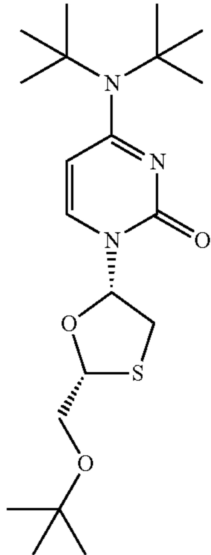
3-Tert-butyl-3TC,
