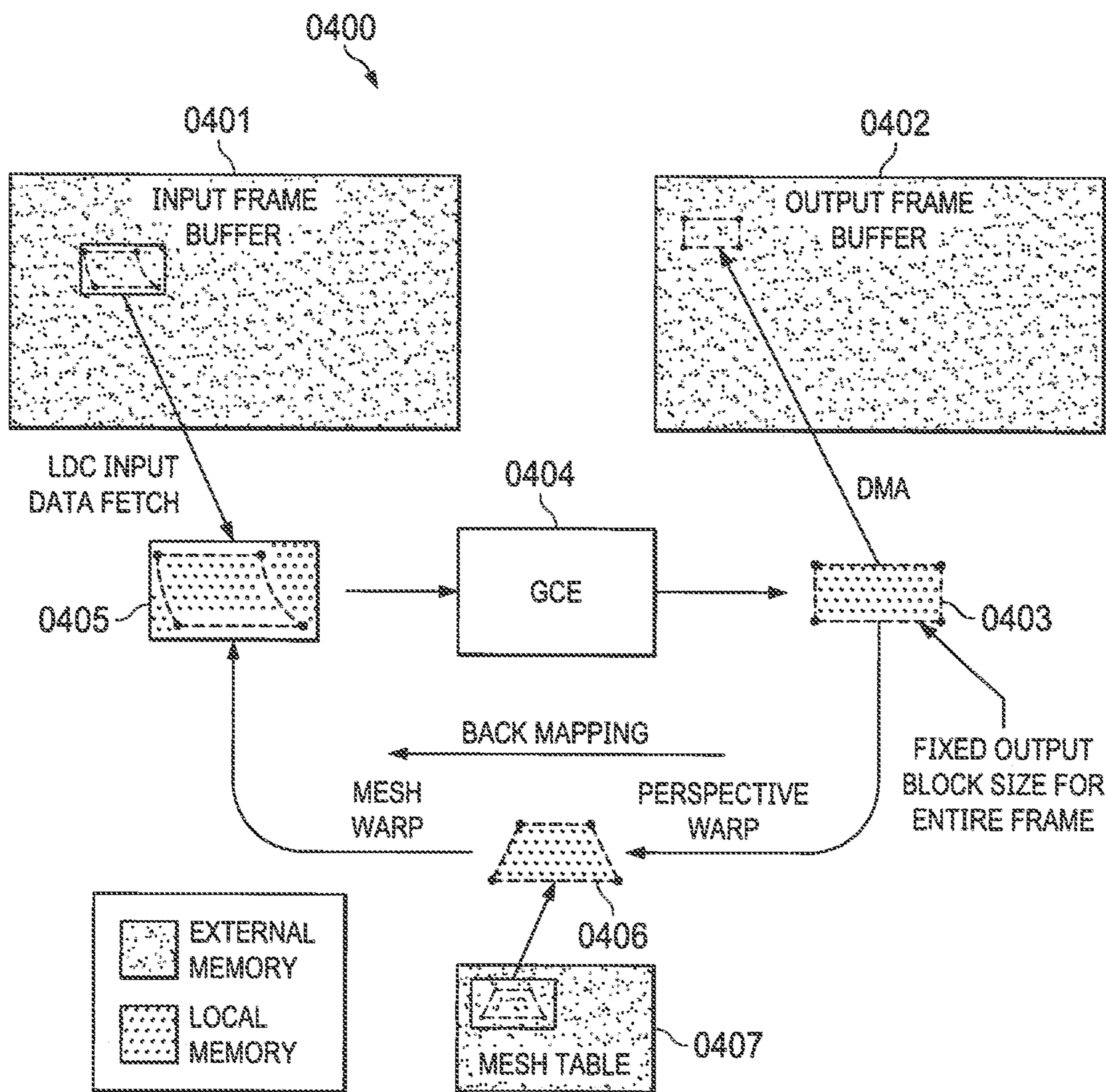
FIG. 4 (PRIOR ART)
