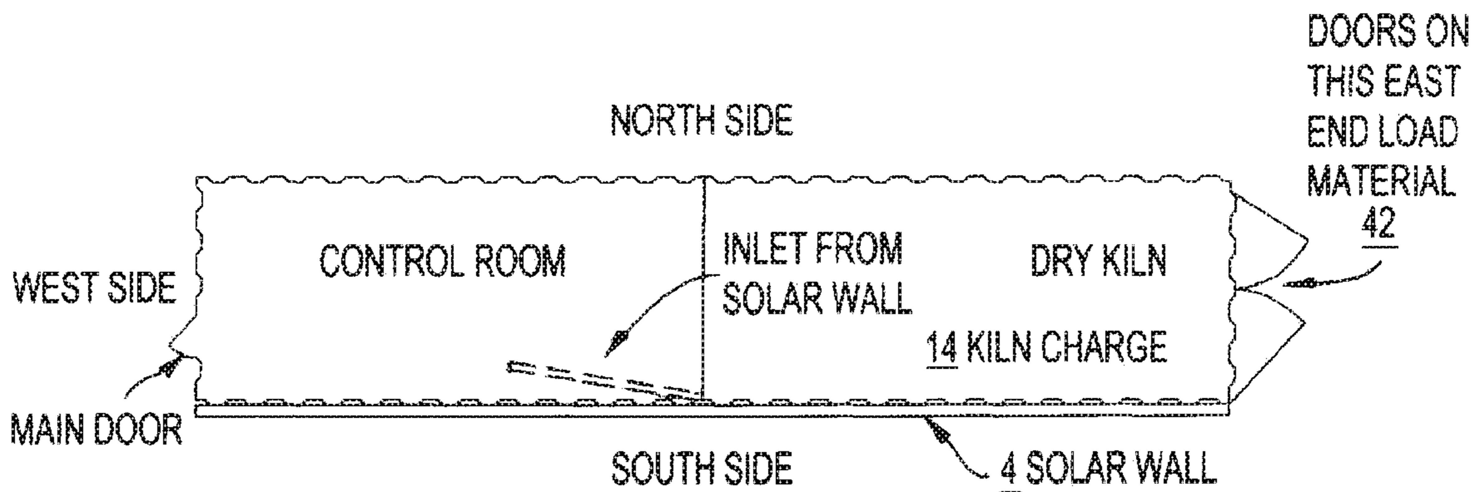
FIG. 2 SOLAR HYBRID KILN DESIGN (TOP VIEW)
