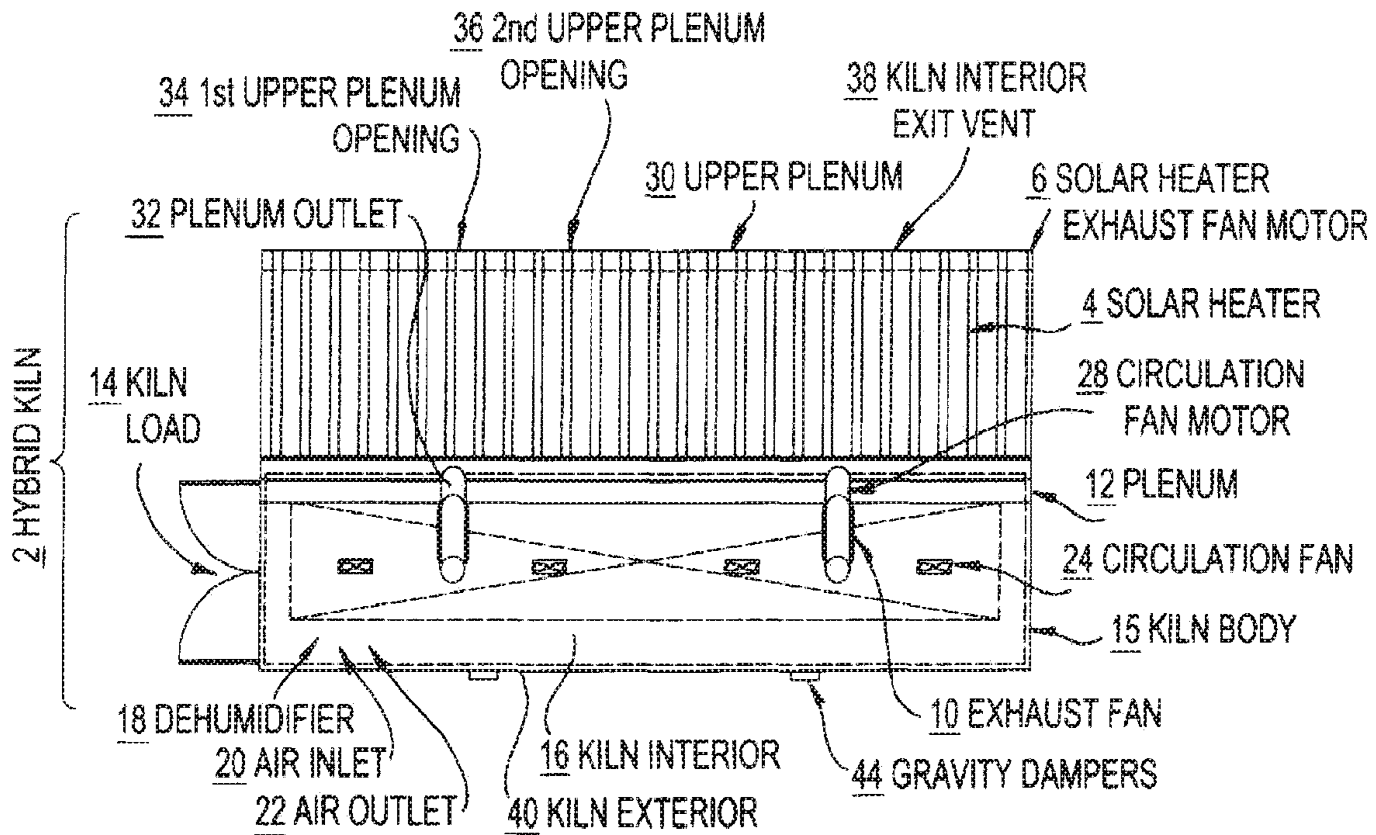
FIG. 1 HYBRID KILN (SIDE VIEW ELEVATION)
