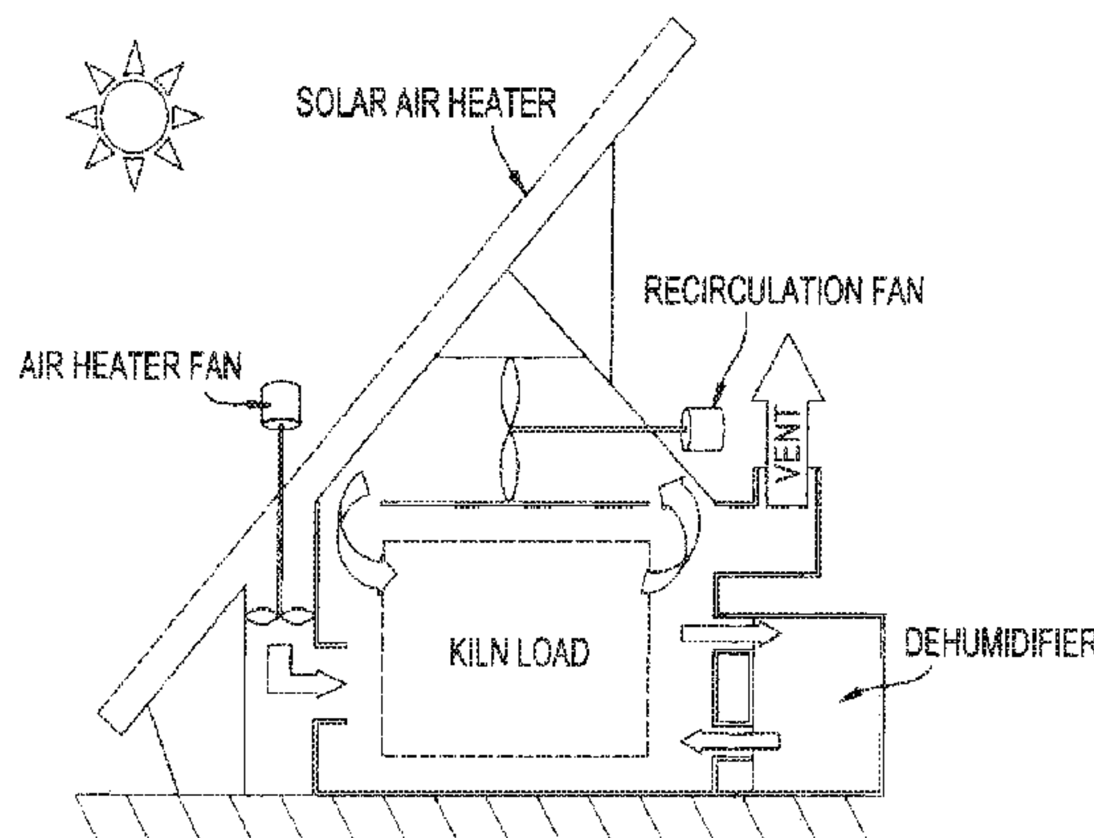
SCHEMATIC OF THE HYBRID SOLAR KILN
