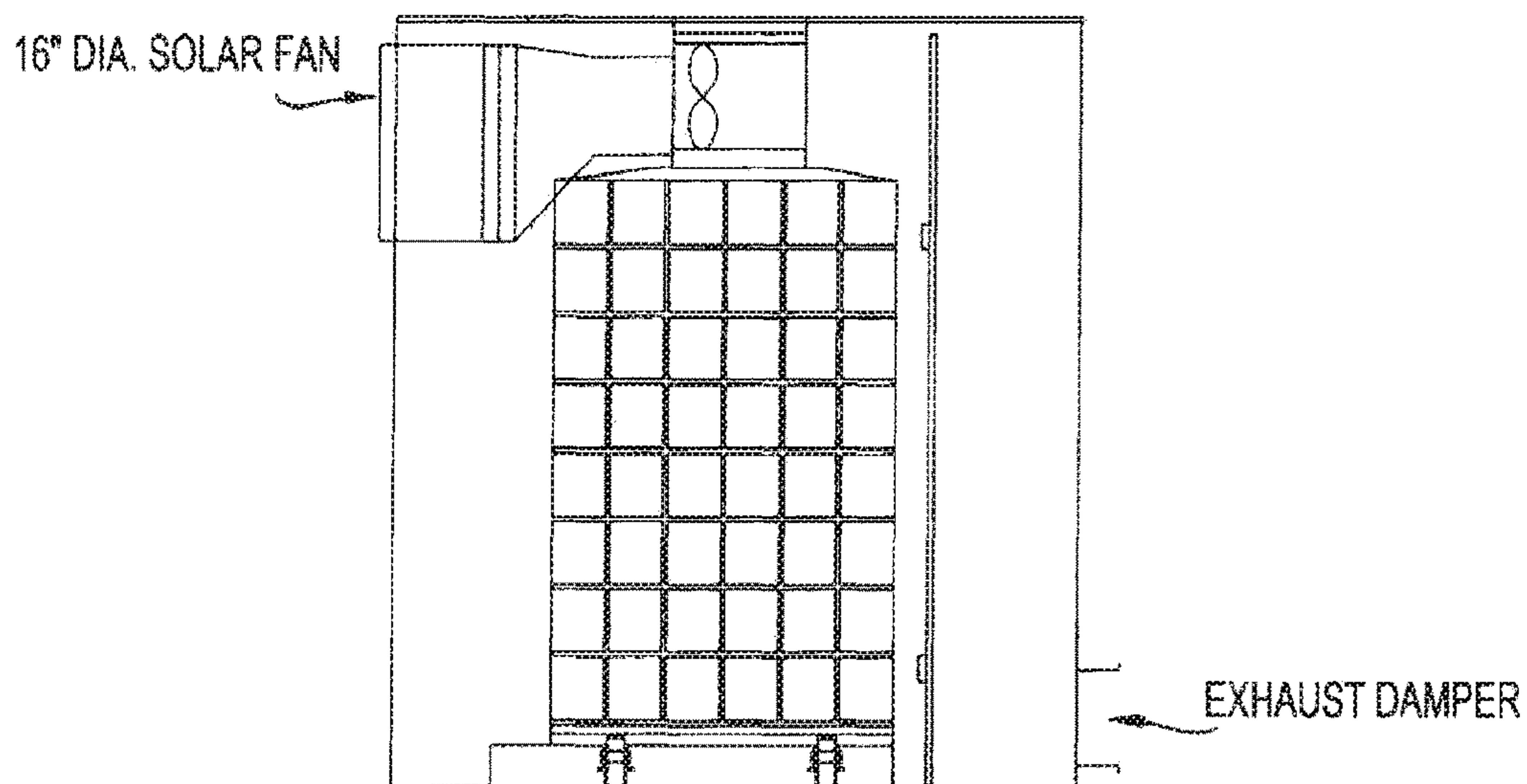
FIG. 3 HYBRID KILN (SIDE ELEVATION)
