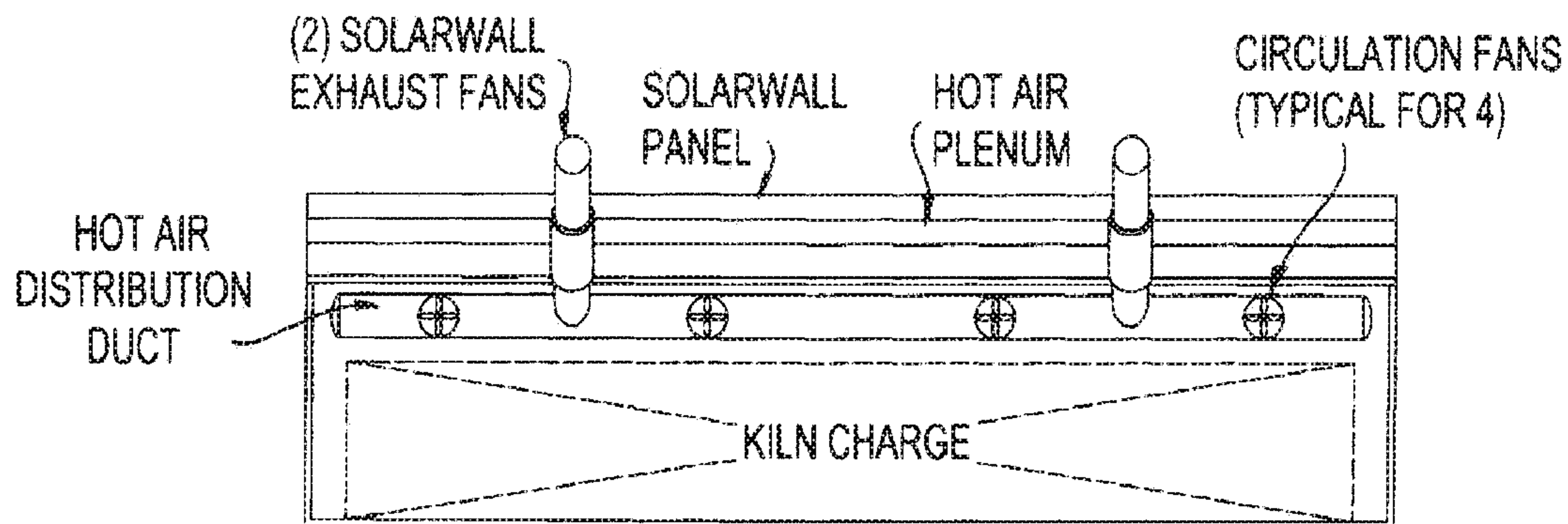
SOLAR WALL TIMBER DRYER BUILT FROM SINGLE 40 FT. SHIPPING CONTAINER
