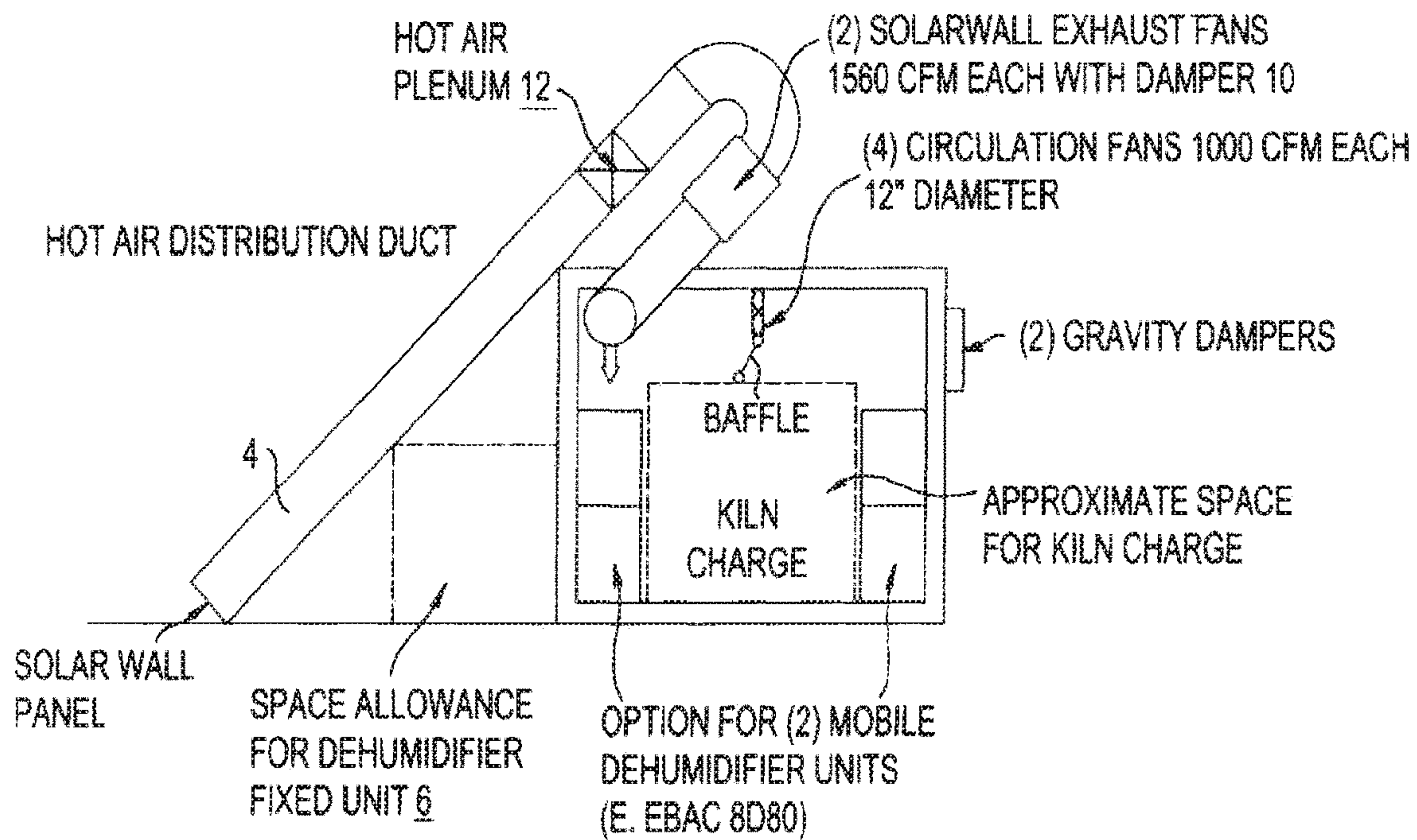
FIG. 4 HYBRID KILN (FRONT ELEVATION)
