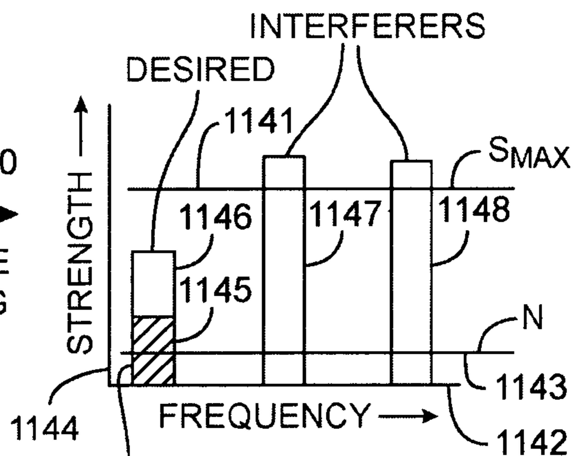
FIG. 11C INTERMOD PRODUCTS
