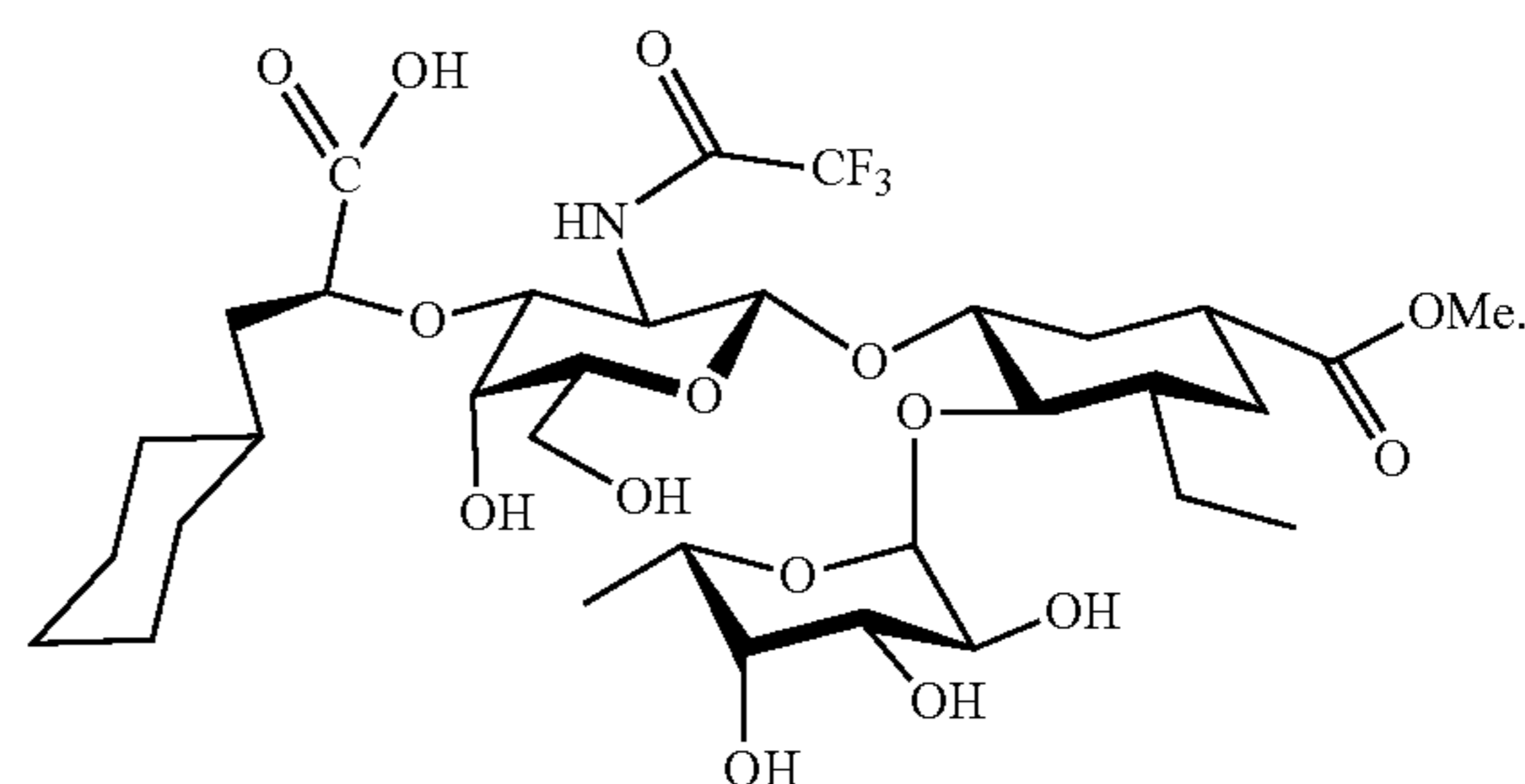
Compound 27
