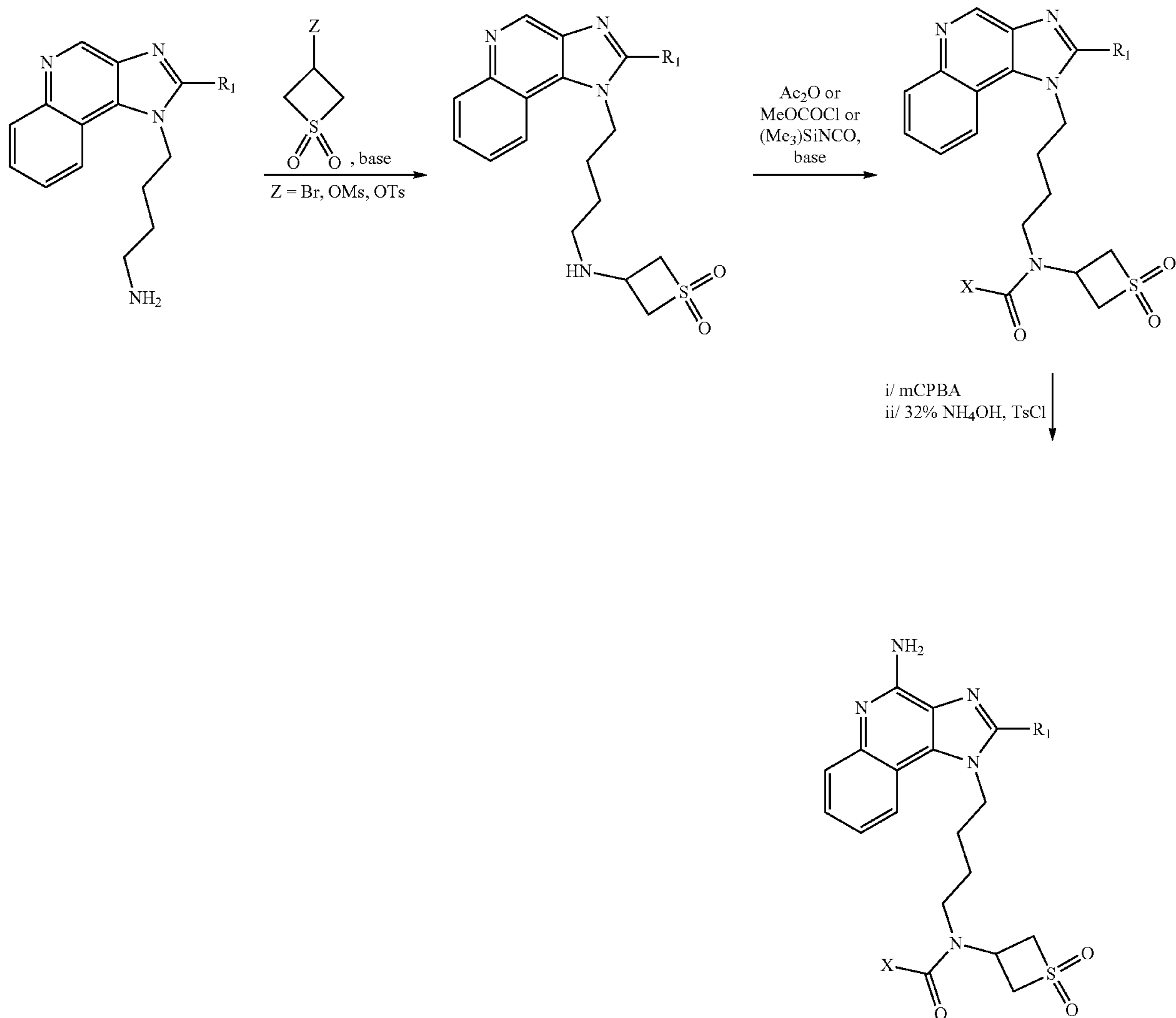
Scheme 8: synthesis of Example 7-11
