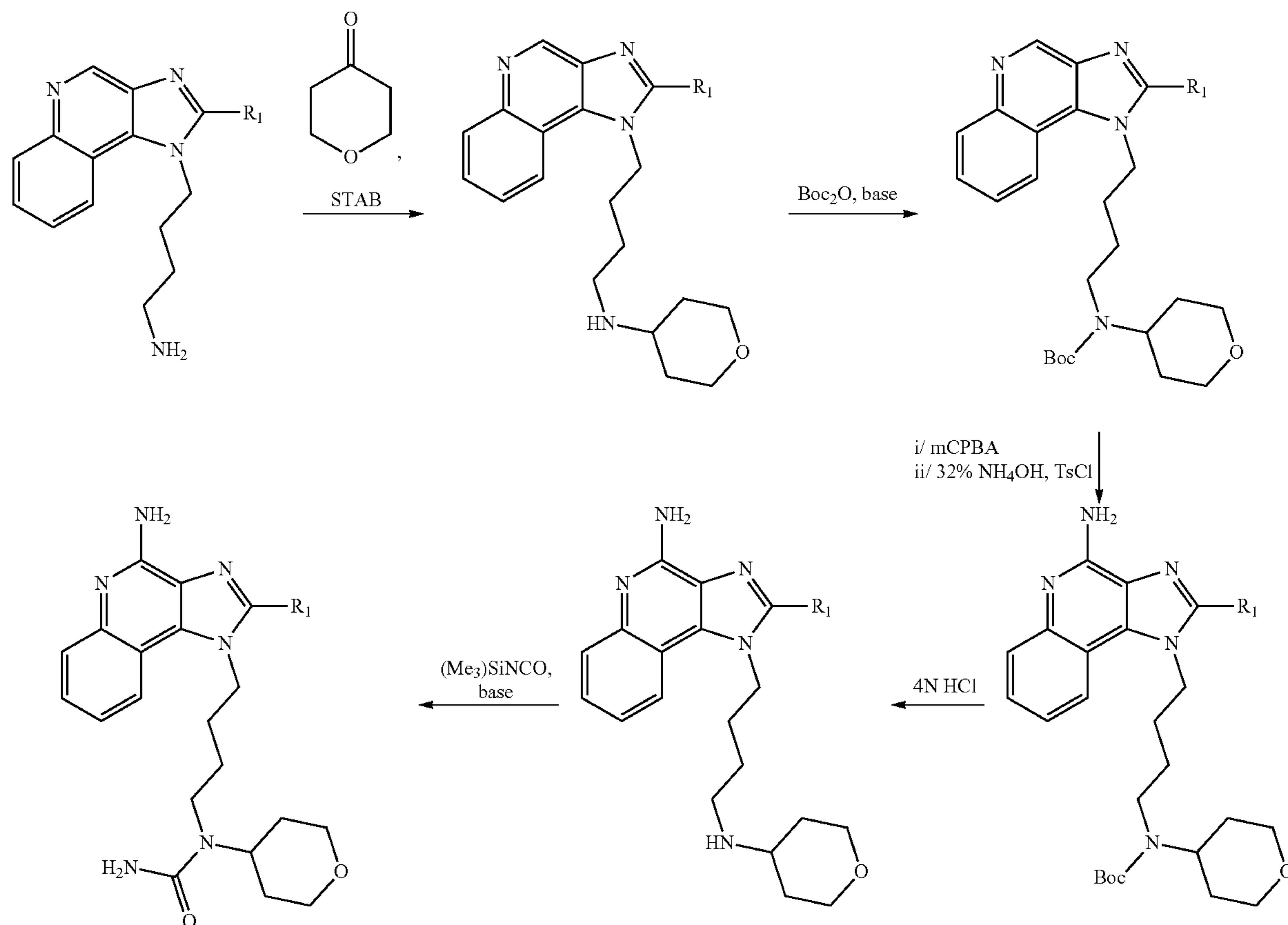
Scheme 5: synthesis of Example 2 and 4 (for illustrative purposes)
