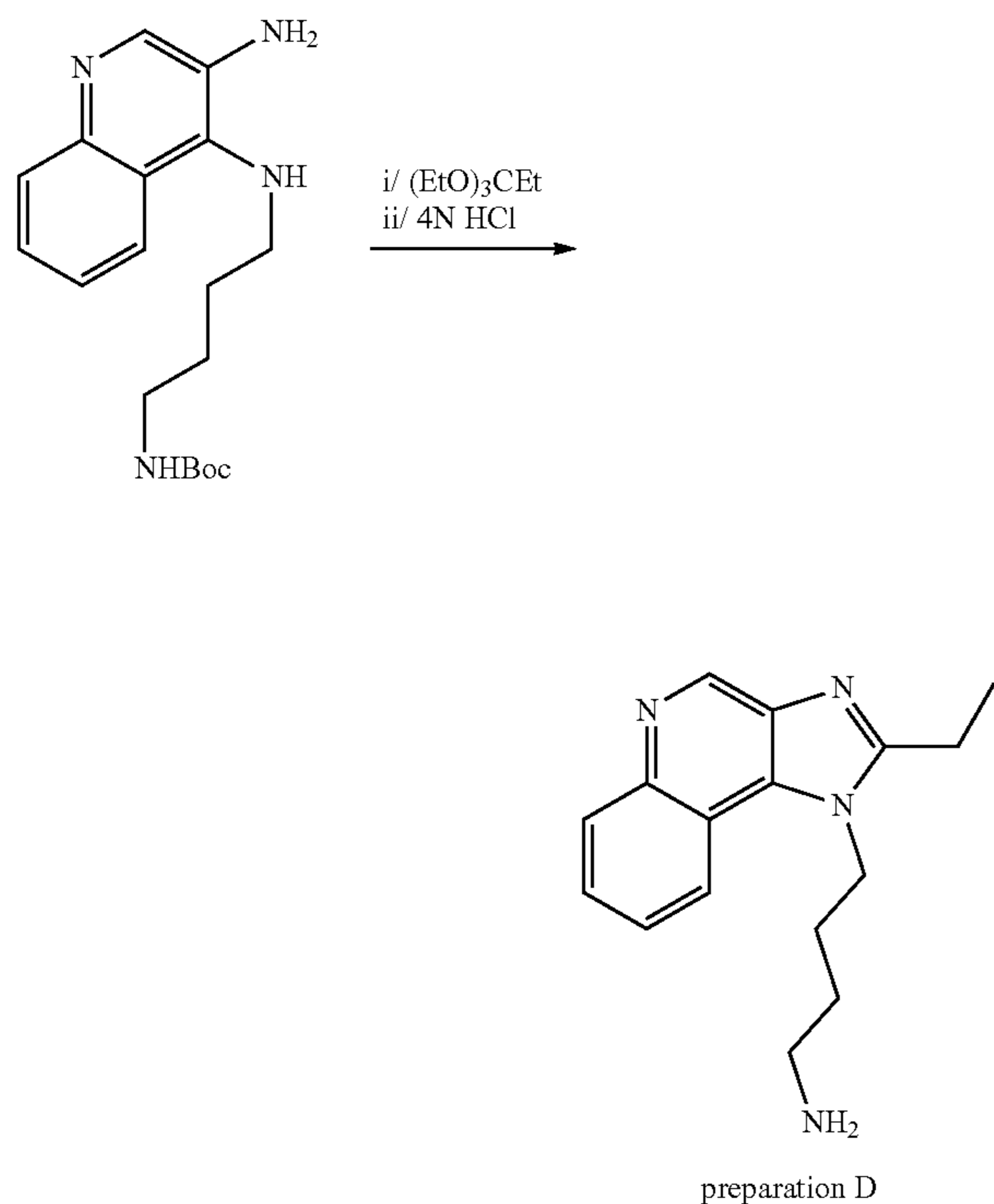
Scheme 2: synthesis of preparation D
