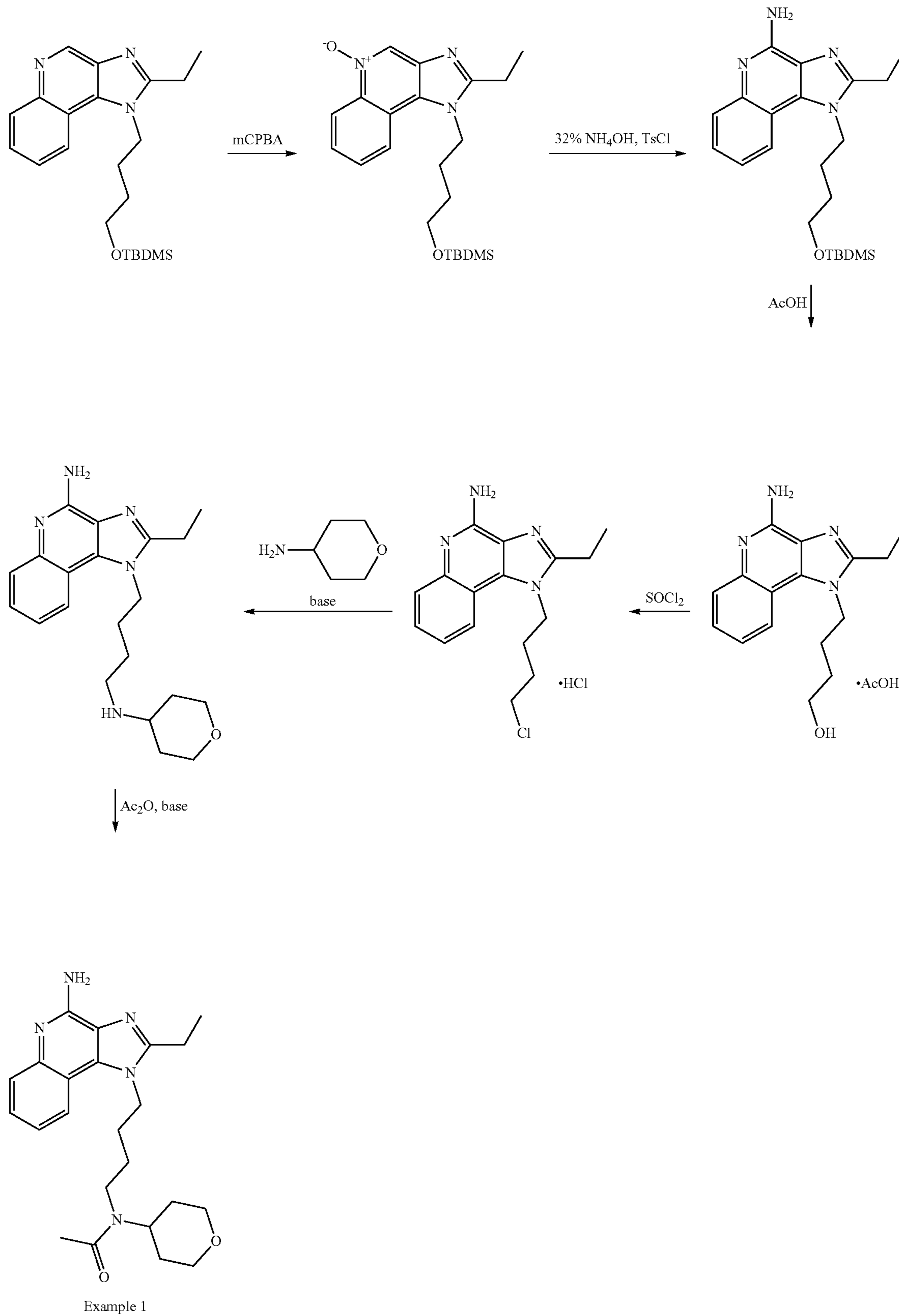
Scheme 4. synthesis of Example 1 (for illustrative purposes)
