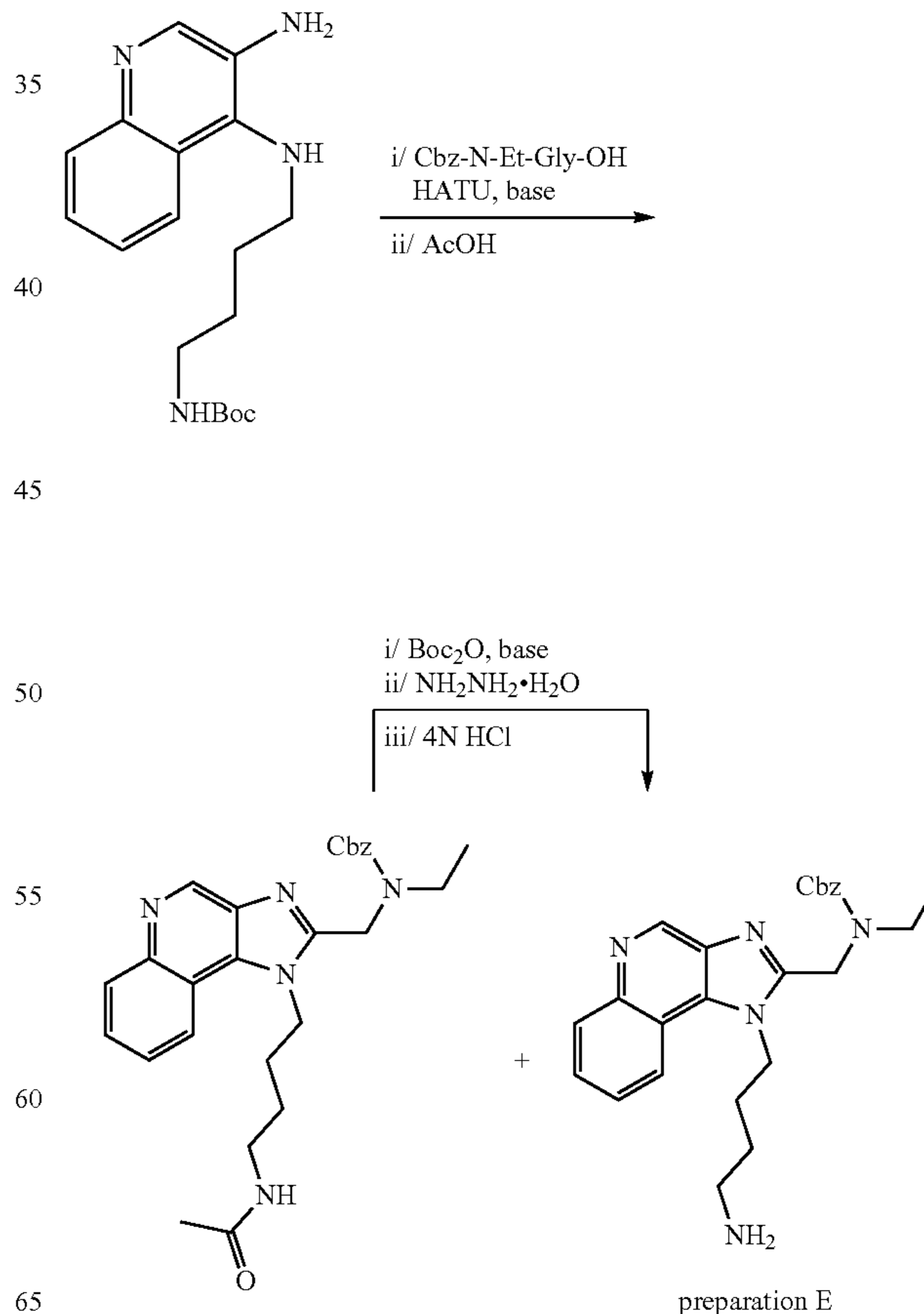
Scheme 3: synthesis of preparation E
