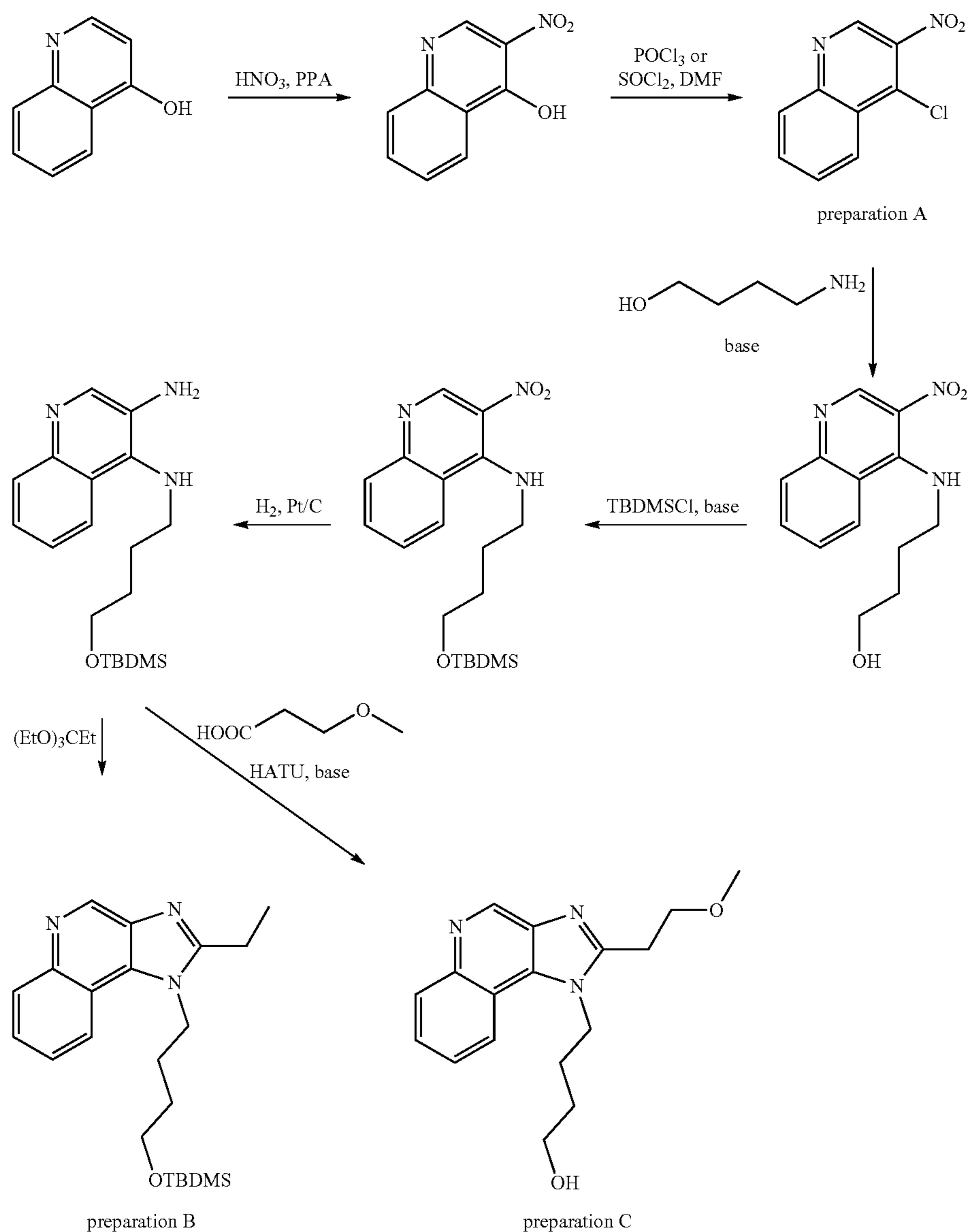
Scheme 1: synthesis of preparation A-C
