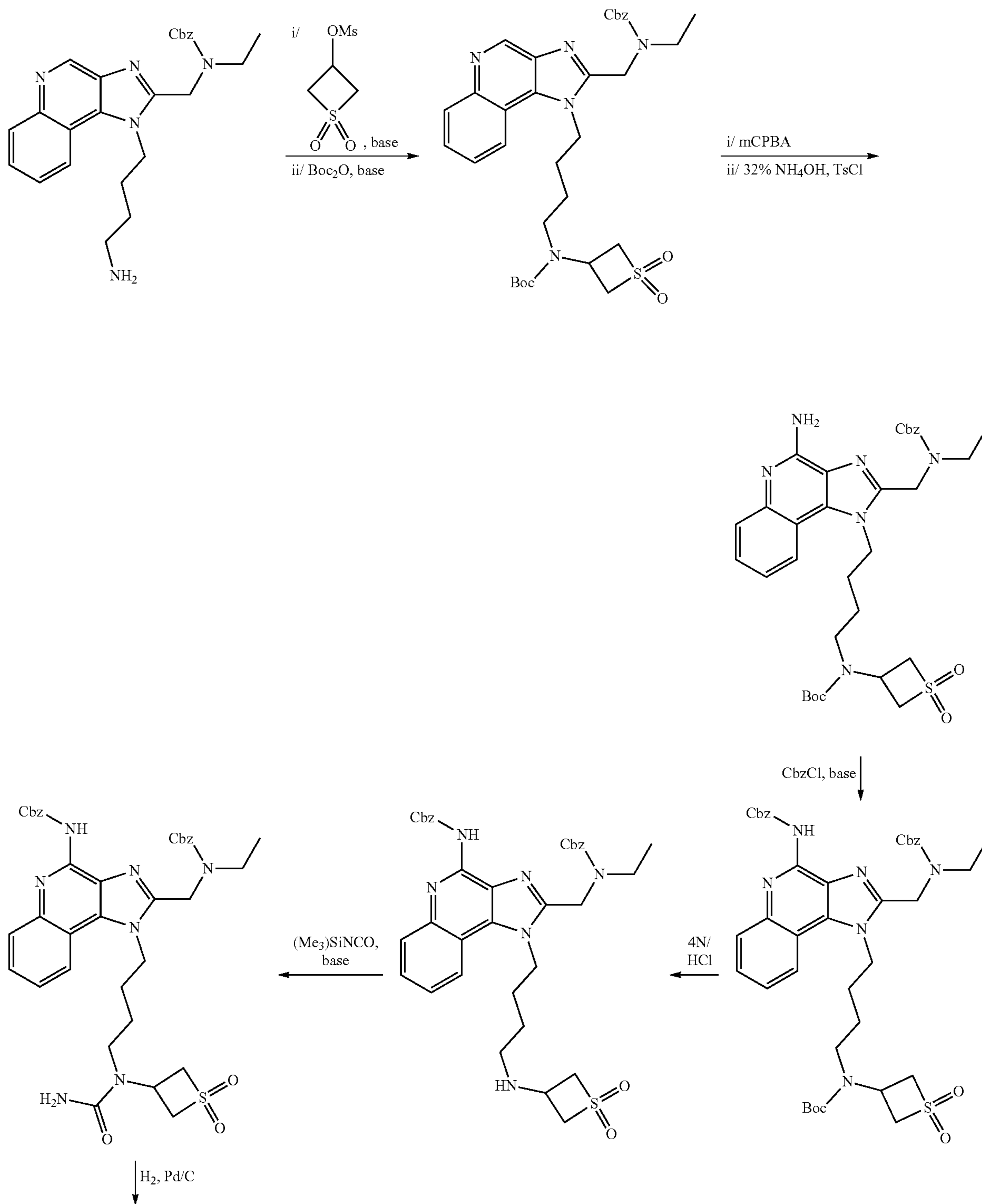
Scheme 9: synthesis of Example 12
