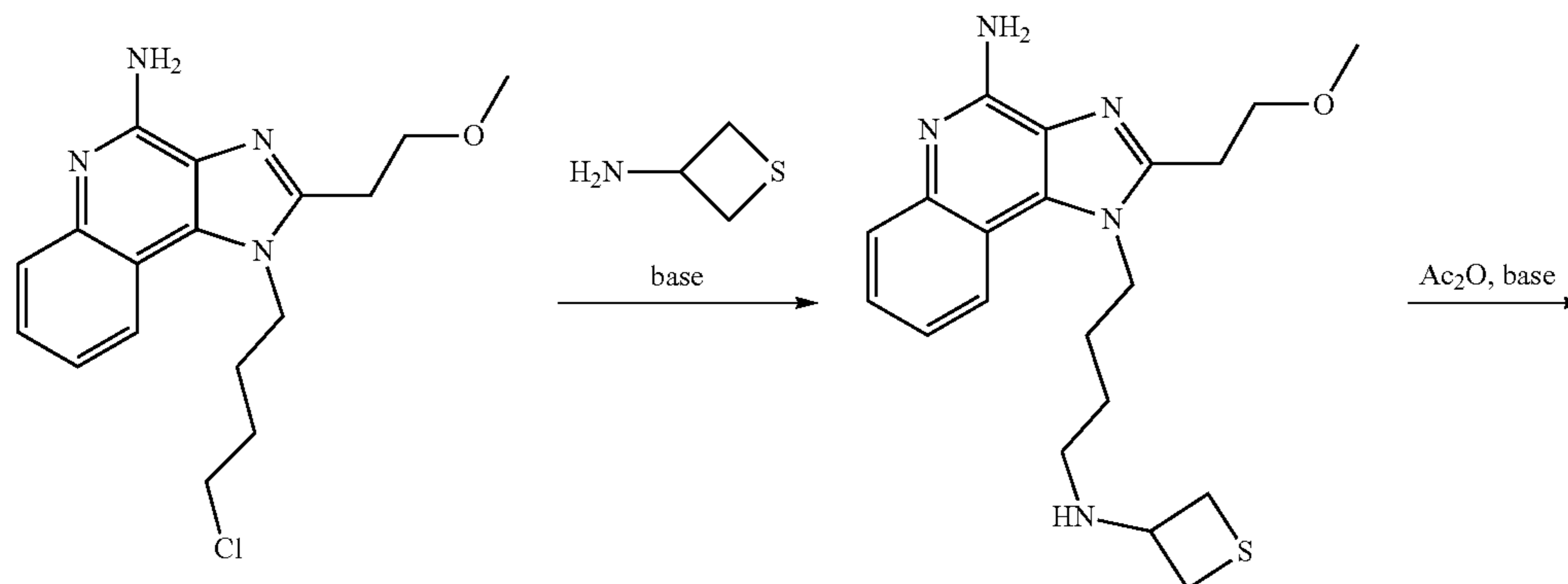
Scheme 10: synthesis of Example 13-15
