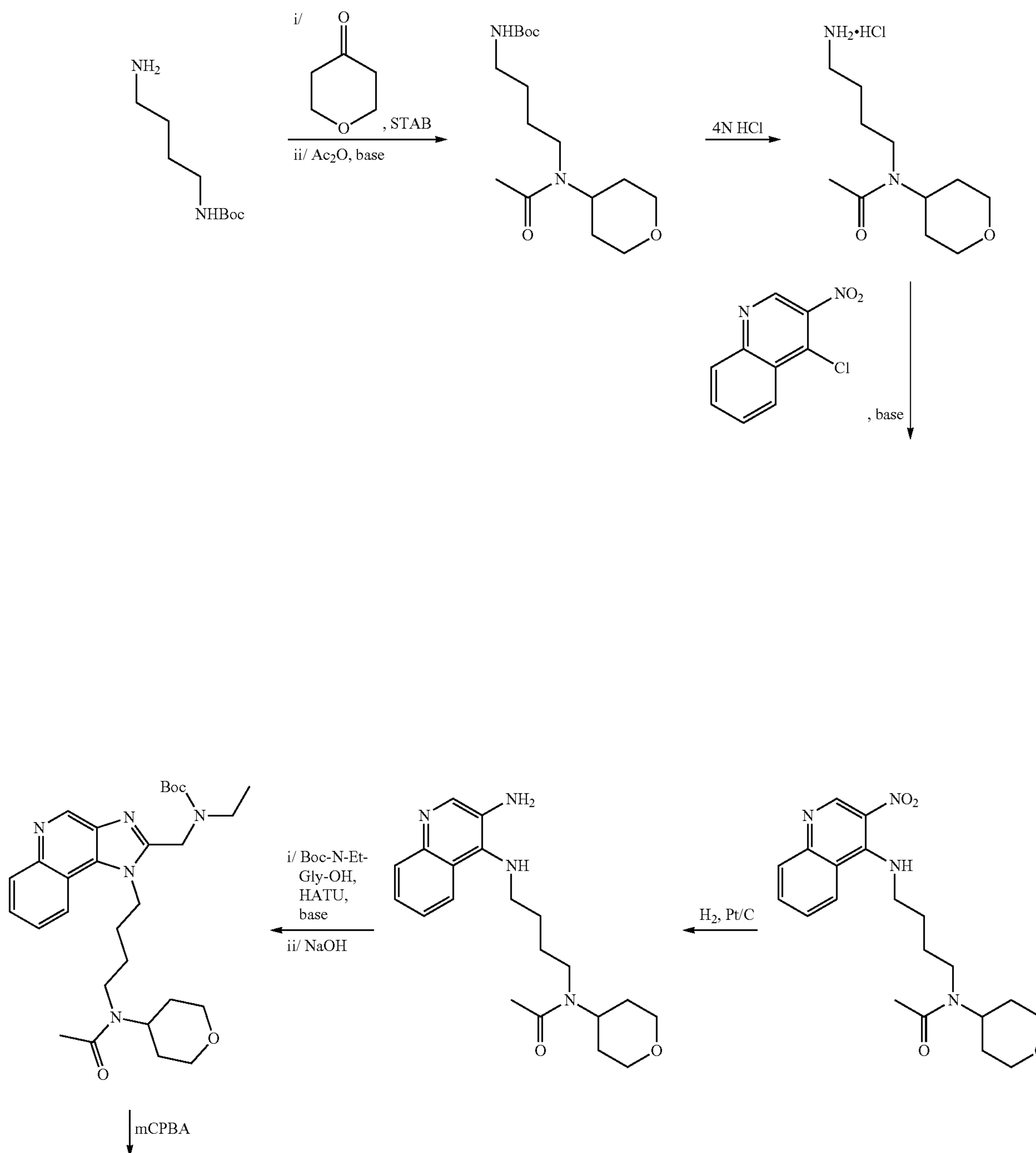
Scheme 6: synthesis of Example 3 (for illustrative purposes)
