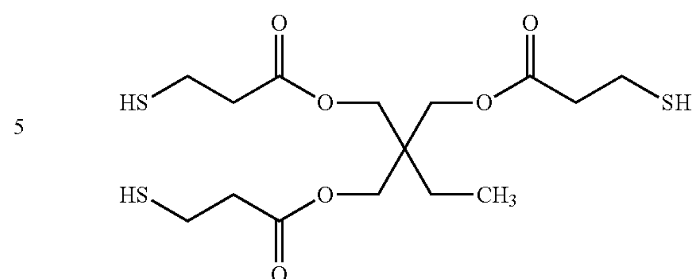
Trimethylolpropane tris(3-mercaptopropionate)
