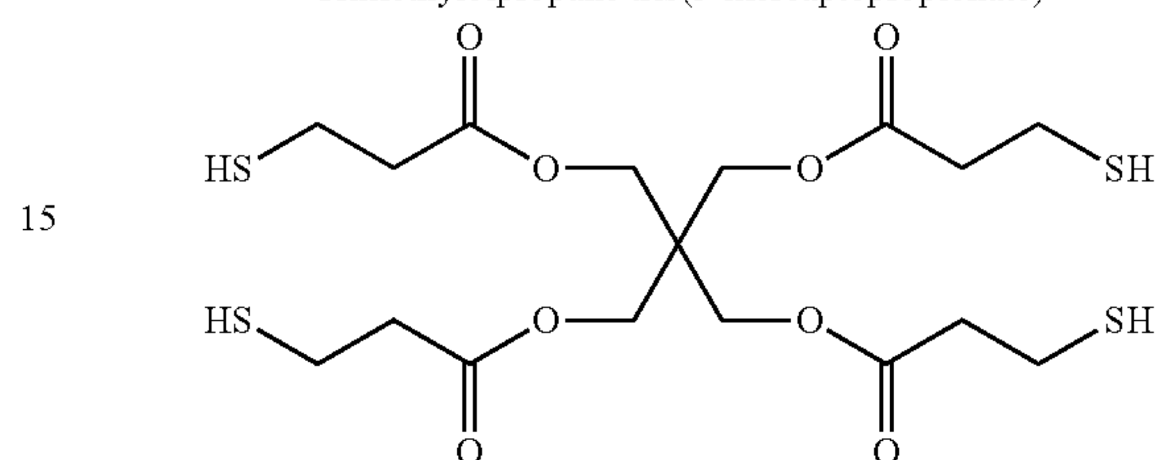
Pentaerythritol tetrakis(3-mercaptopropionate)
