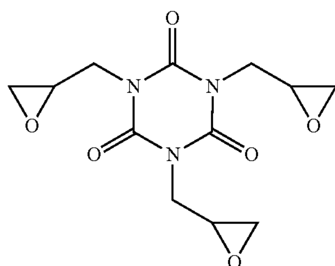
Tris(2,3-epoxypropyl) isocyanurate
