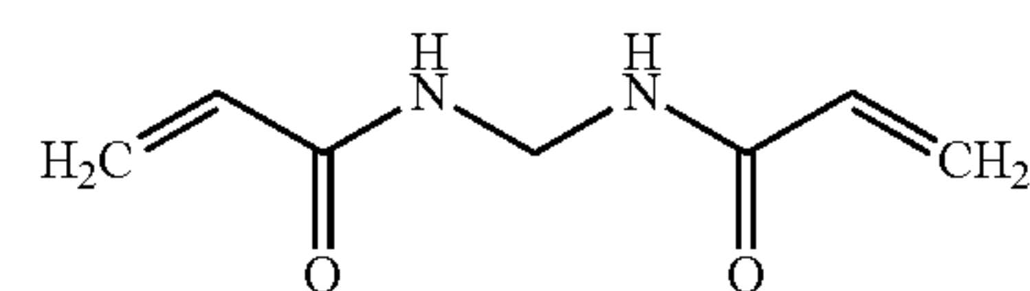
N,N'-Methylenebisacrylamide (MBAA)
