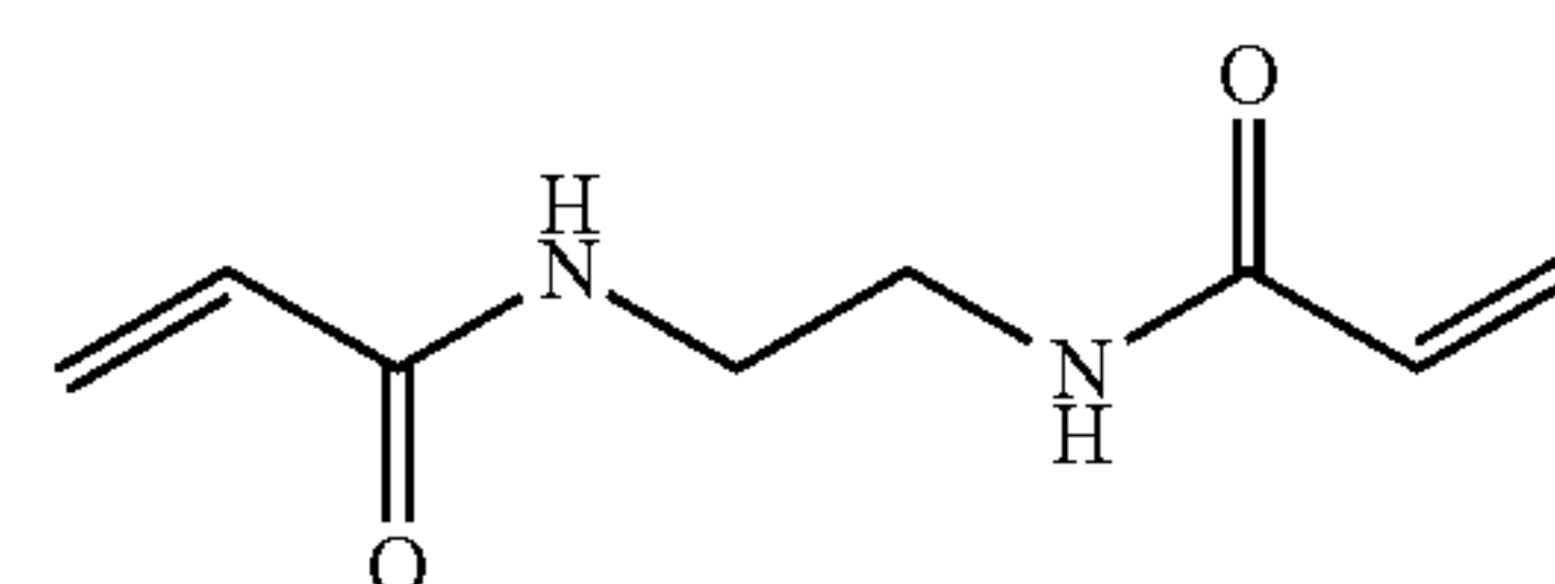
N,N'-Ethylenebisacrylamide (EBAA)
