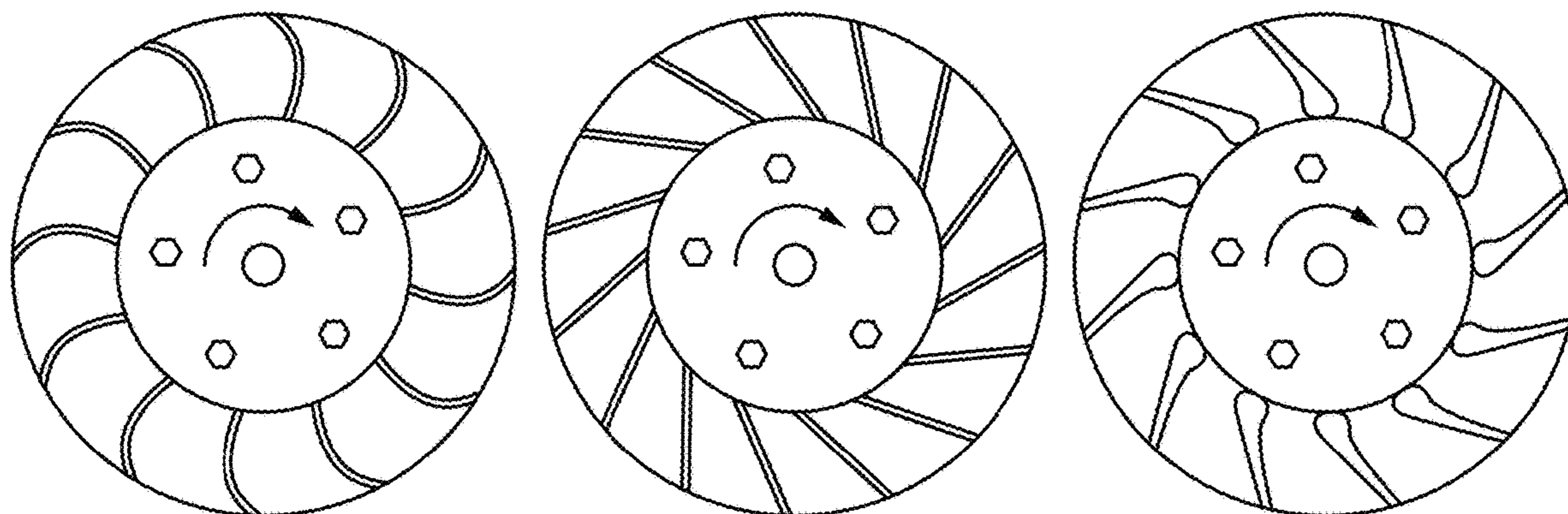
BACKWARD CURVED BLADES
