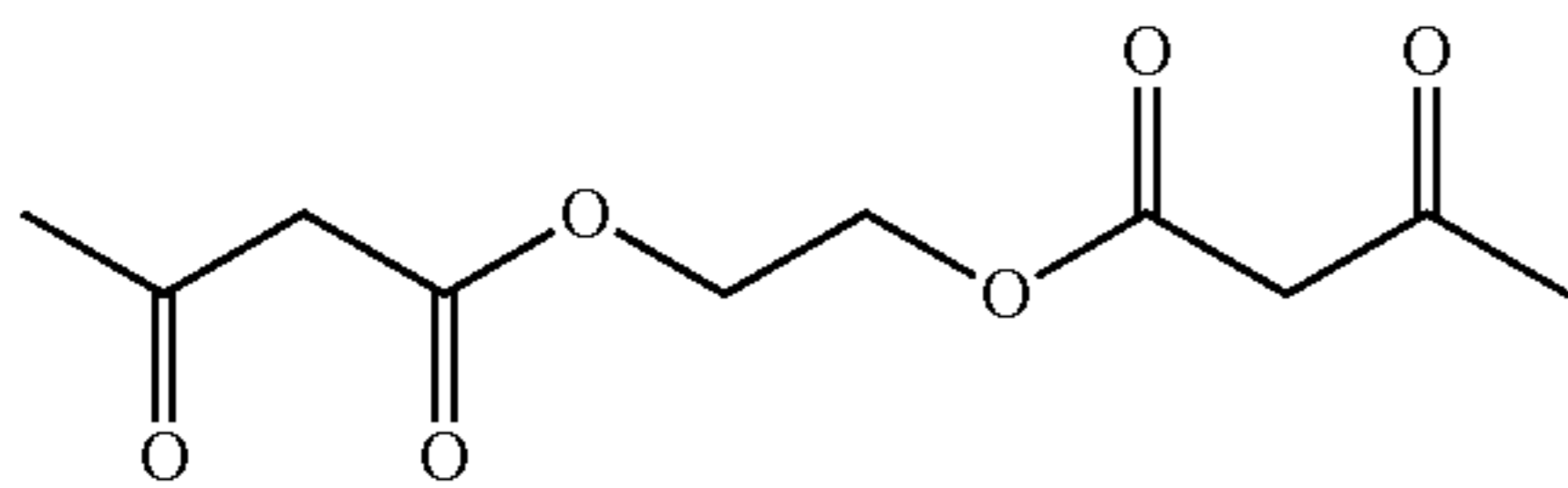
ethane-1,2-diyl bis(3-oxobutanoate)
