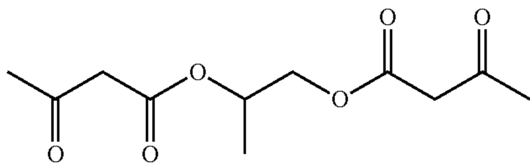
propane-1,2-diyl bis(3-oxobutanoate)
