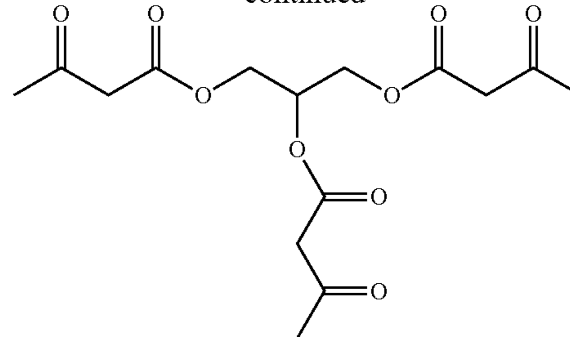
propane-1,2,3-triyl tris(3-oxobutanoate)
