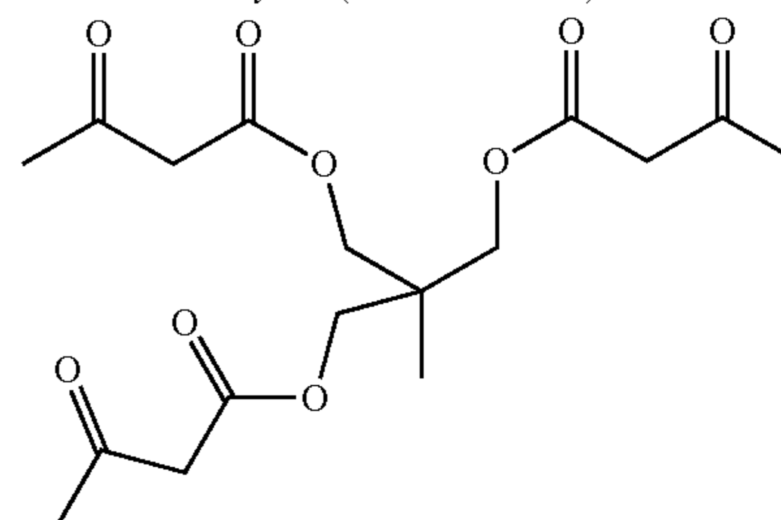
2-methyl-2-(((3-oxobutanoyl)oxy)methyl)propane-1,3-diyl bis(3-oxobutanoate)
