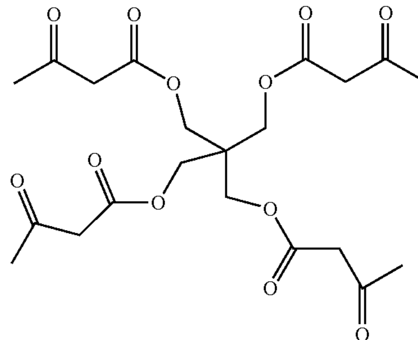
2,2-bis(((3-oxobutanoyl)oxy)methyl)-propane-1,3-diyl bis(3-oxobutanoate)
