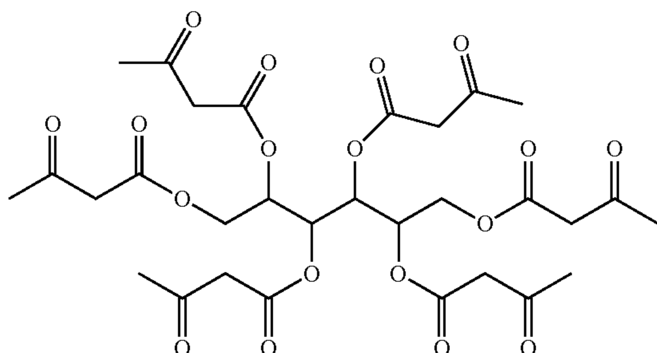
hexane-1,2,3,4,5,6-hexayl hexakis(3-oxobutanoate)
