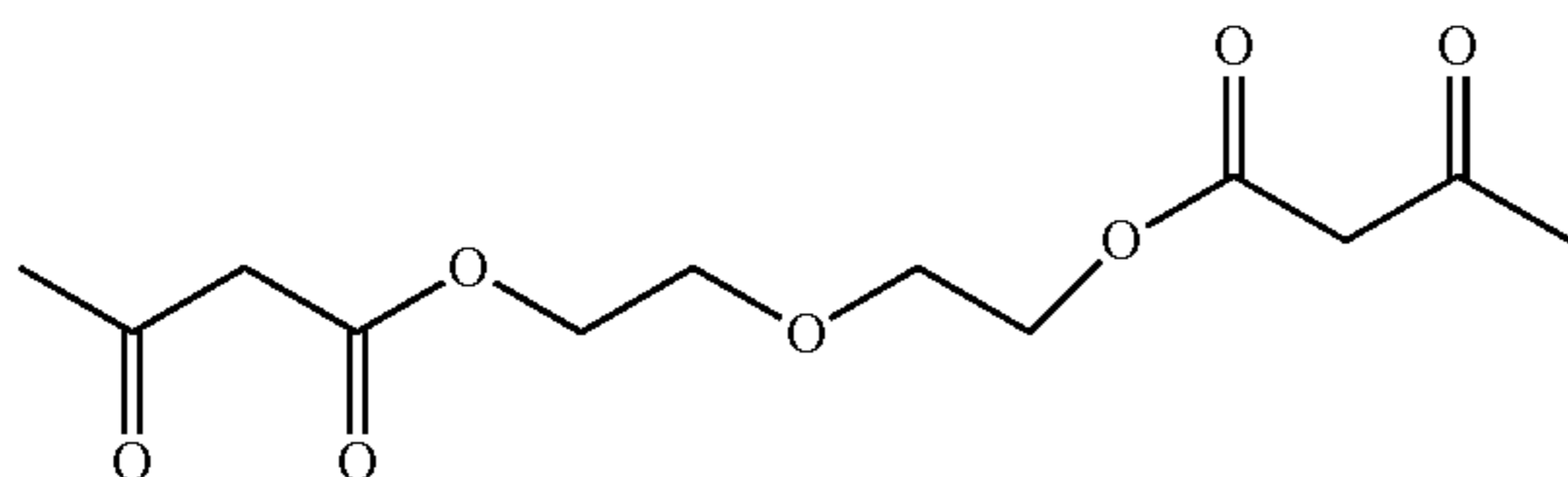
oxybis(ethane-2-1-diyl) bis(3-oxobutanoate)
