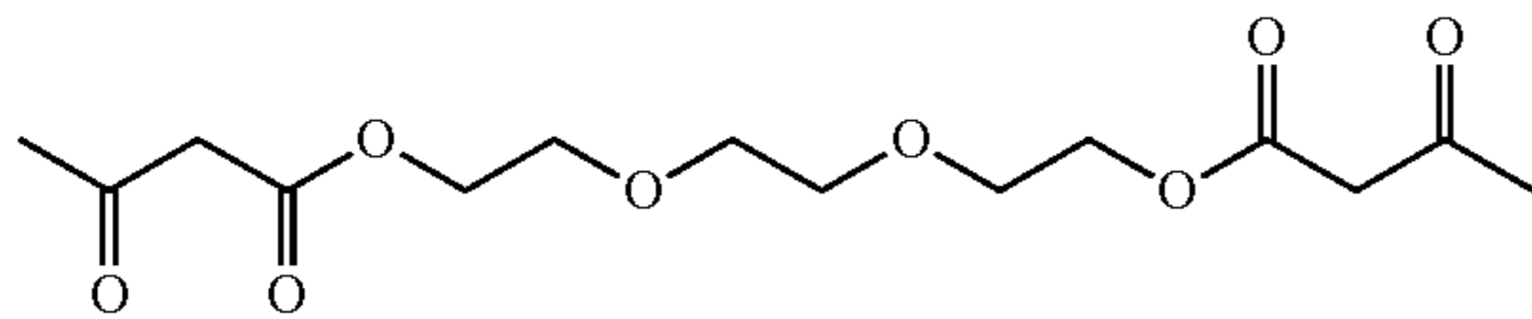
(ethane-1,2-diylbis(oxy))bis(ethane-2,1-diyl) bis(3-oxobutanoate)
