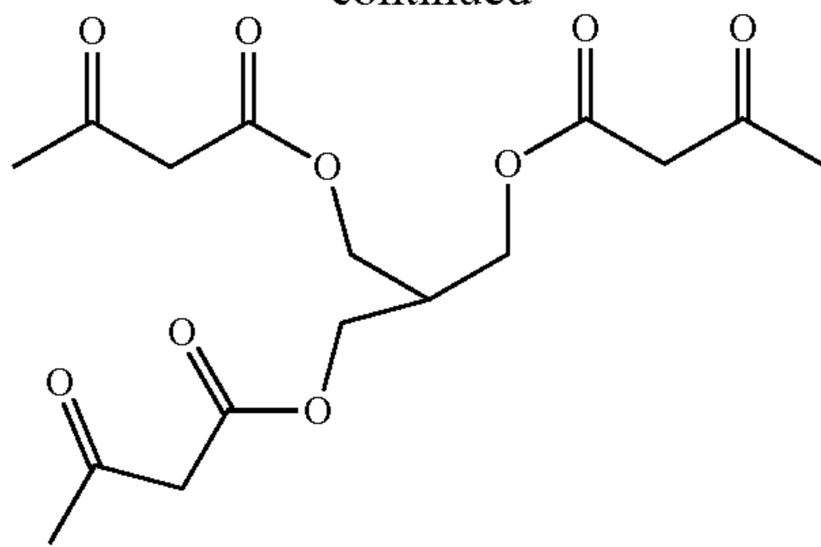
2-(((3-oxobutanoyl)oxy)methyl)propane-1,3-diyl bis(3-oxobutanoate)
