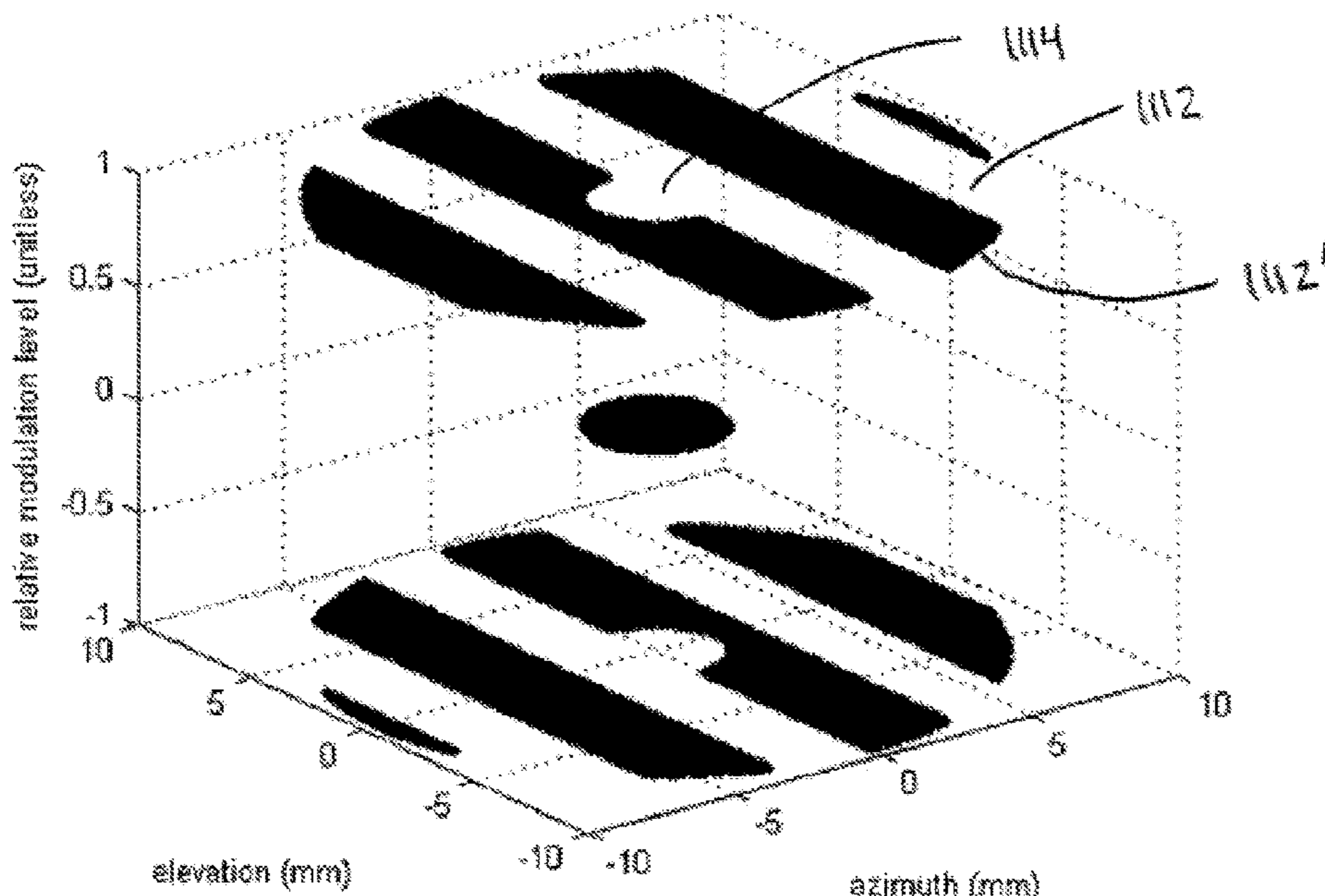
Modulation of Lateral Split (0.55 mm) 7 MHz Transducer
