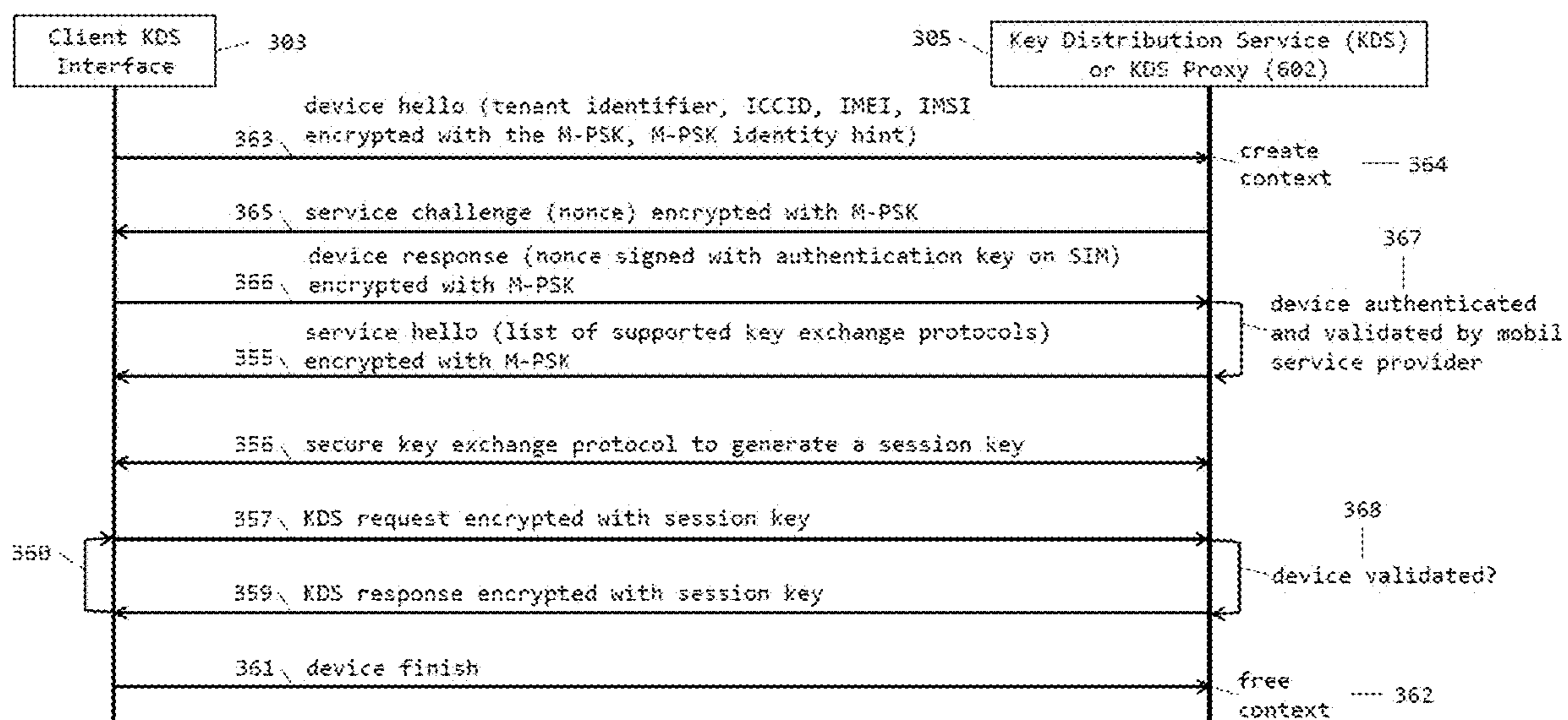
MOBILE DEVICE AUTHENTICATION HANDSHAKE WITH M-PSK
