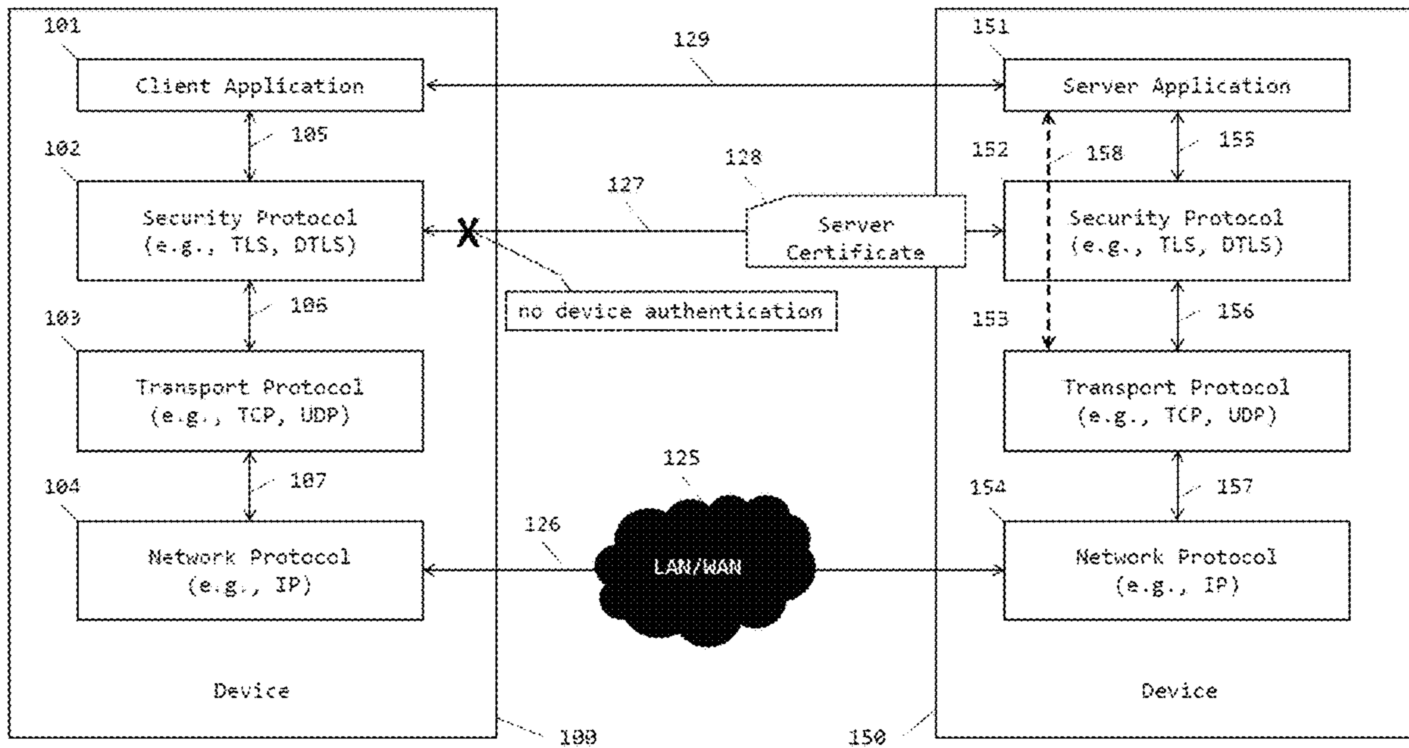
TLS CONNECTION WITH SERVER CERTIFICATE VERIFICATION
