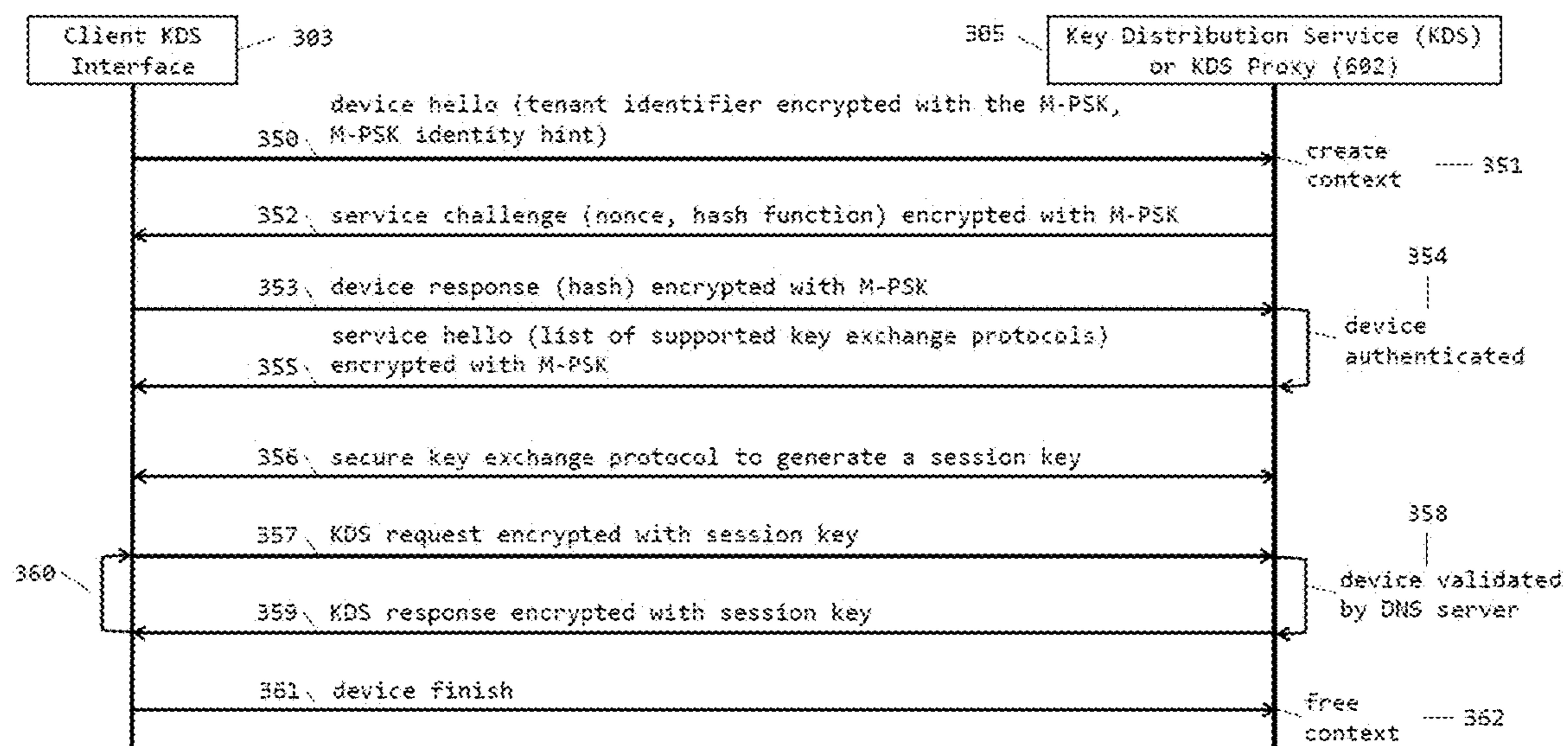
DEVICE AUTHENTICATION HANDSHAKE WITH M-PSK
