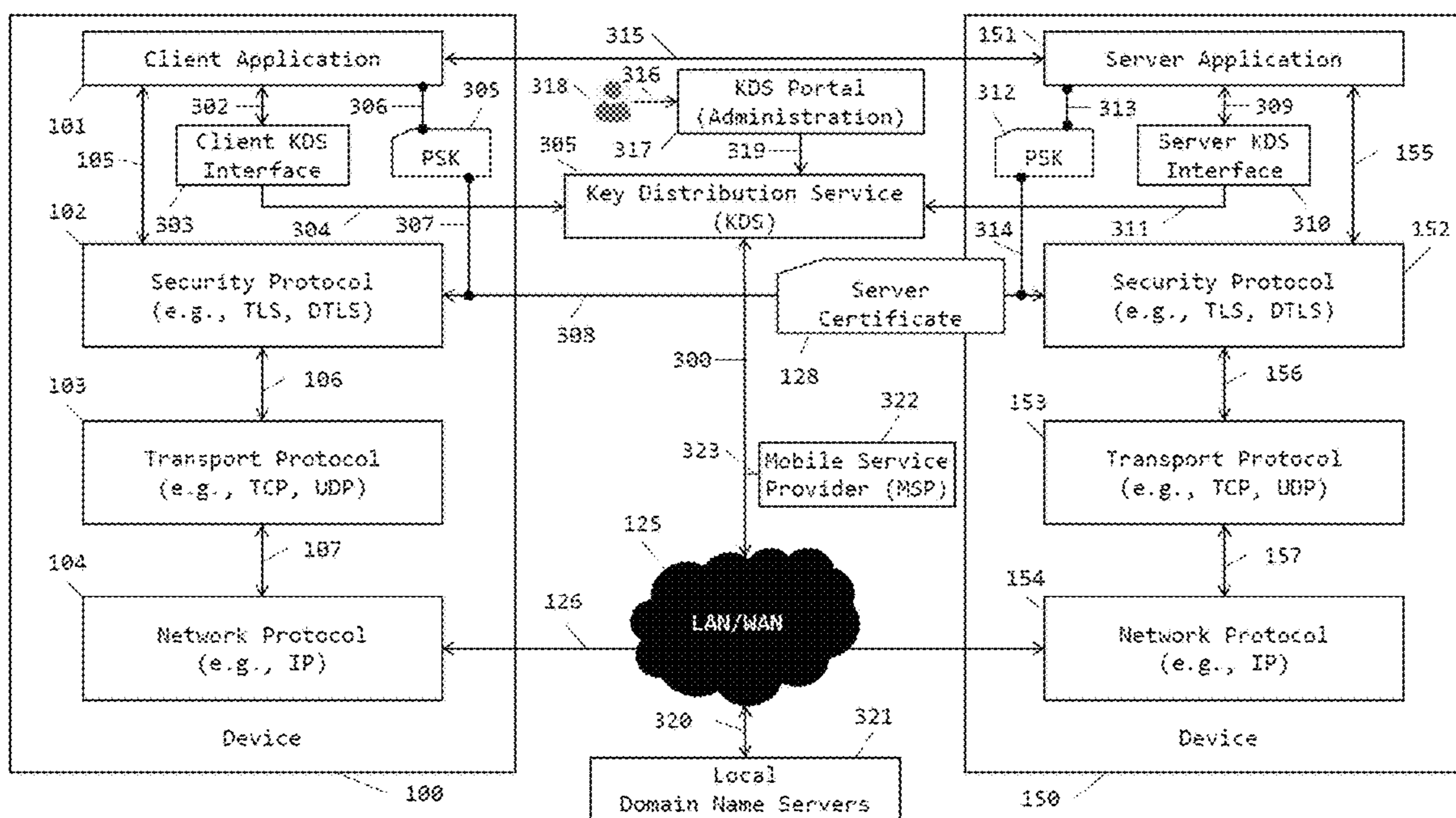
FIG. 3A TLS CONNECTION WITH PSK BASED CLIENT AUTHENTICATION
