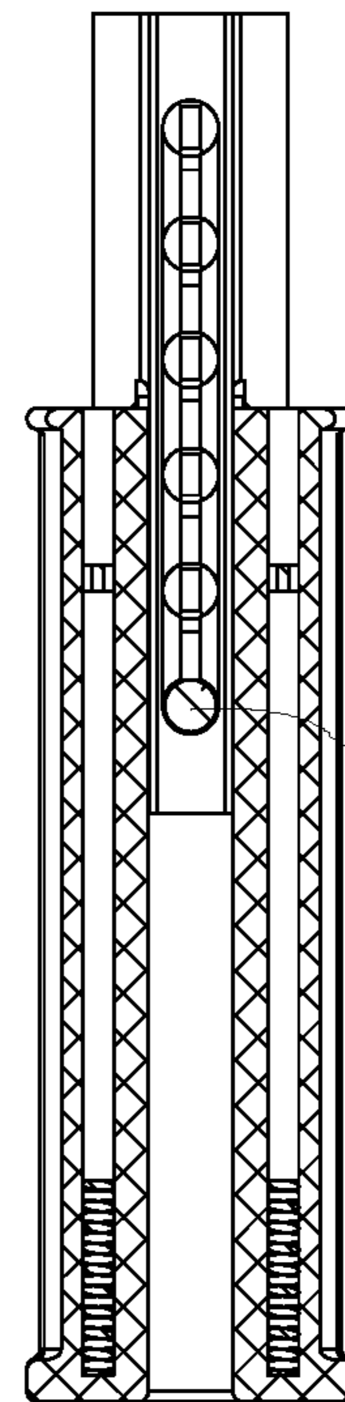
SECTION K-K
