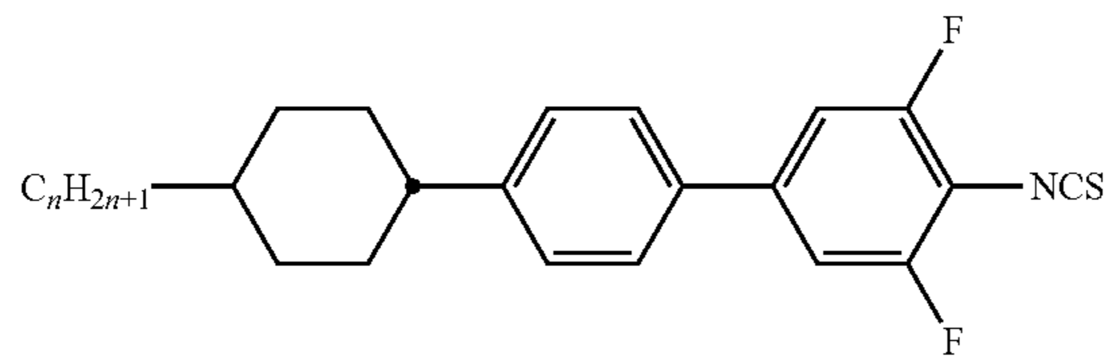
CPU-n-S
