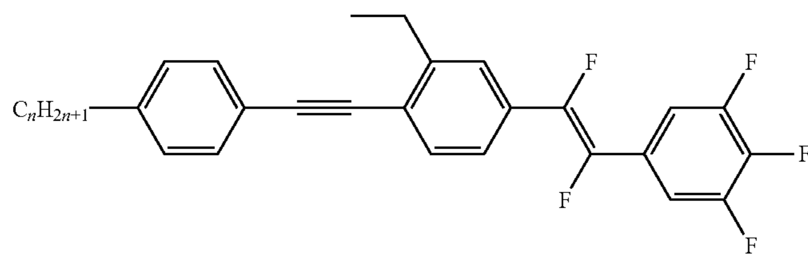
PTPI(2)WU-n-F
