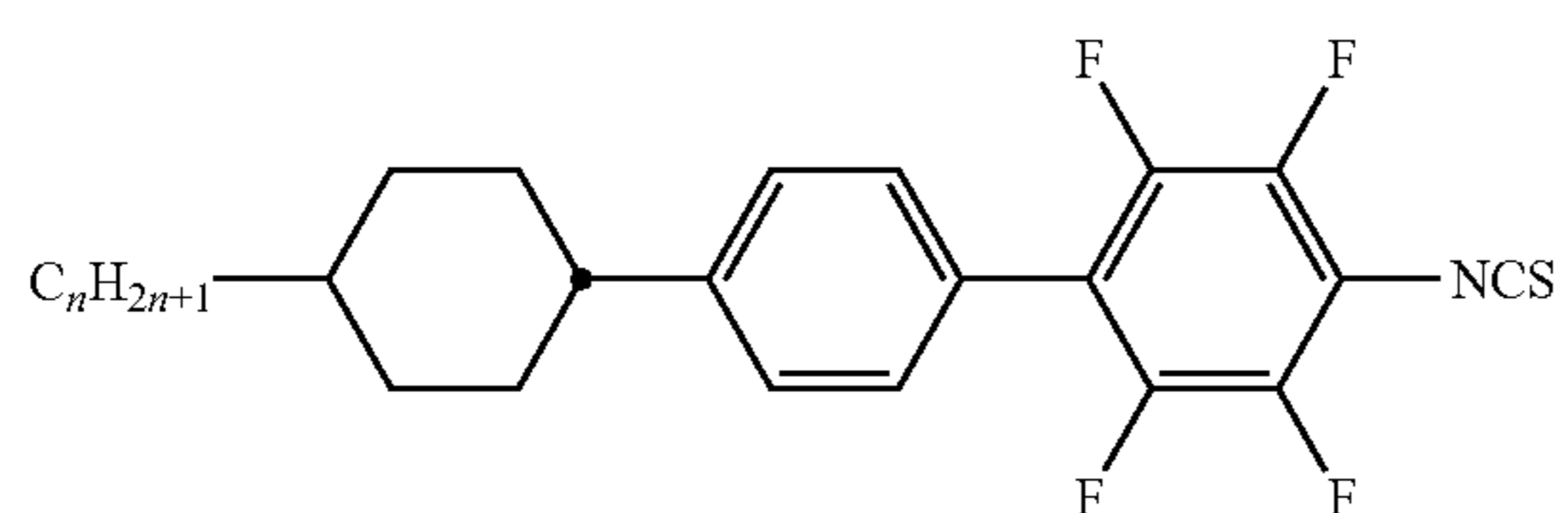
CPU(F,F)-n-S
