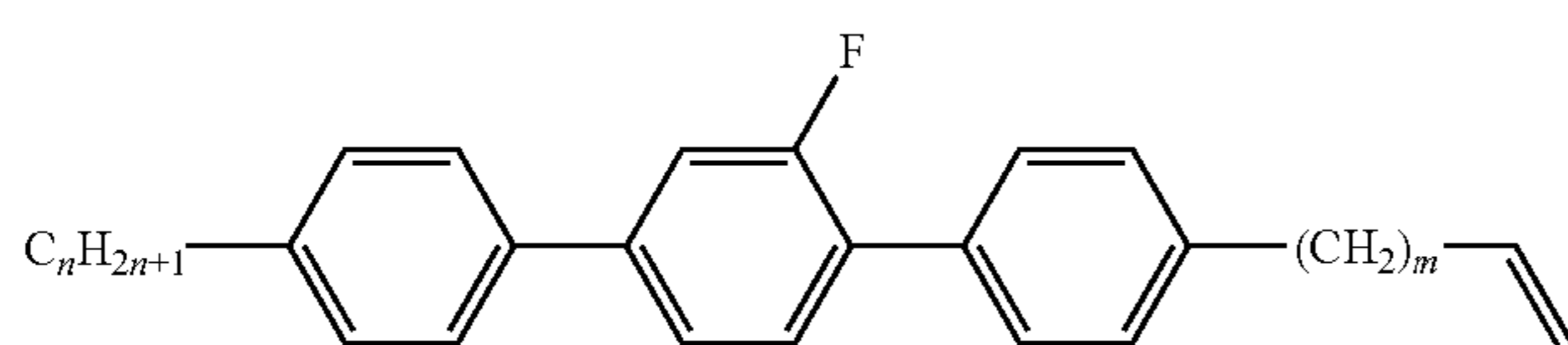
PGP-n-mVI
