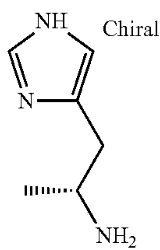
histamine R(-)-alpha-methyl-dihydrochloride(
