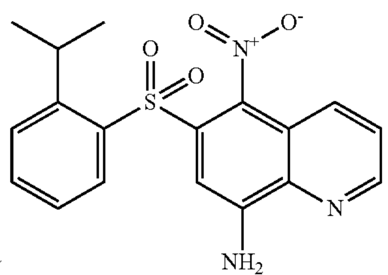
PD160170 (
