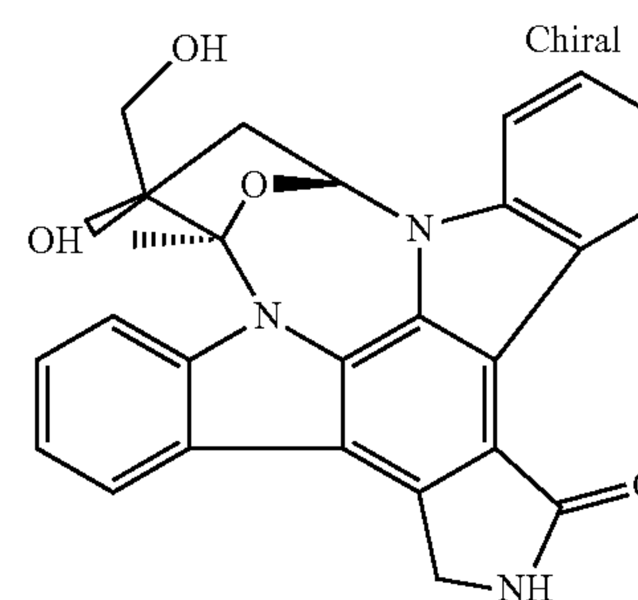
Lestaurtinib (CEP701, ),
