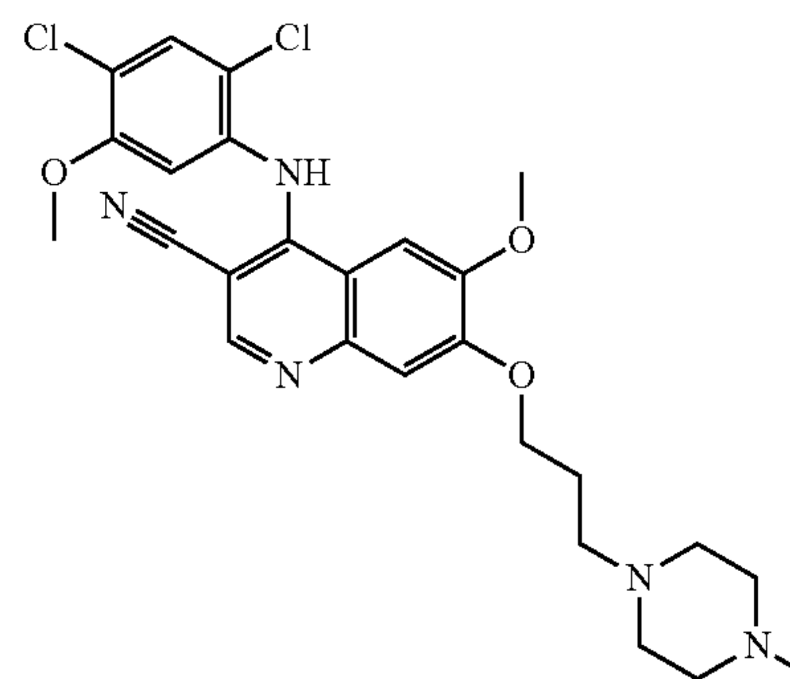
Bosutinib (SKI 606, ),
