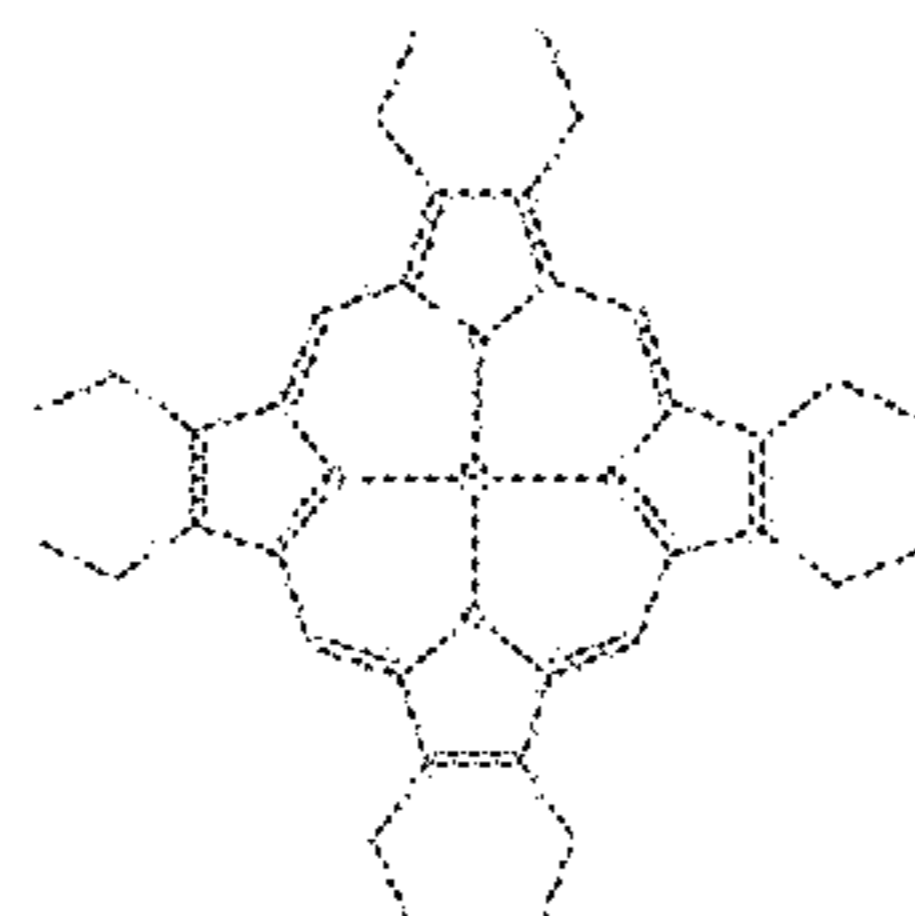
Compound 14
