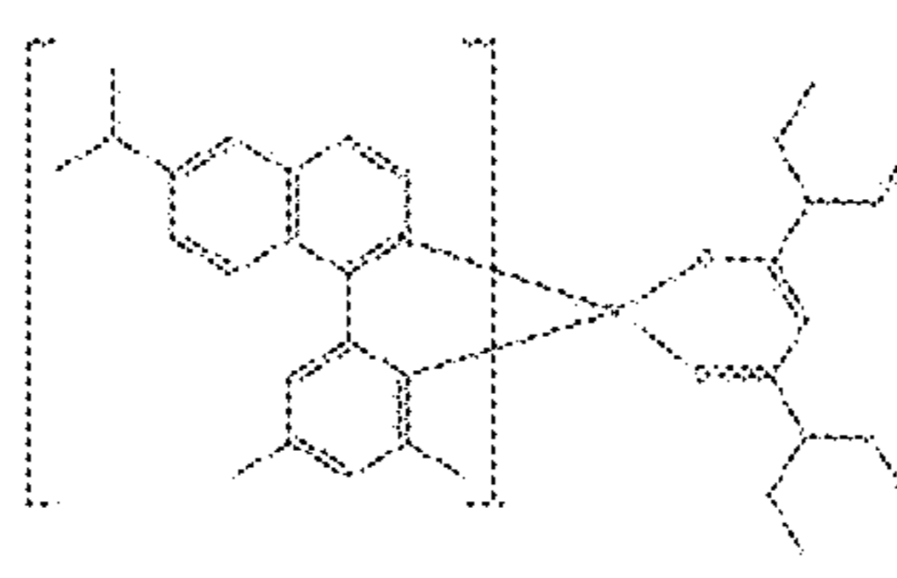
Compound 11
