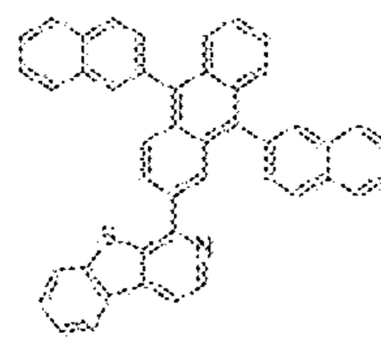
Compound 6
