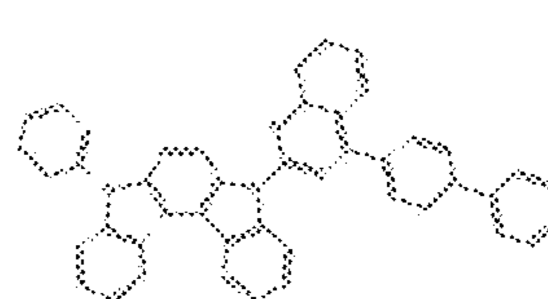
Compound 8
