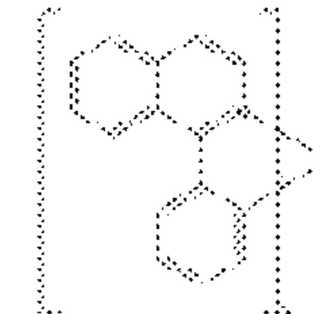
Compound 9
