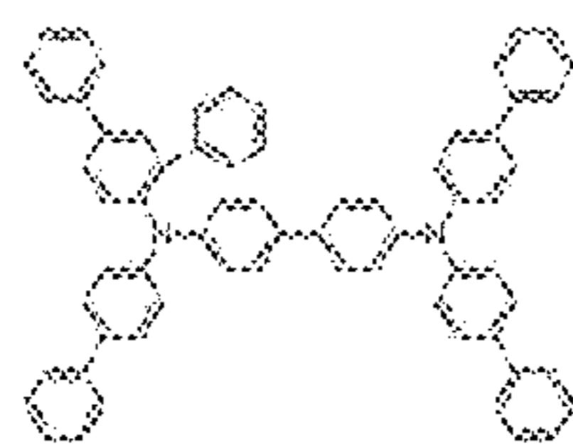
Compound 2
