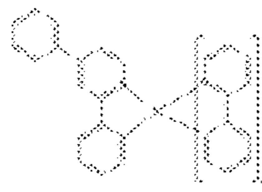
Compound 5
