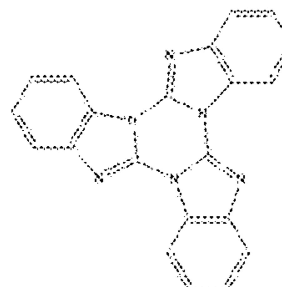
Compound 15
