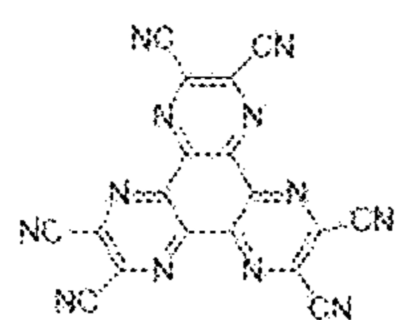
Compound 1
