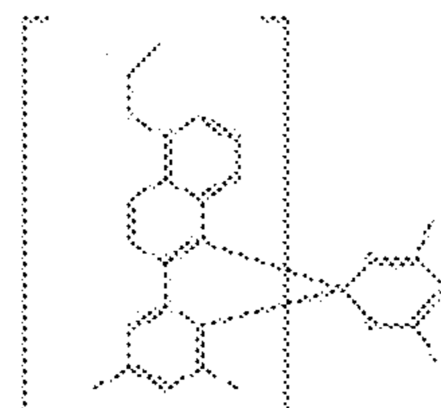
Compound 10
