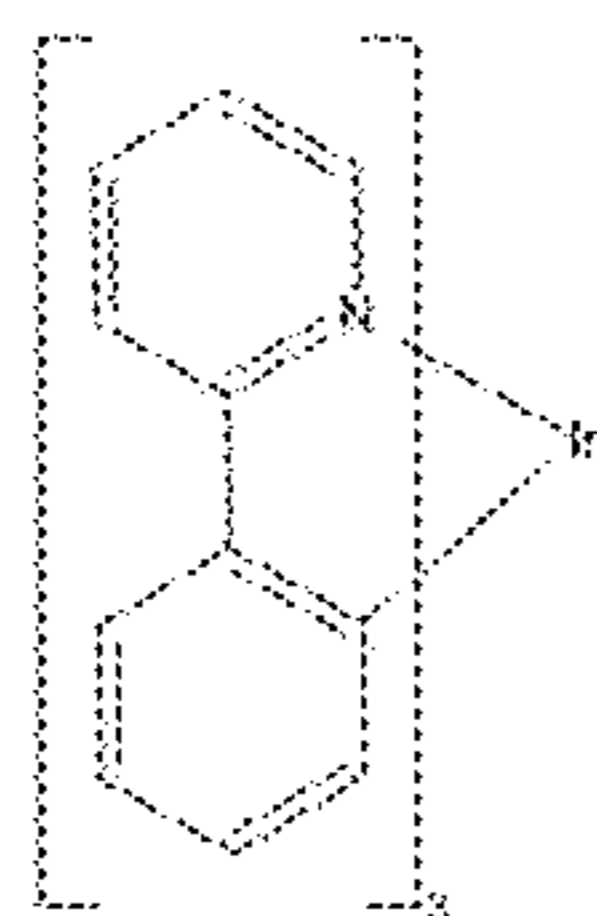
Compound 13
