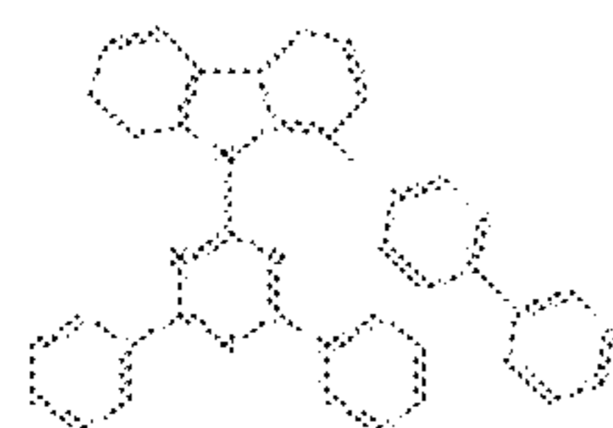
Compound 4
