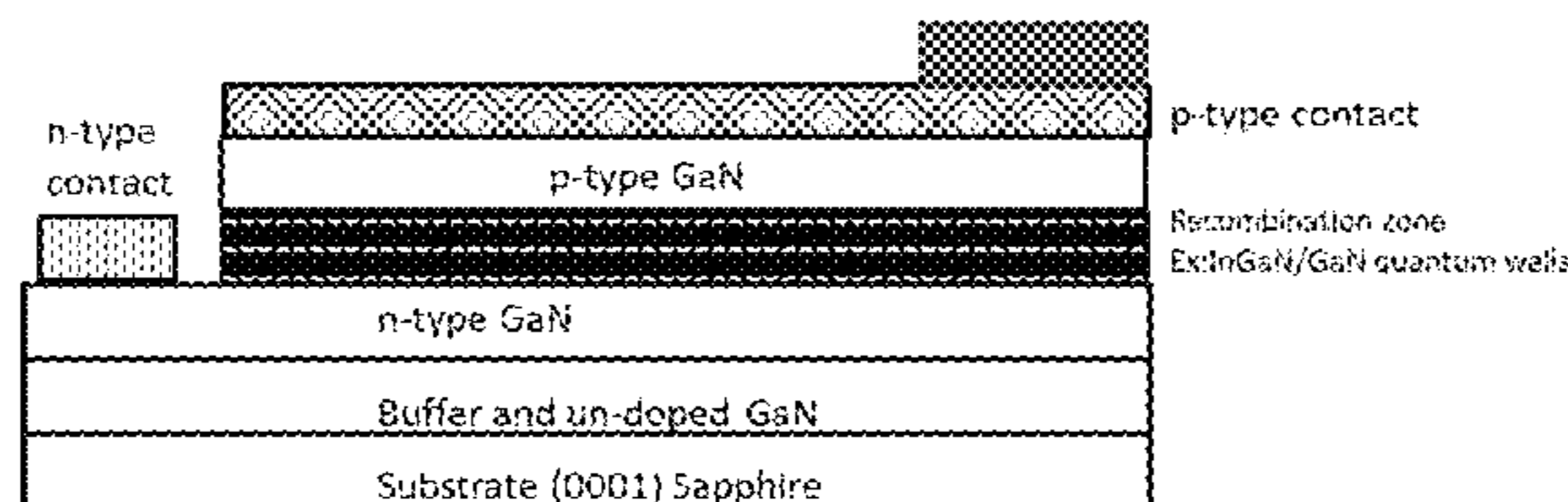
Example Inorganic LED design
