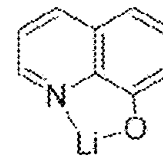
Compound 7
