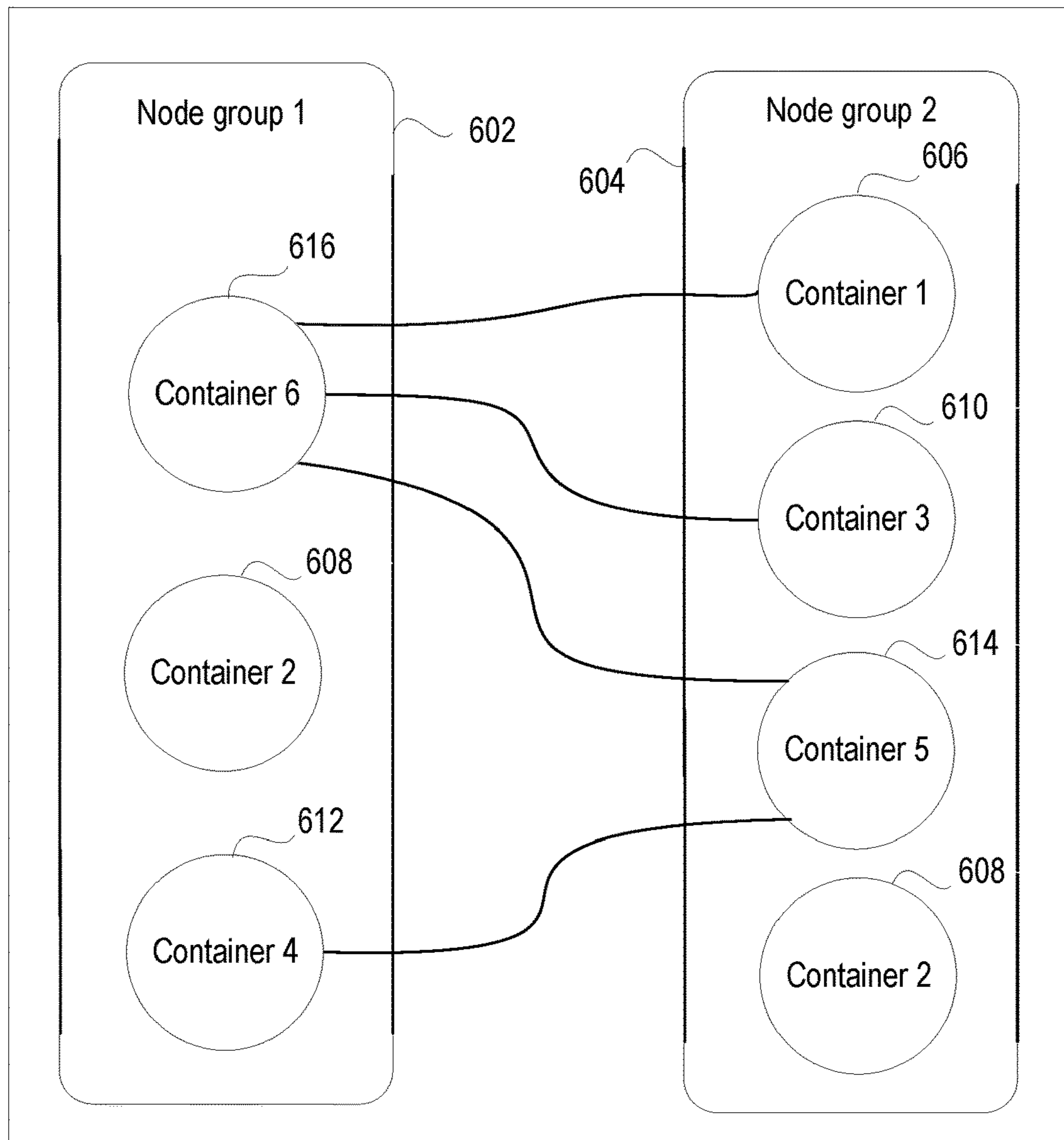
Allowed grouping
