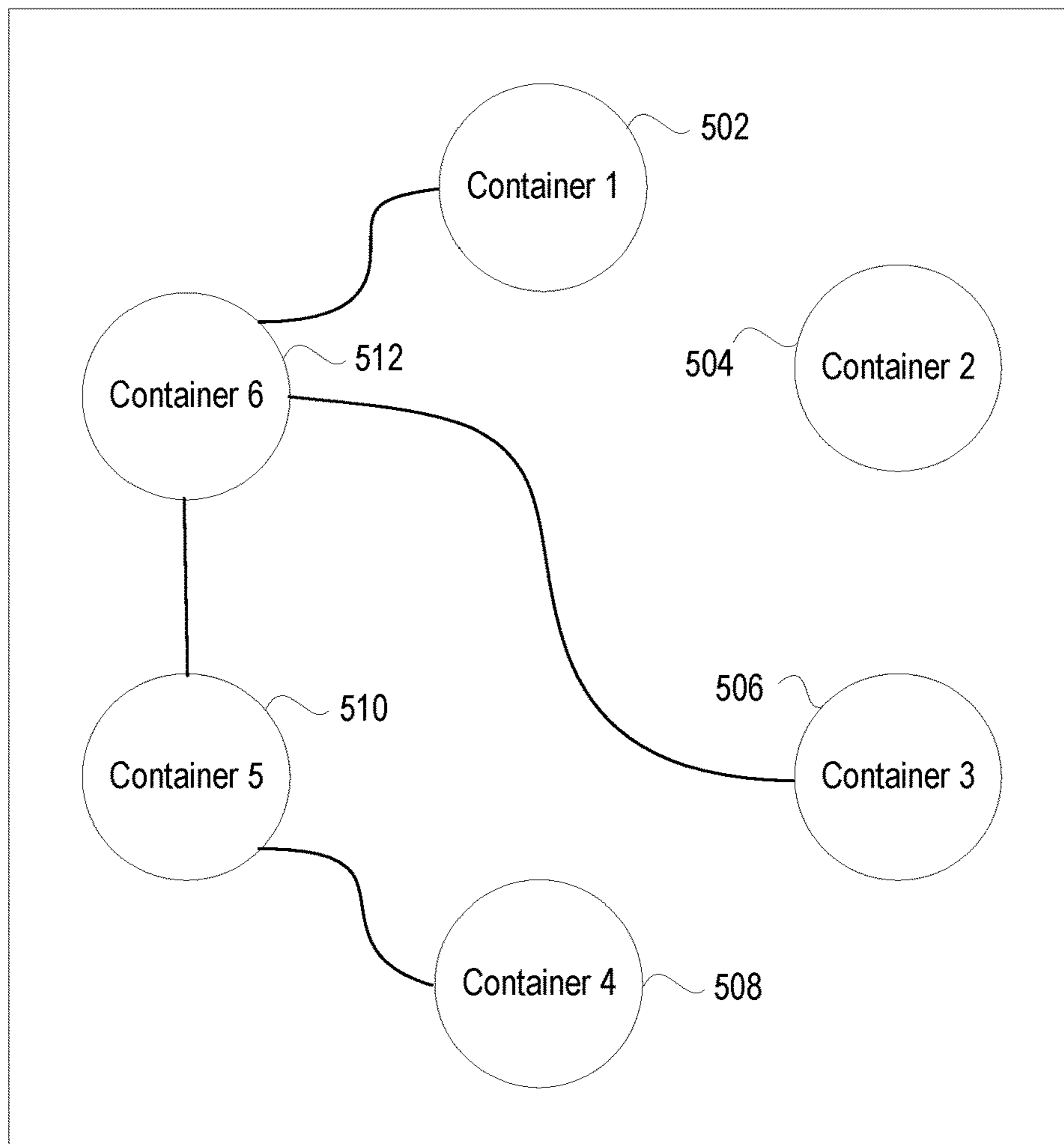
Forbidden arrangements
