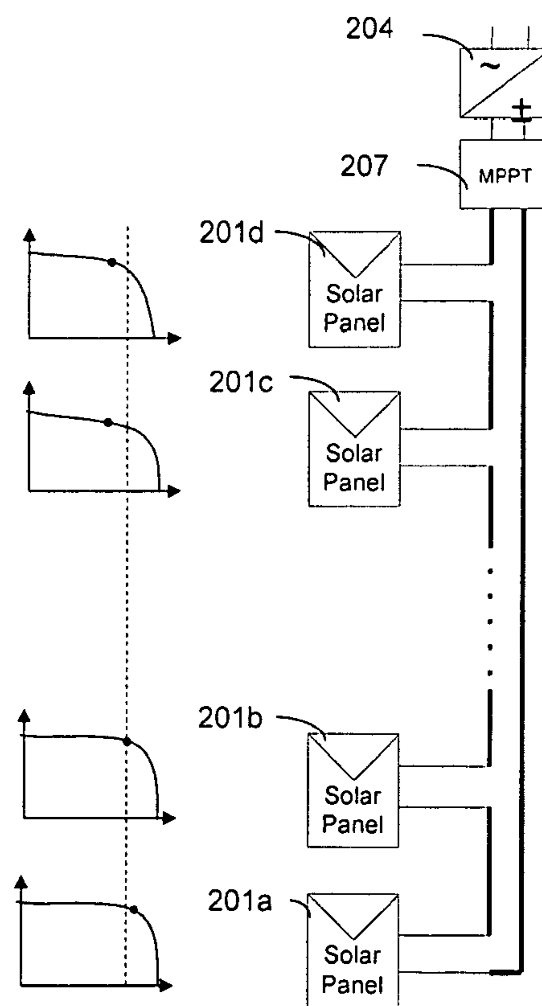
Figure 2 - Prior Art
