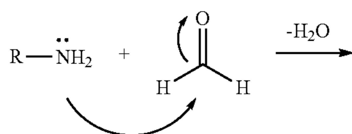
Mannich reaction
