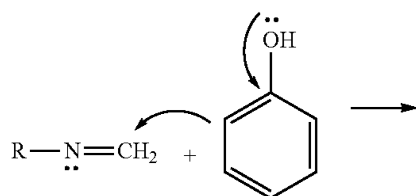
Electrophilic substitution
