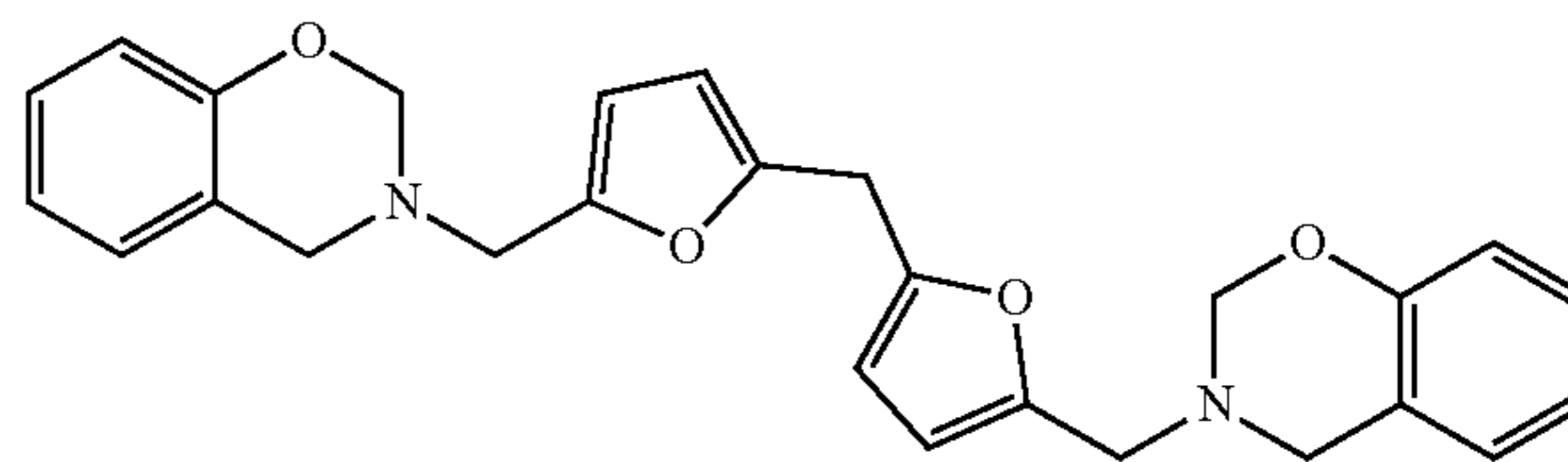
Bz-DFDA-phenol (1)
