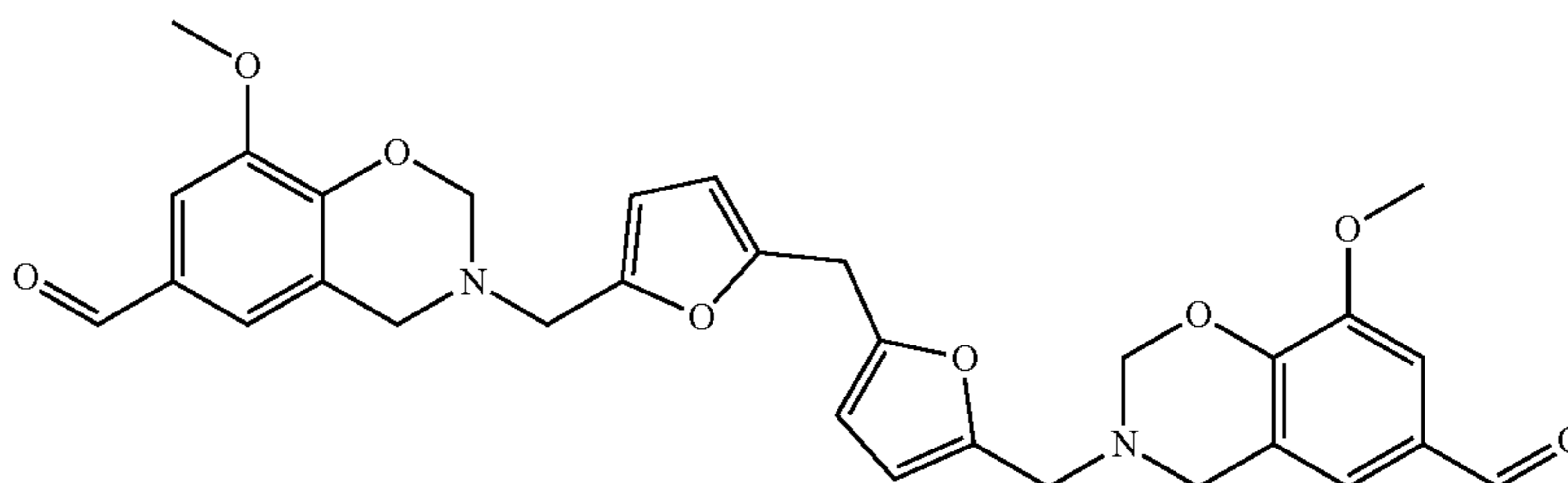
Bz-DFDA-vanillin (2)
