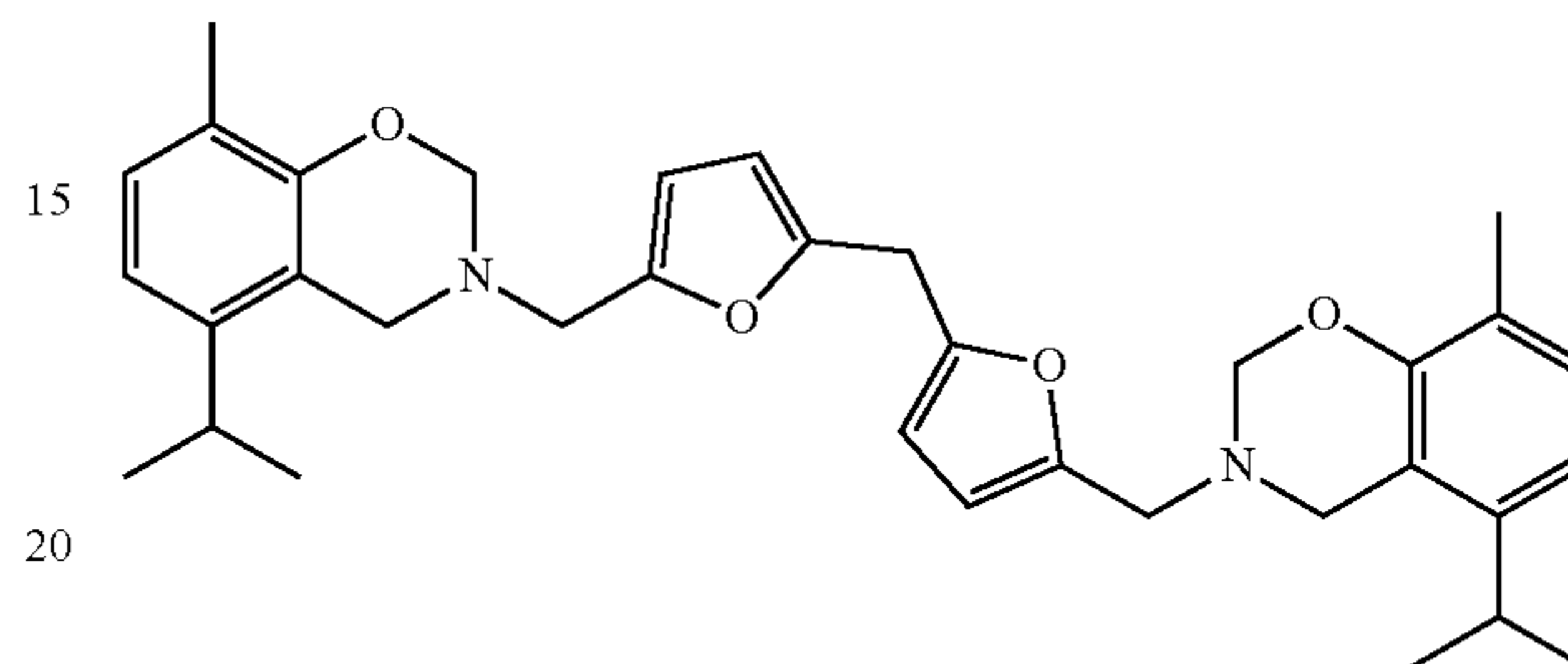
Bz-DFDA-carvacrol (4)
