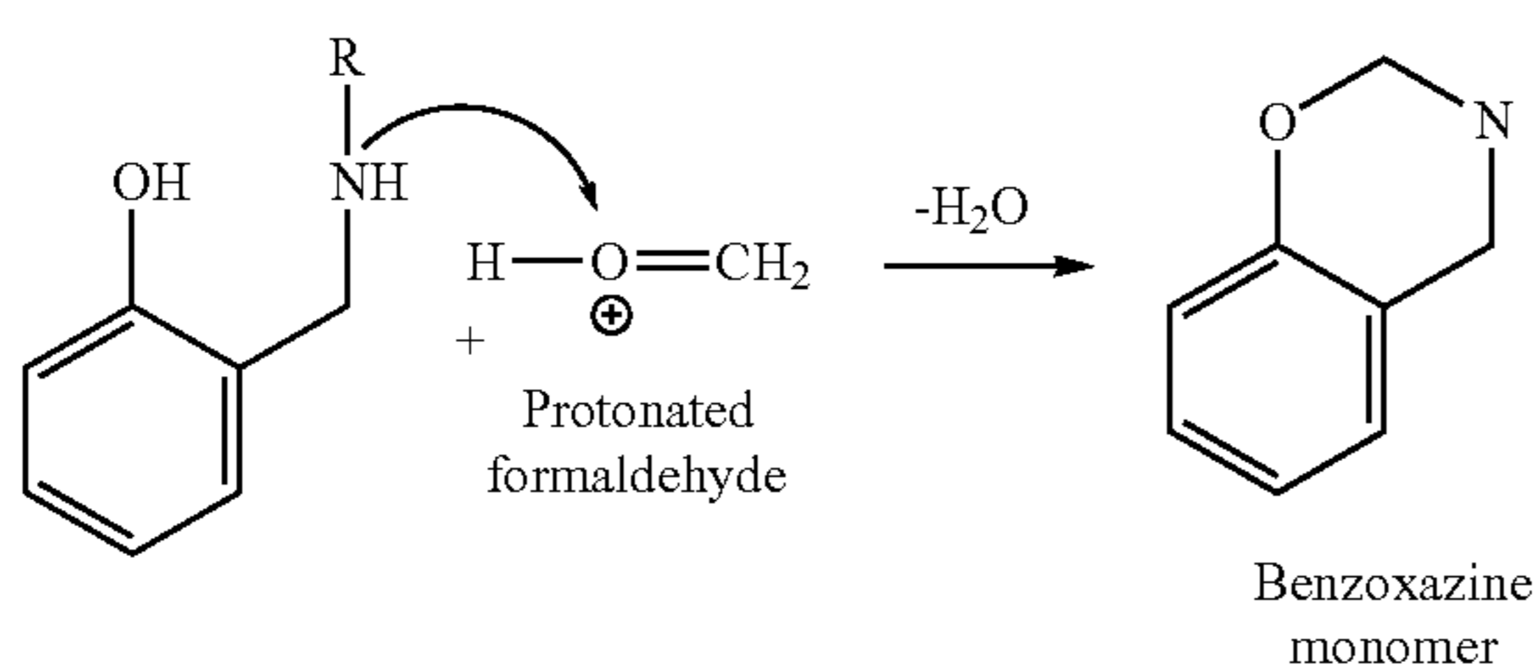
Electrophilic substitution
